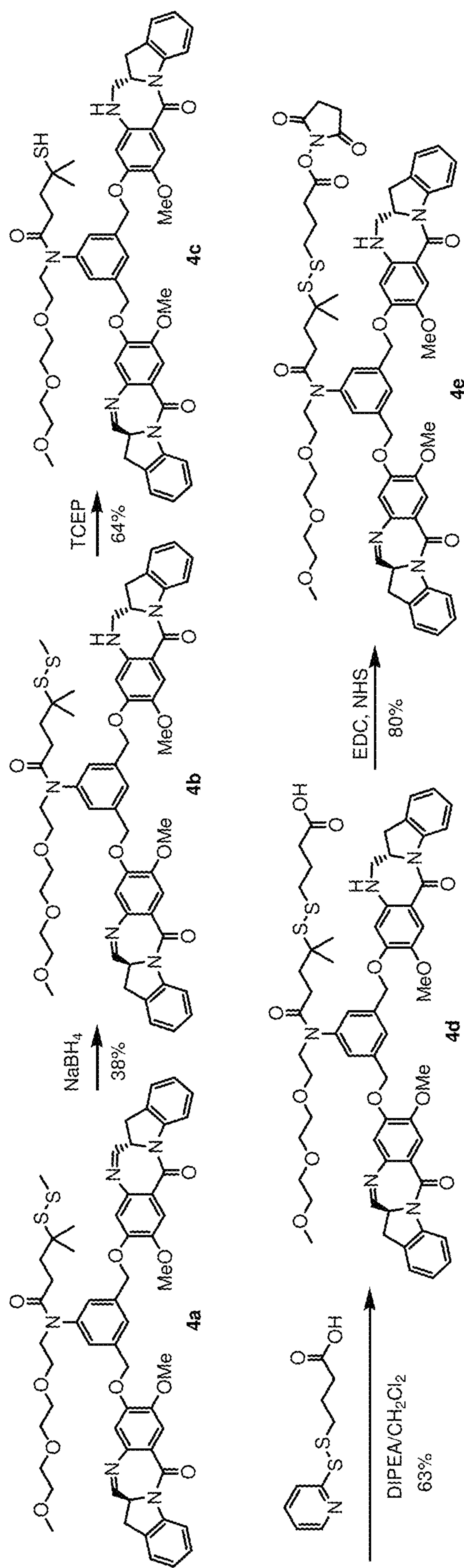
FIG. 4. Synthetic Scheme of Dimers 4b-e
