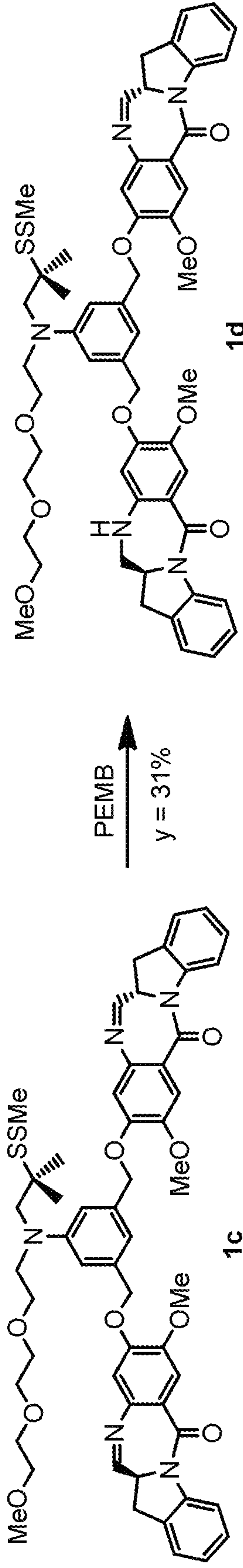
FIG. 39. Synthetic Scheme of Compound 1d with 5-ethyl-2-methylpyridine borane (PEMB)
