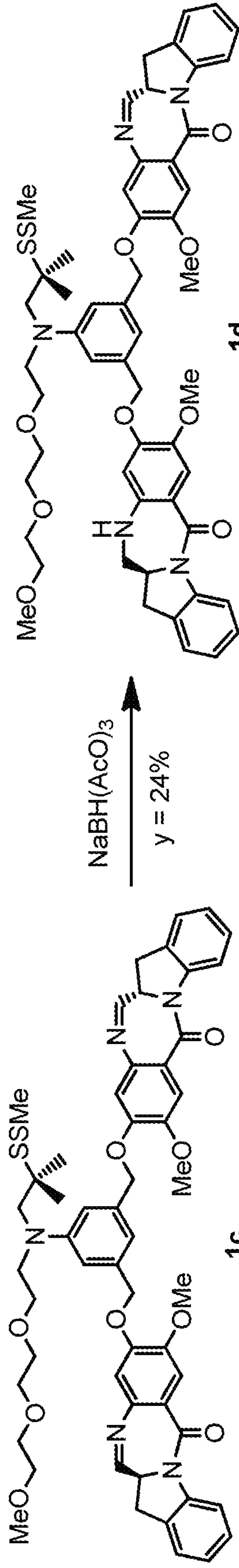
FIG. 40. Synthetic Scheme of Compound 1d with sodium triacetoxymethylborohydride (STAB)
