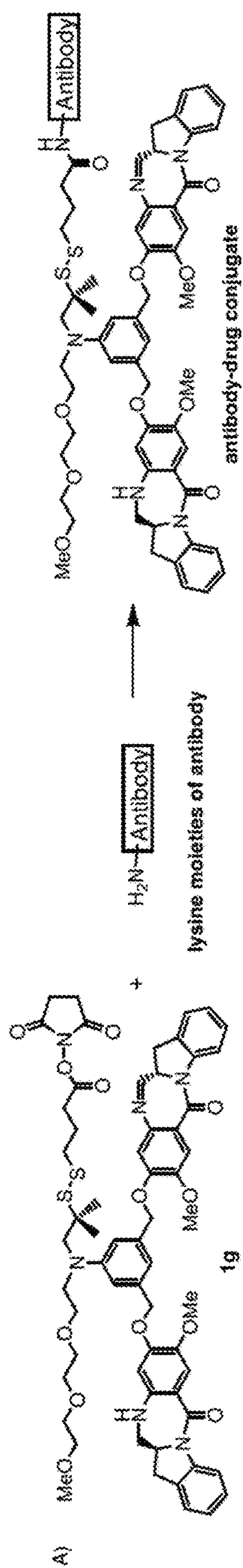
FIG. 22B. One Step Conjugation Scheme of Compound 10 to a lysine moiety of an Antibody
