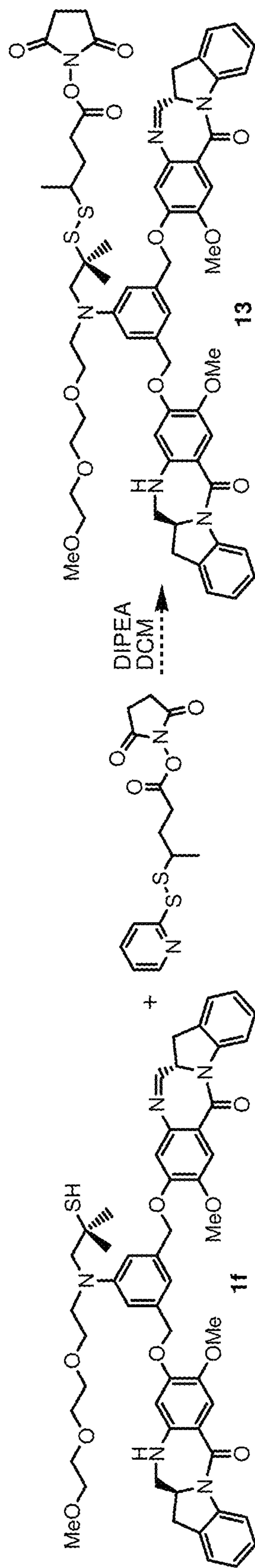
FIG. 16. Synthetic Scheme of the One-step SPP Linkable Dimer 13
