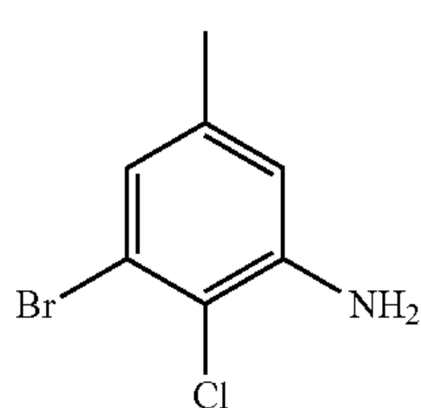
3-bromo-2-chloro-5-methylaniline
