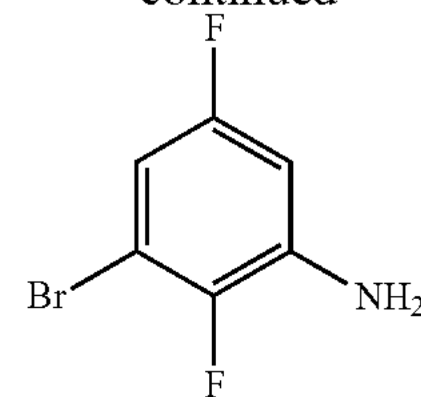
3-bromo-2,5-difluoroaniline
