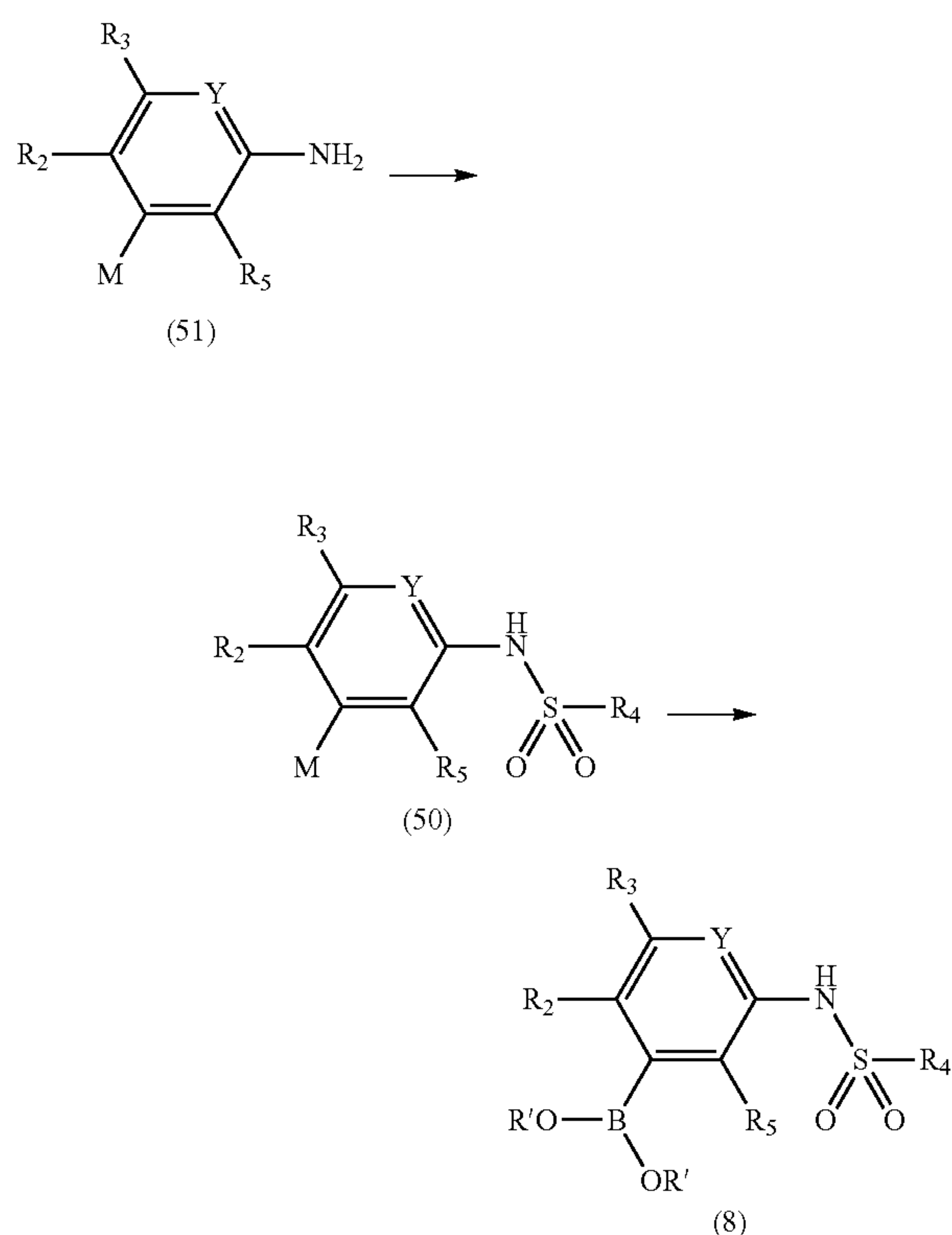
Reaction Scheme VII
