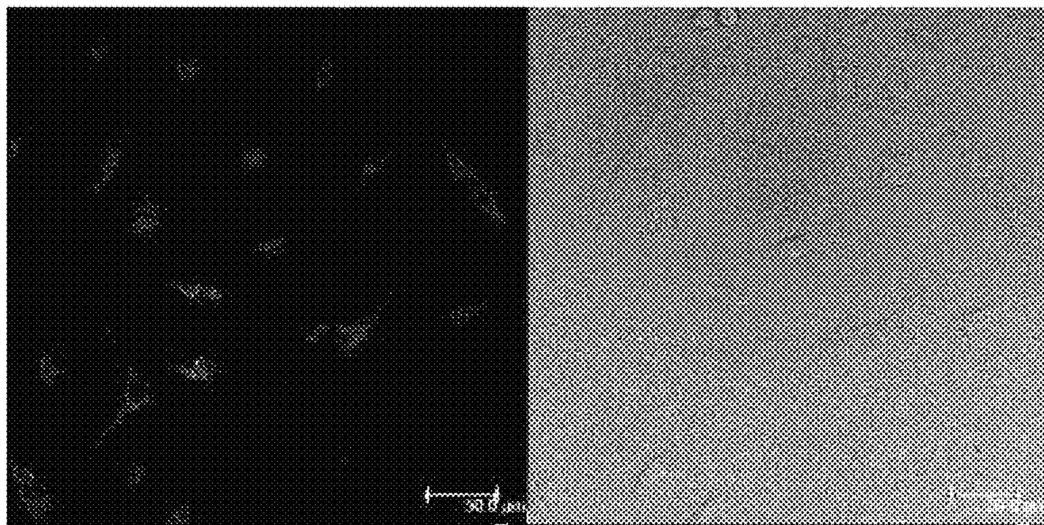
(b)Ac-LM-HMRG+ALLN1 μM
