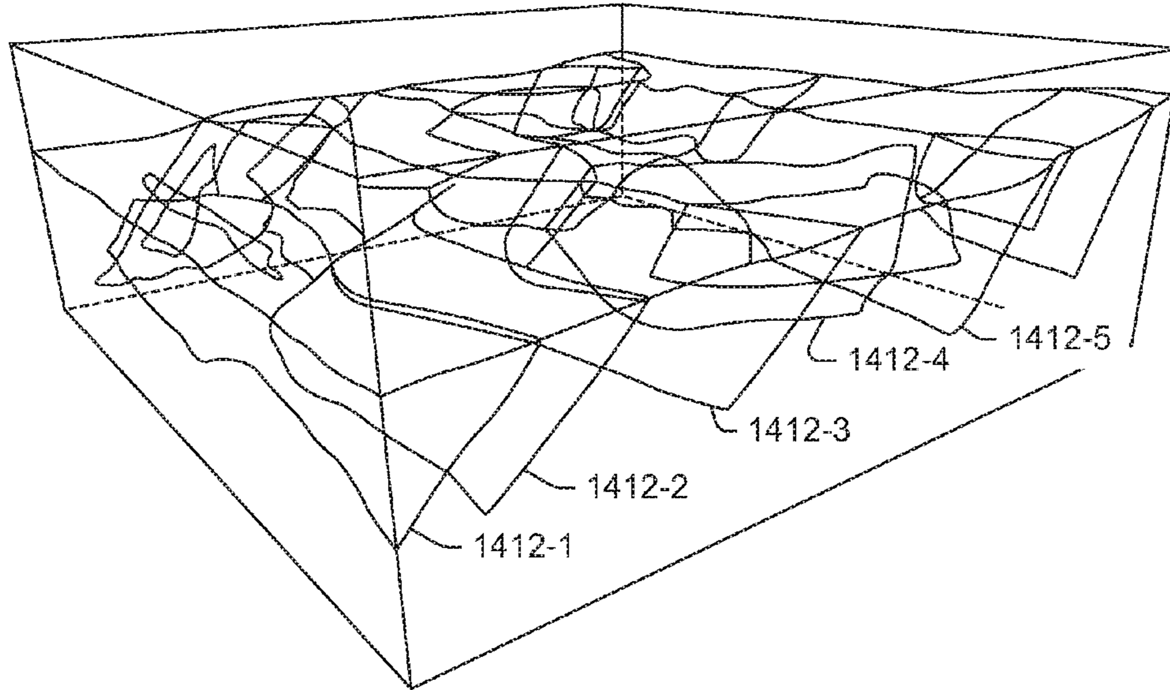
Active Faults 1410
