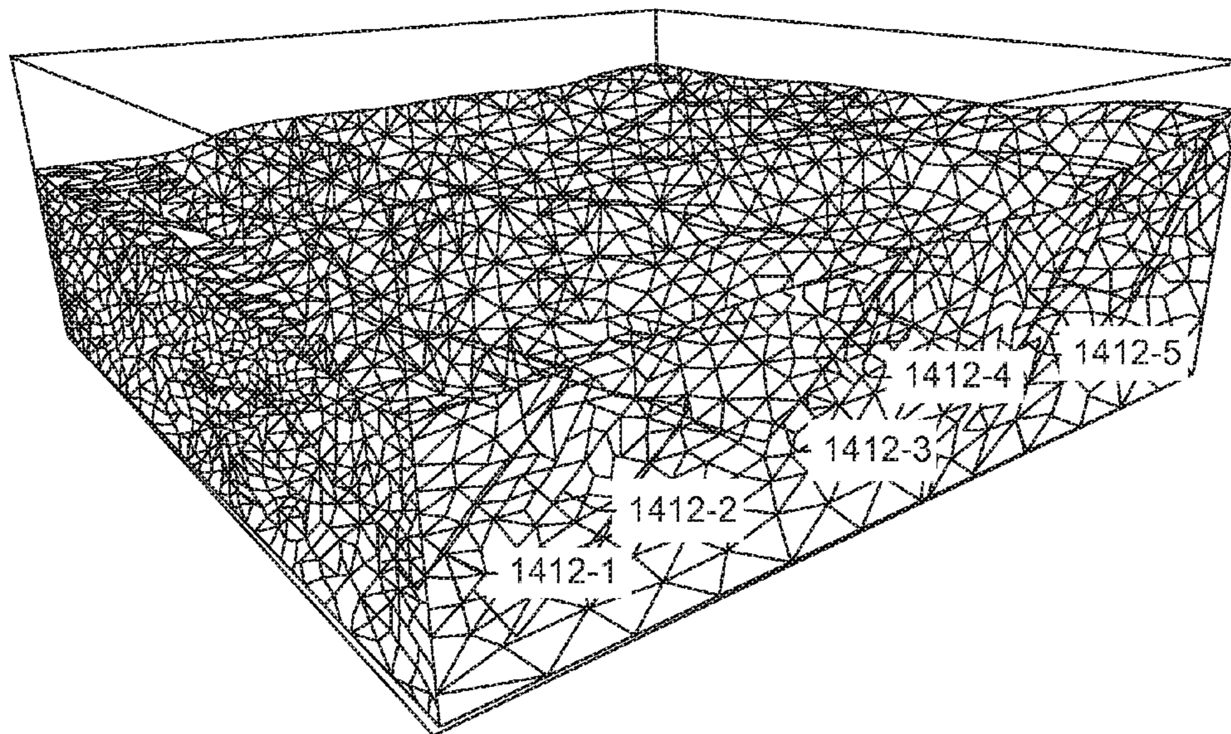
Re-Meshed 1430
