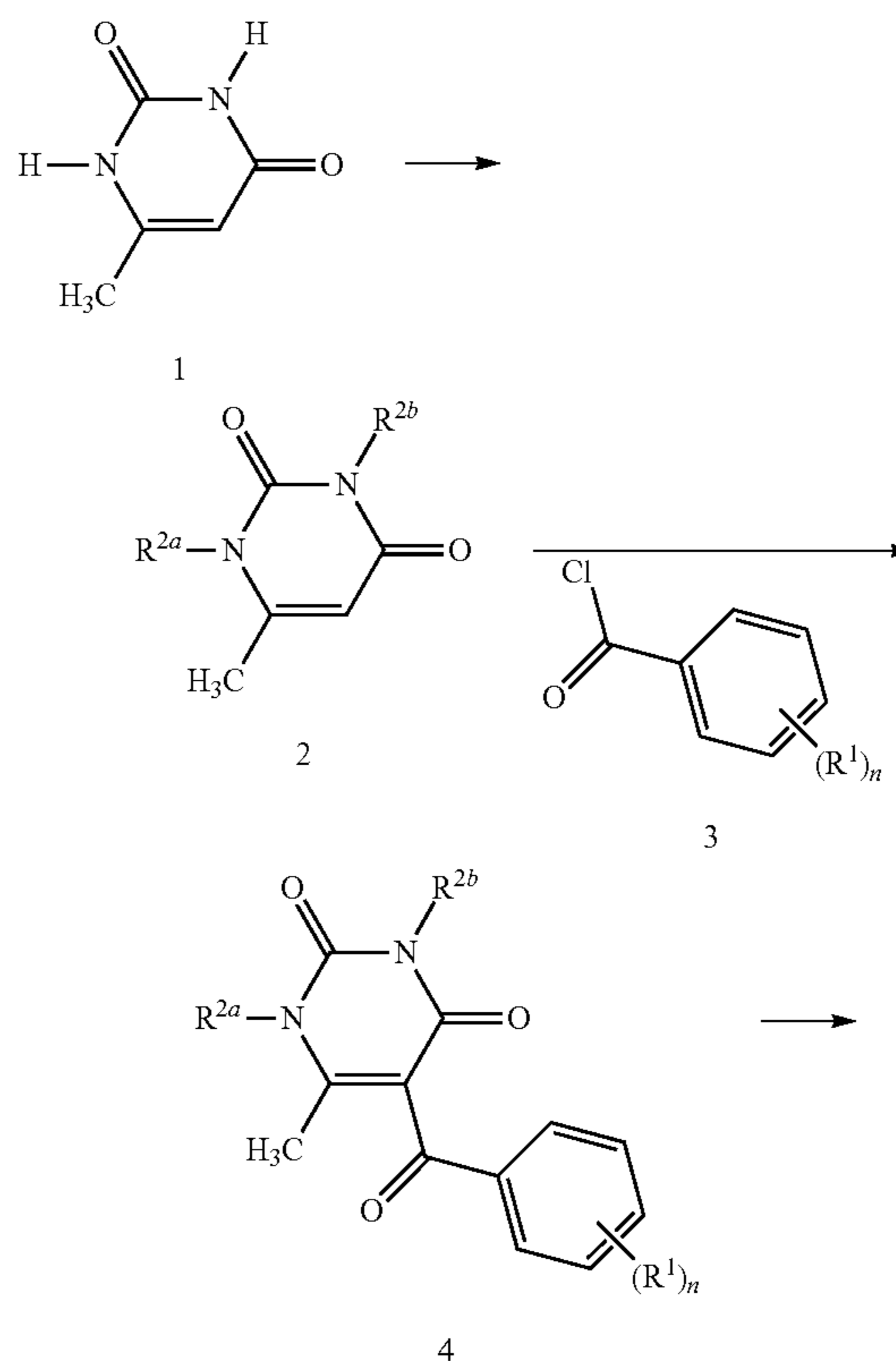
General Reaction Scheme (I)
