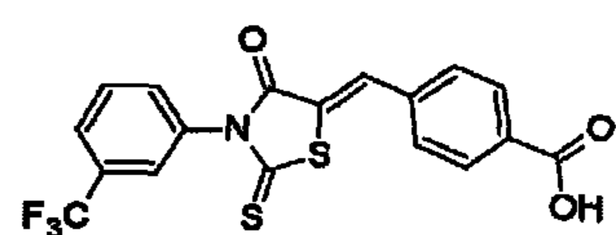
CFTR inh -172
