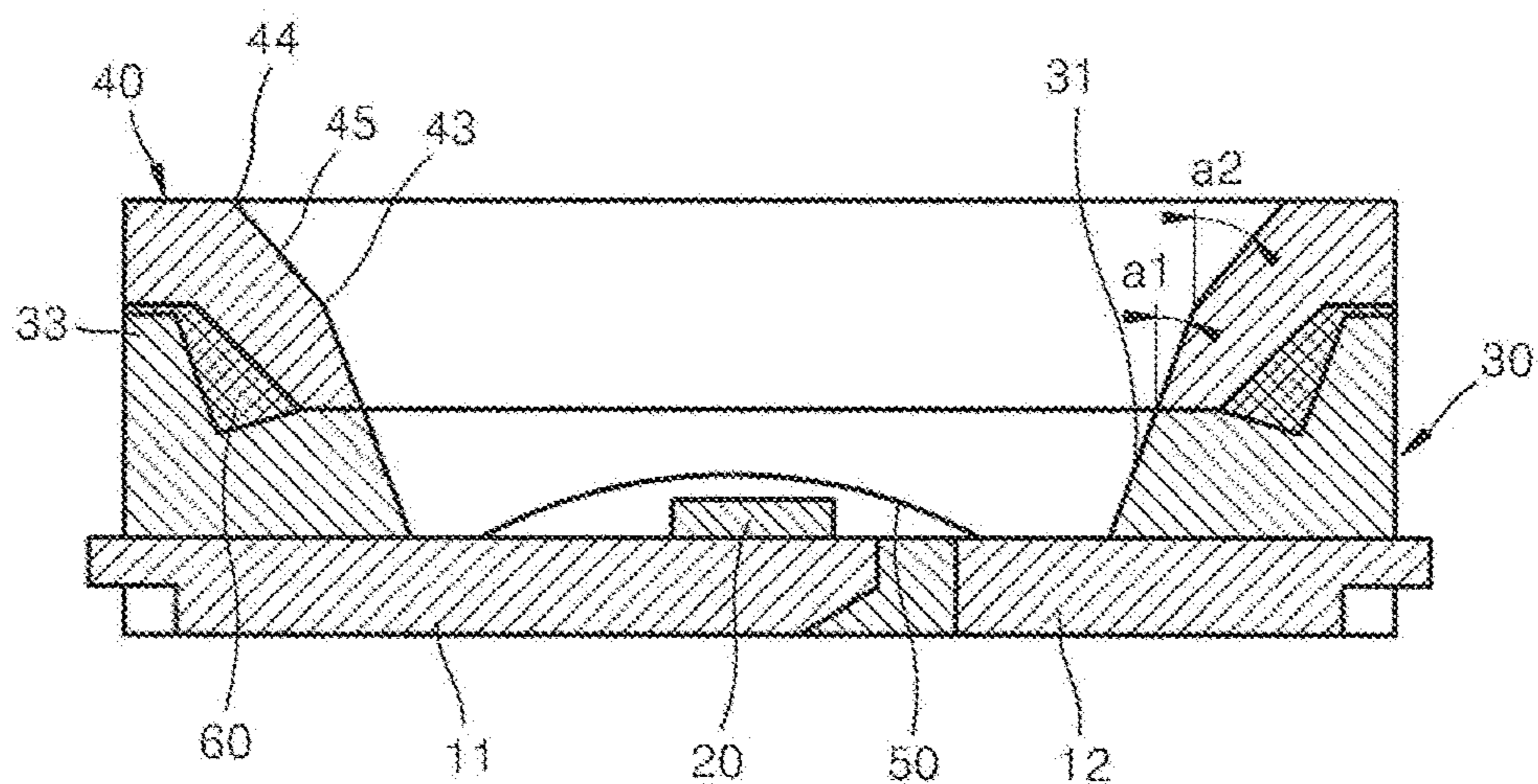
FIG. 13 (AMENDED)
