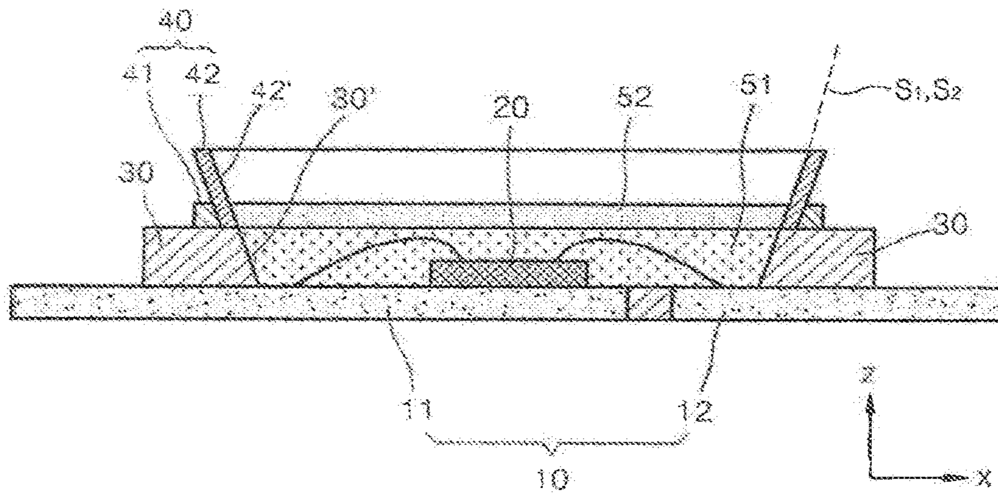
FIG. 1 (AMENDED)
