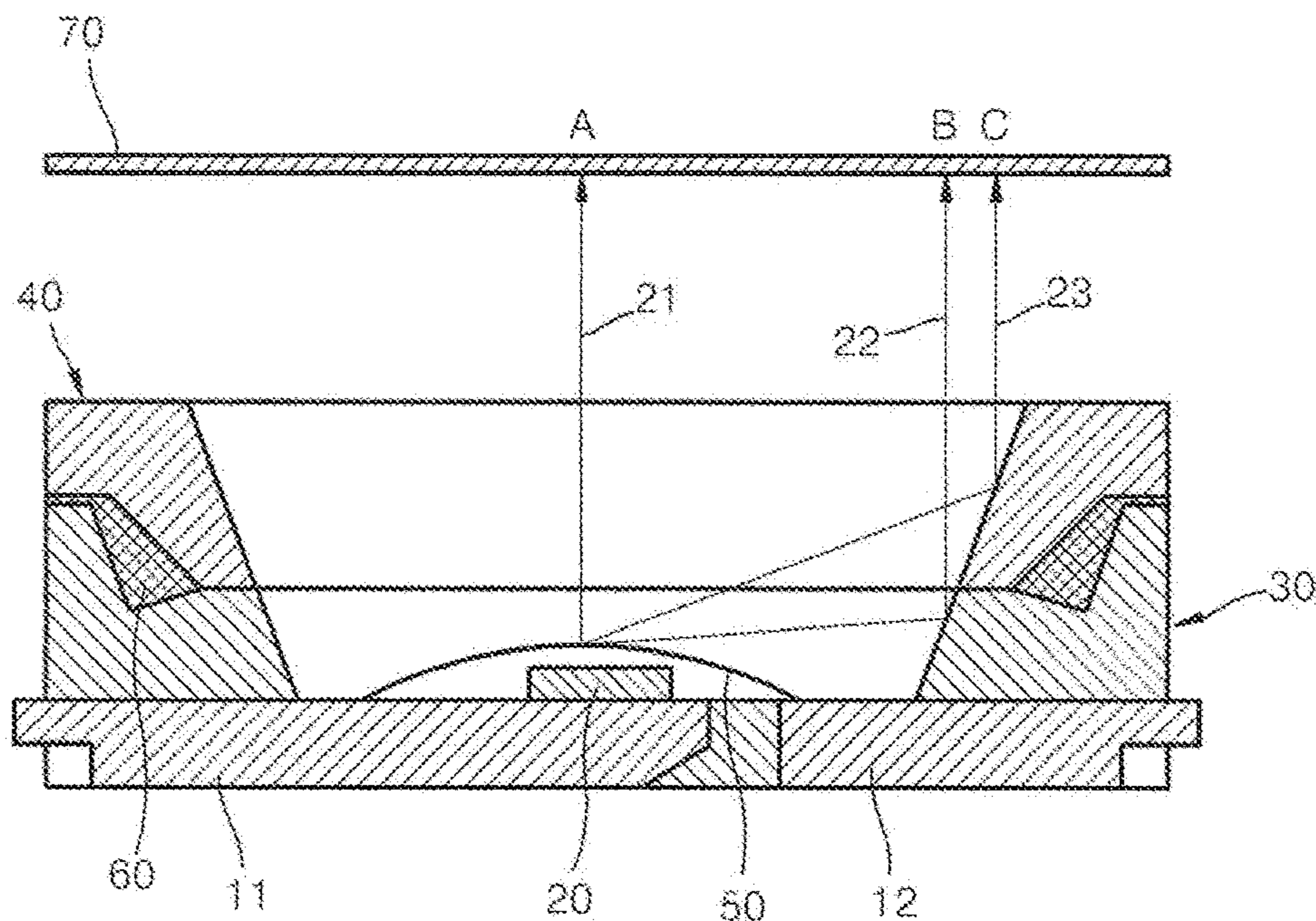
FIG. 14 (AMENDED)
