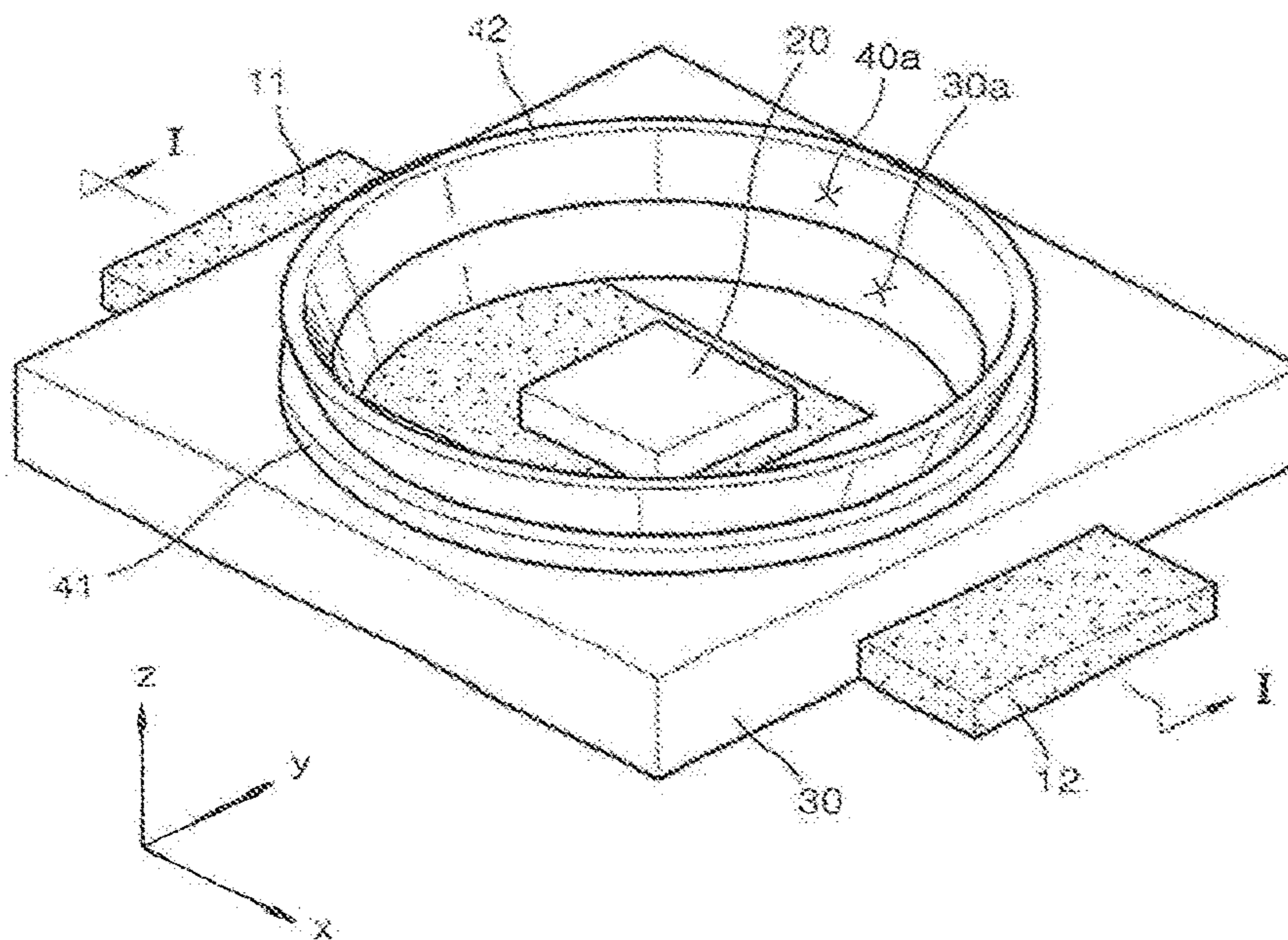
FIG. 2 (AMENDED)
