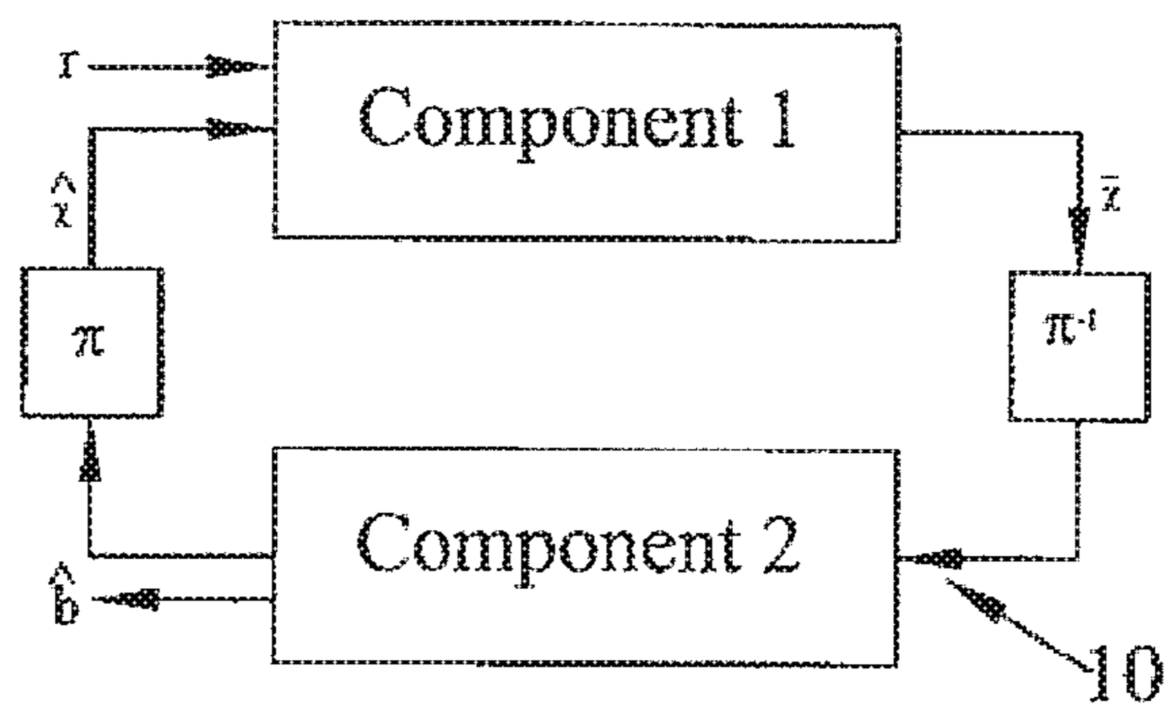
Generic iterative receiver structure
