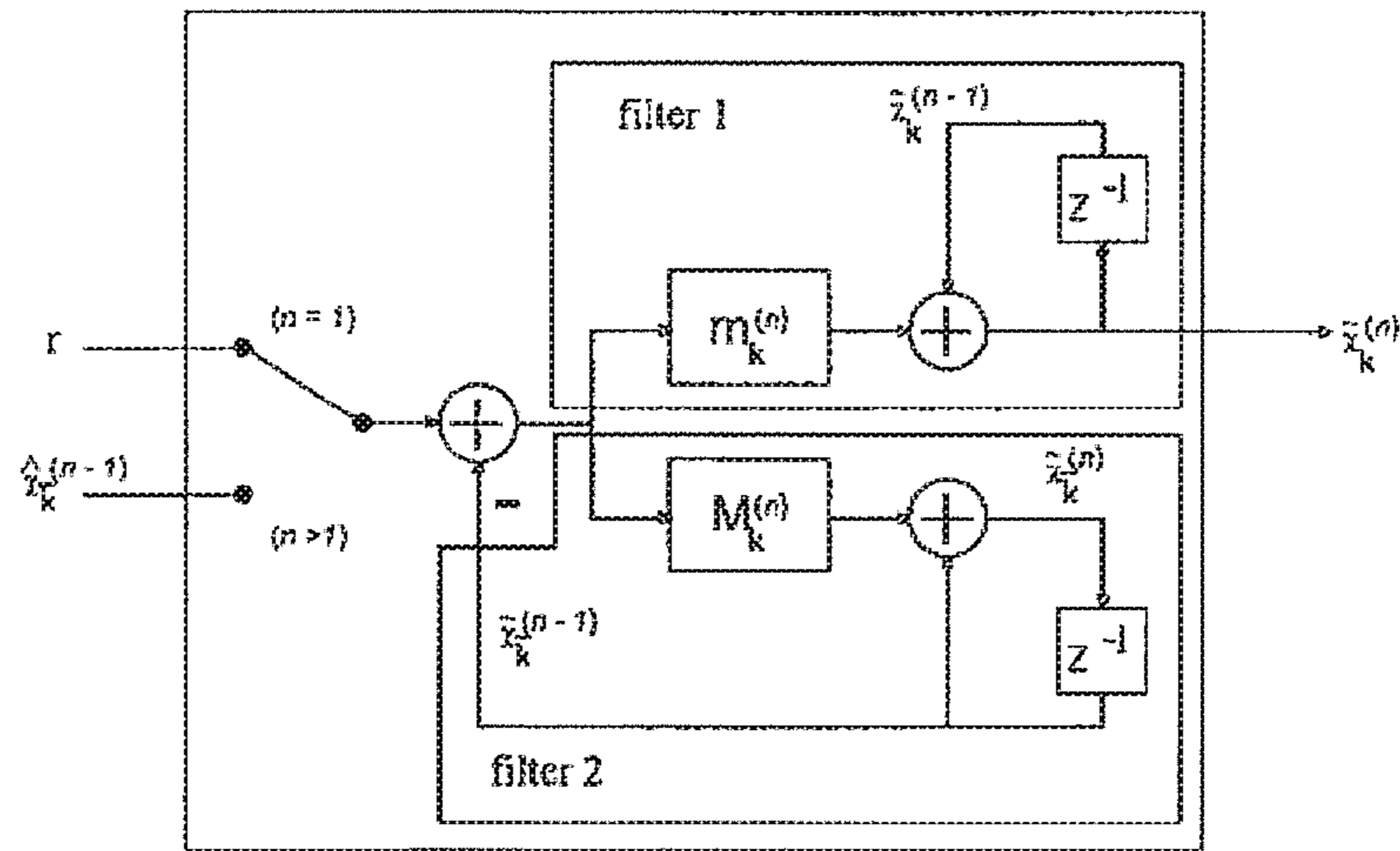
The recursive filter \Lambda_k^{(n)} For (n = 1) the input signal is r while for n \geq 2 the input signal is \hat{x}_k^{(n-1)} Figure 8
