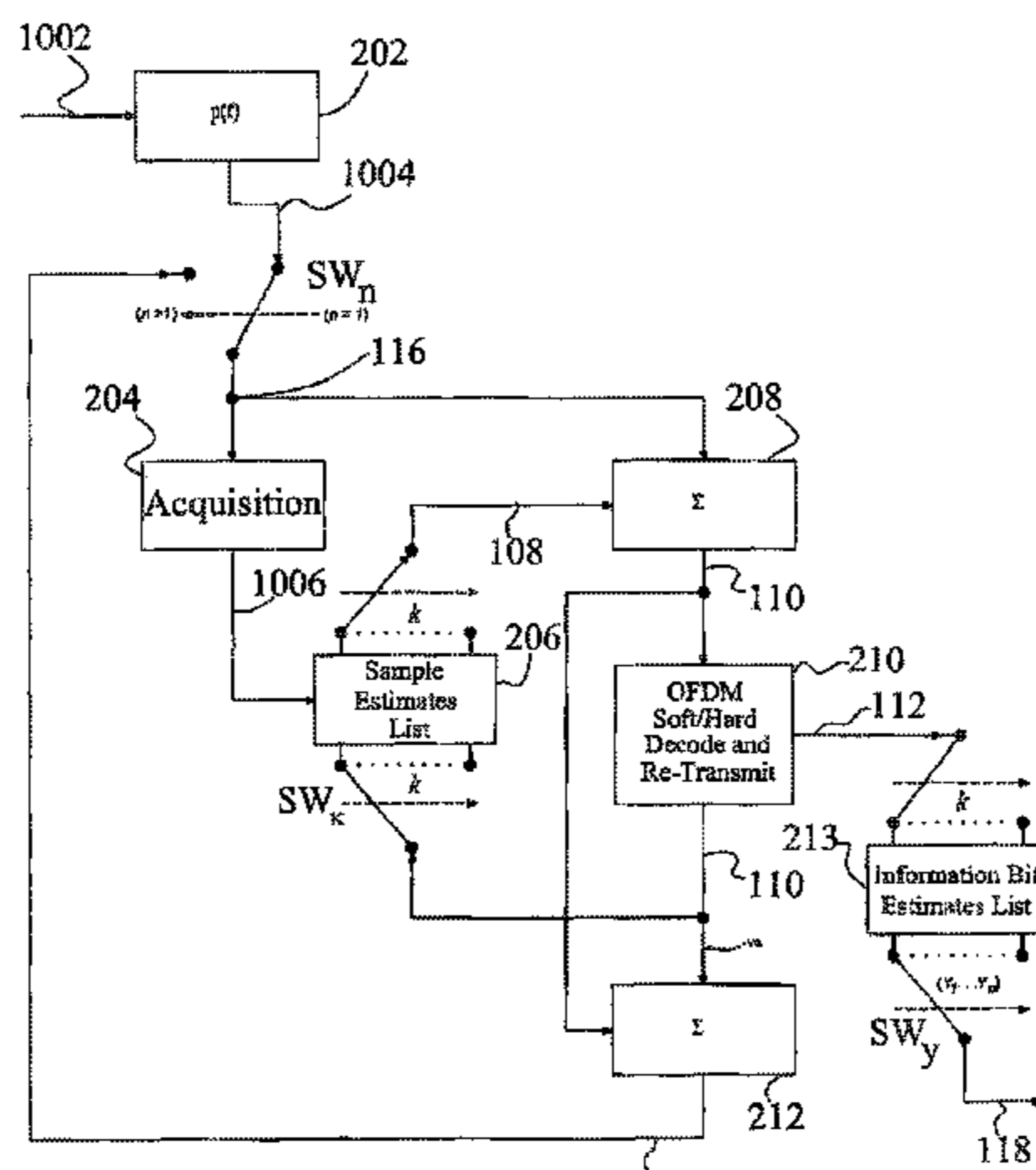
Iterative Interference Canceling Receiver Structure
