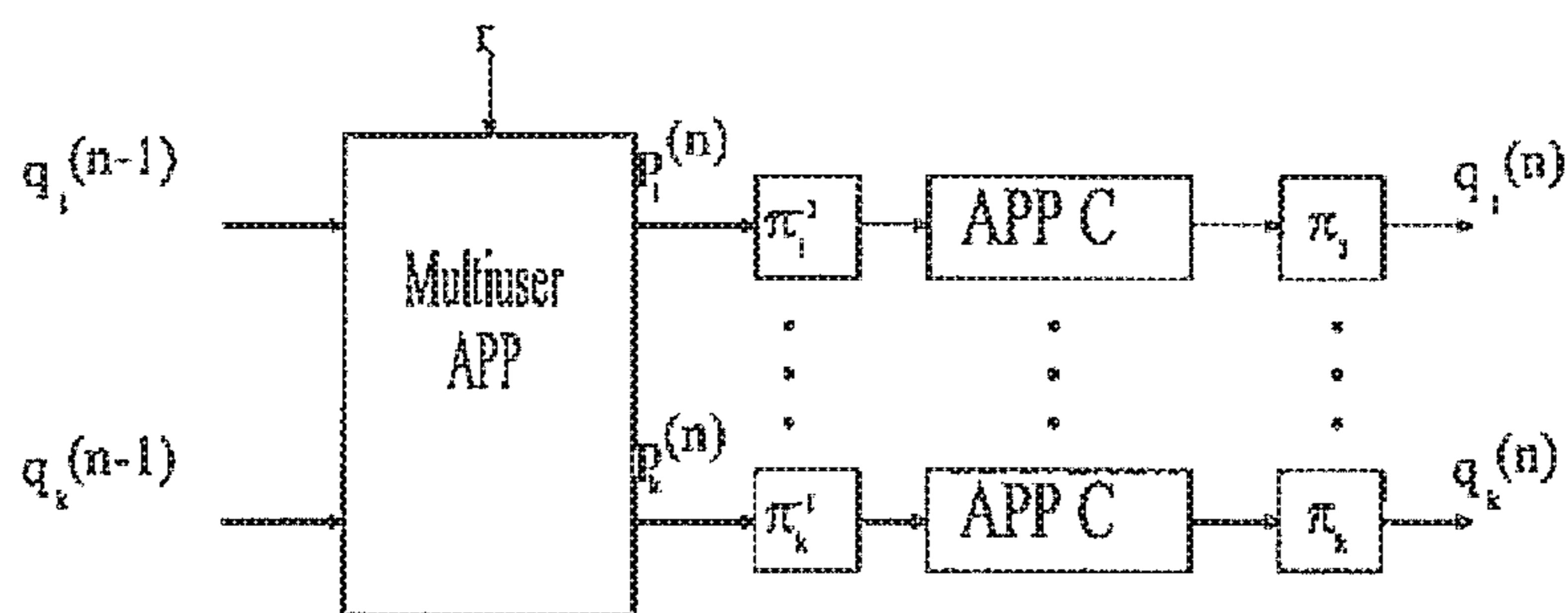
Canonical iterative multiuser decoder
