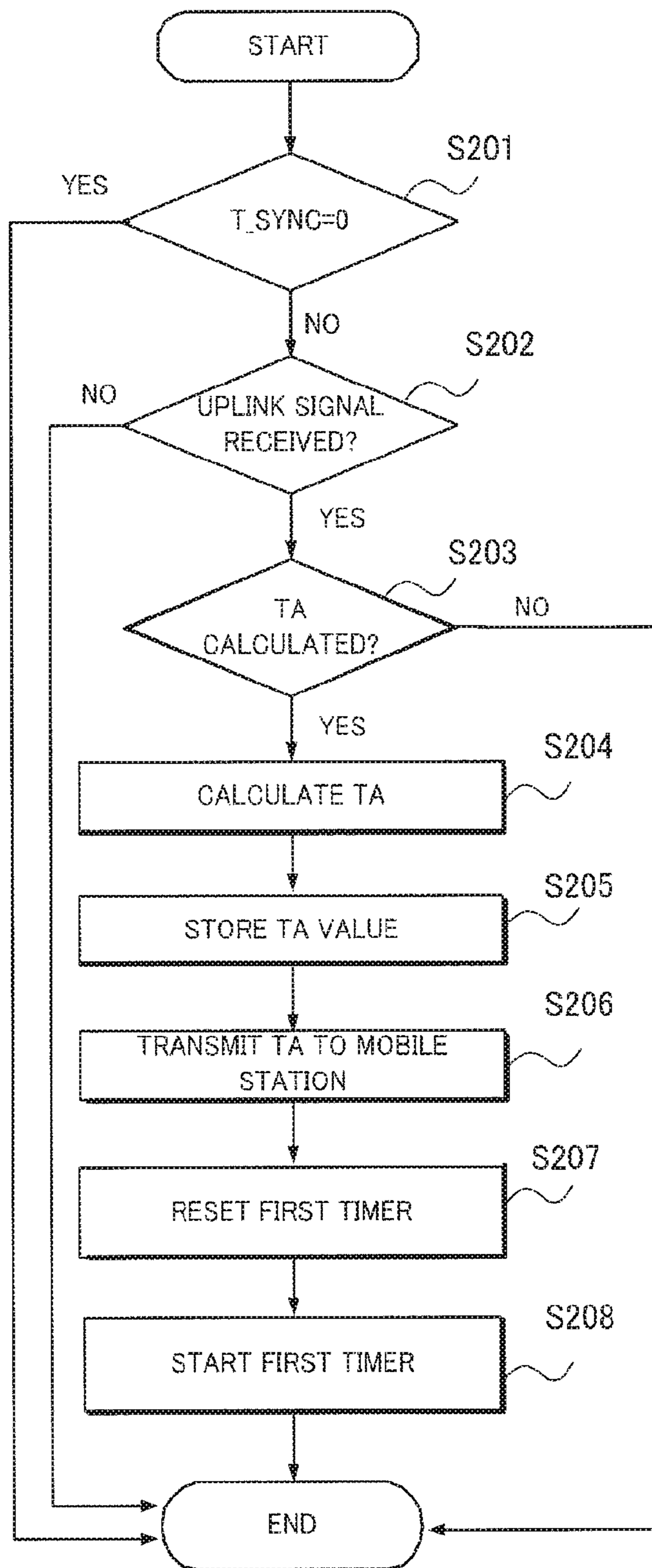
FIG. 16 DEEMED IN-SYNC STATE
