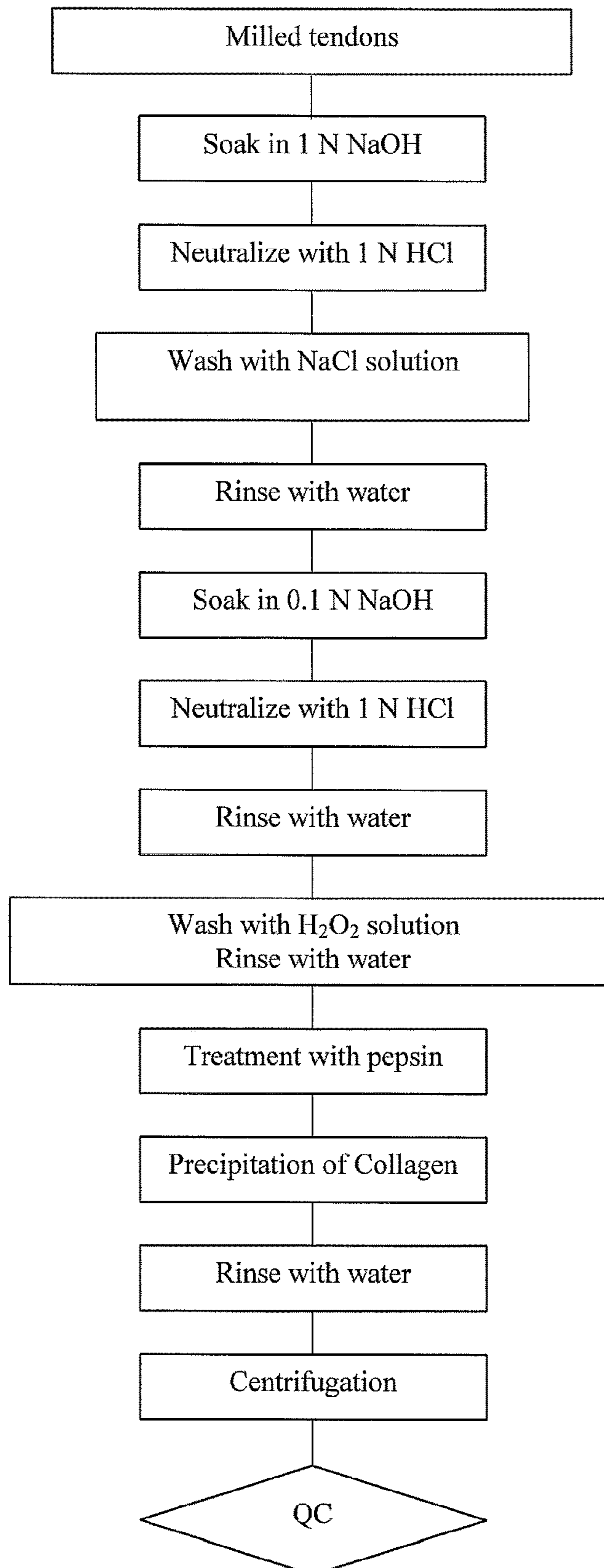
Flow Diagram for Production of Collagen
