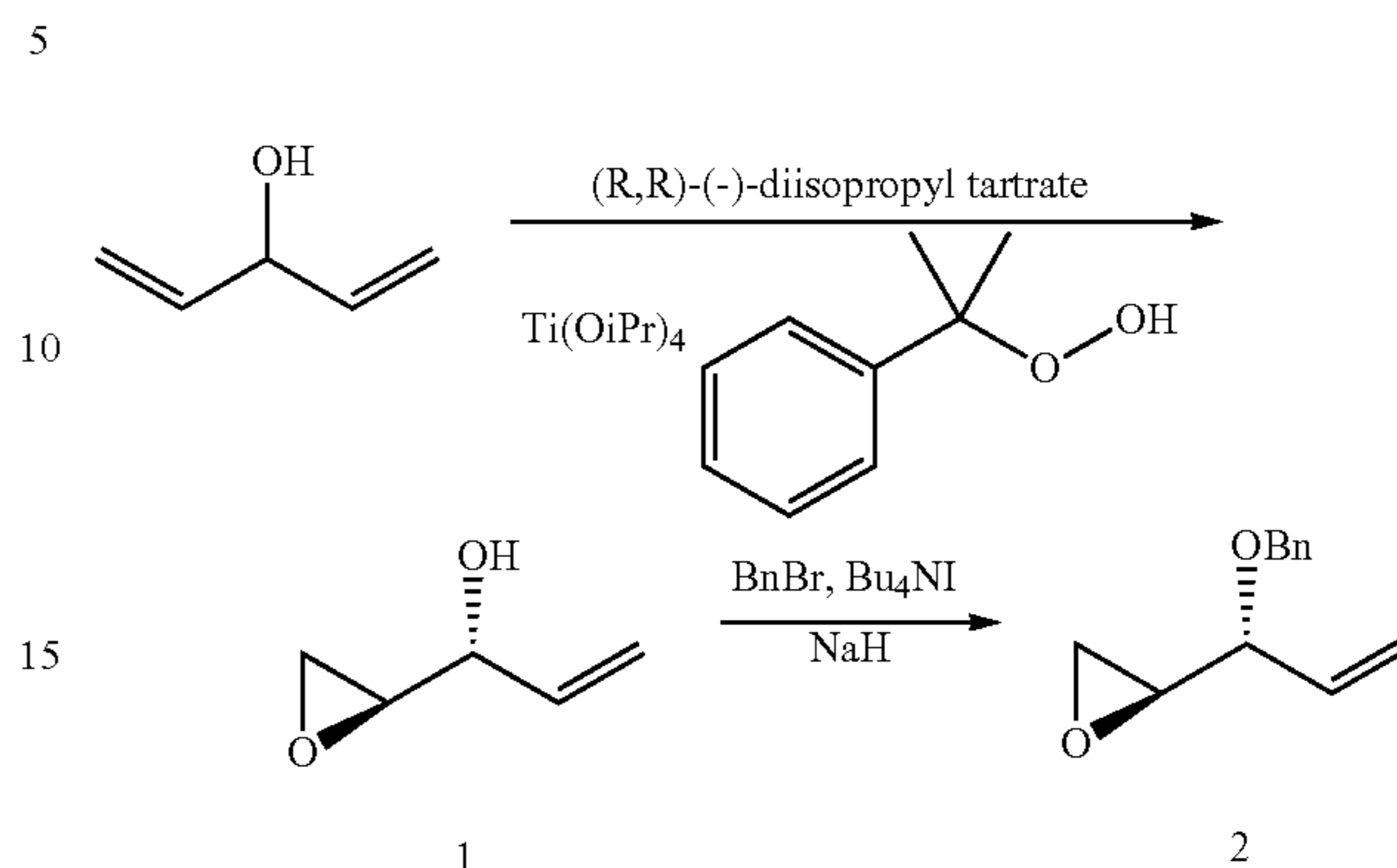
Synthesis of (2R,3R)-4-azido-2-benzyloxy-3-fluorobutanoic acid (5)
