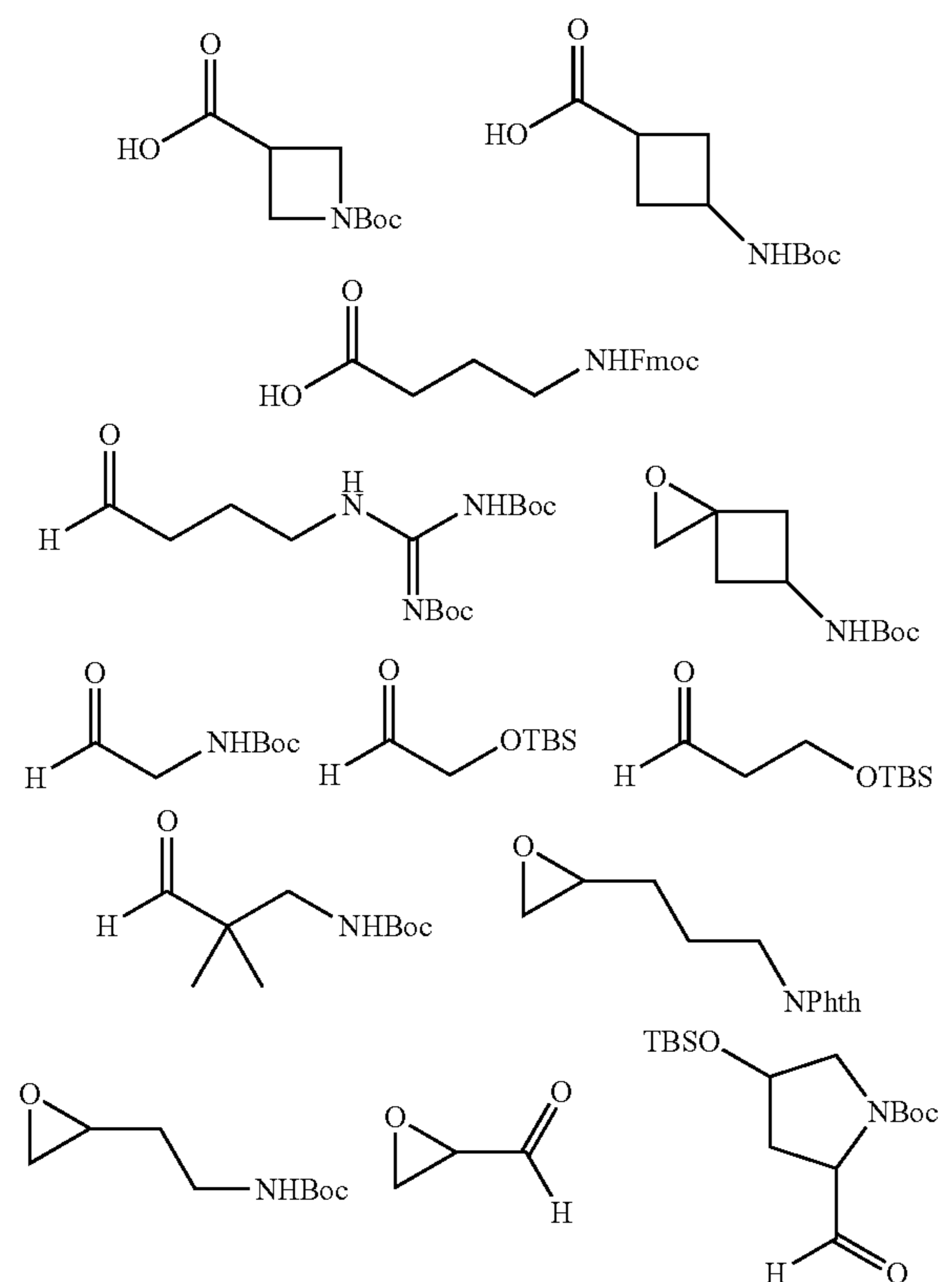
Representative N-6' Coupling Reagents
