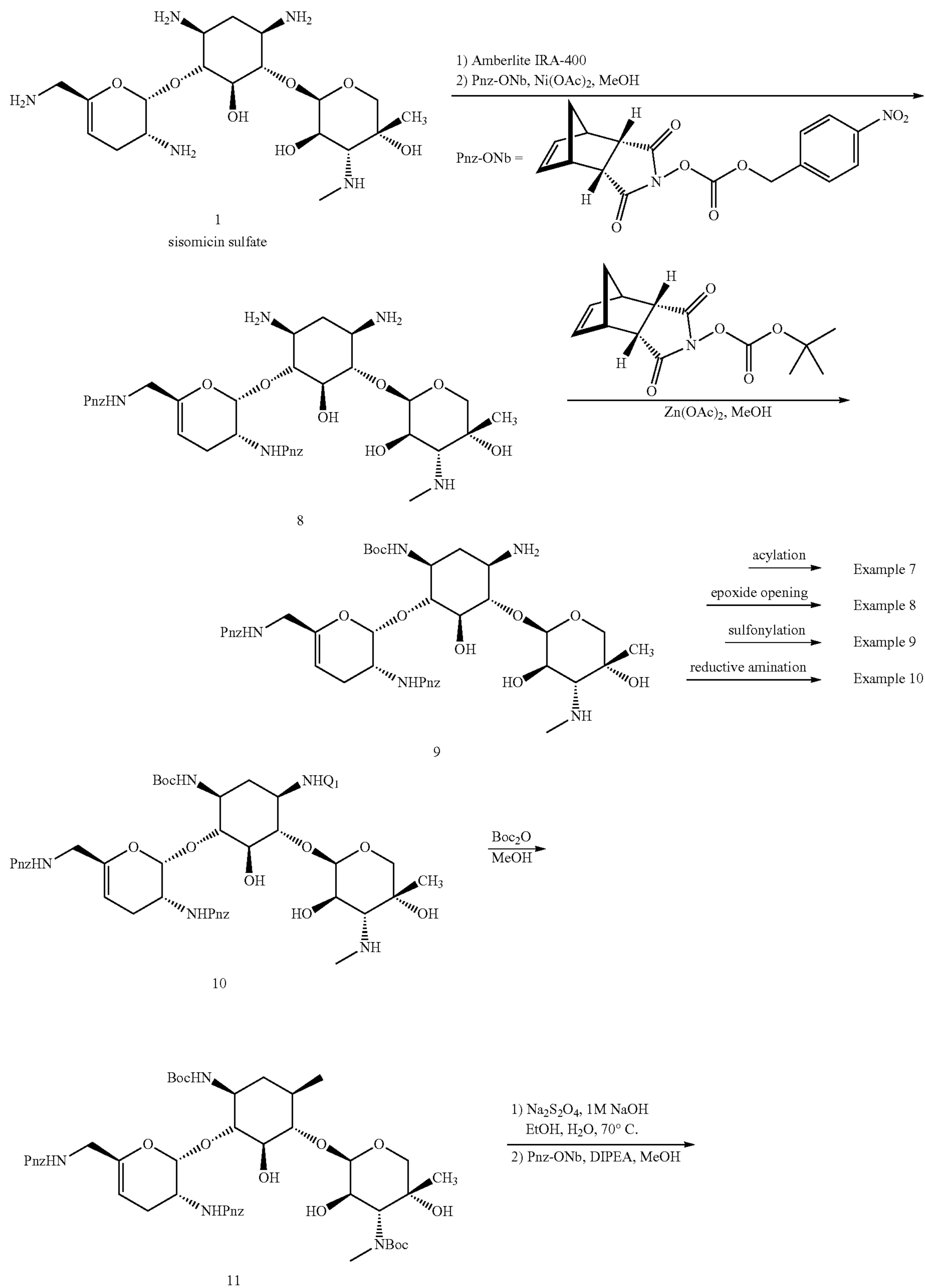
Scheme 2 N-2',N-1 Bis-substituted Sisomicin Analogs
