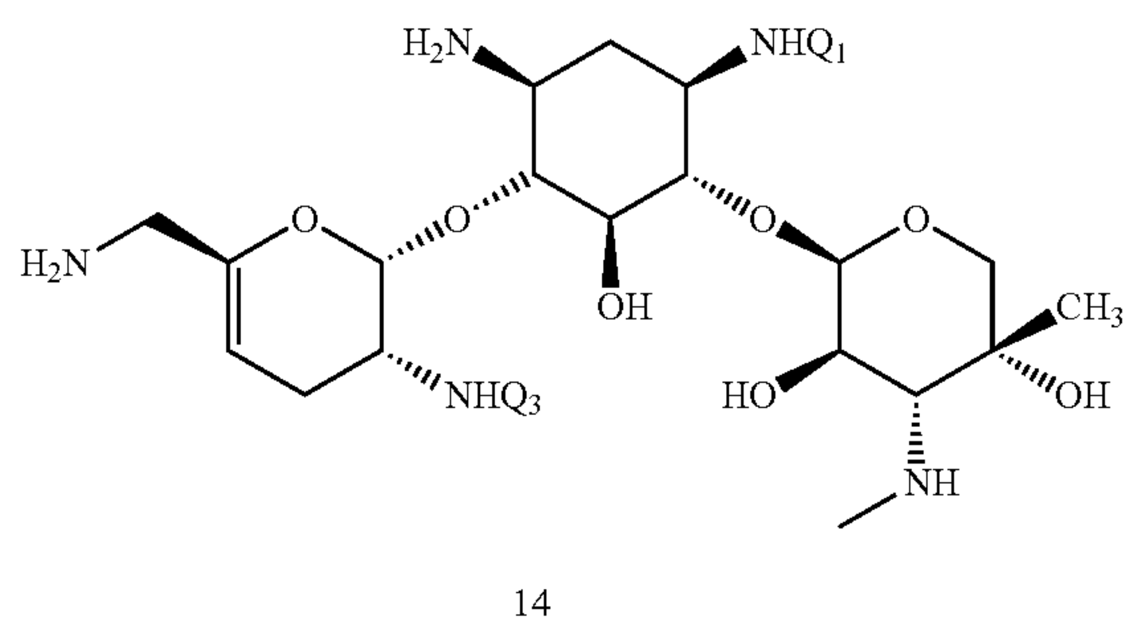
N-1,N-2'-bis-substituted sisomicin
