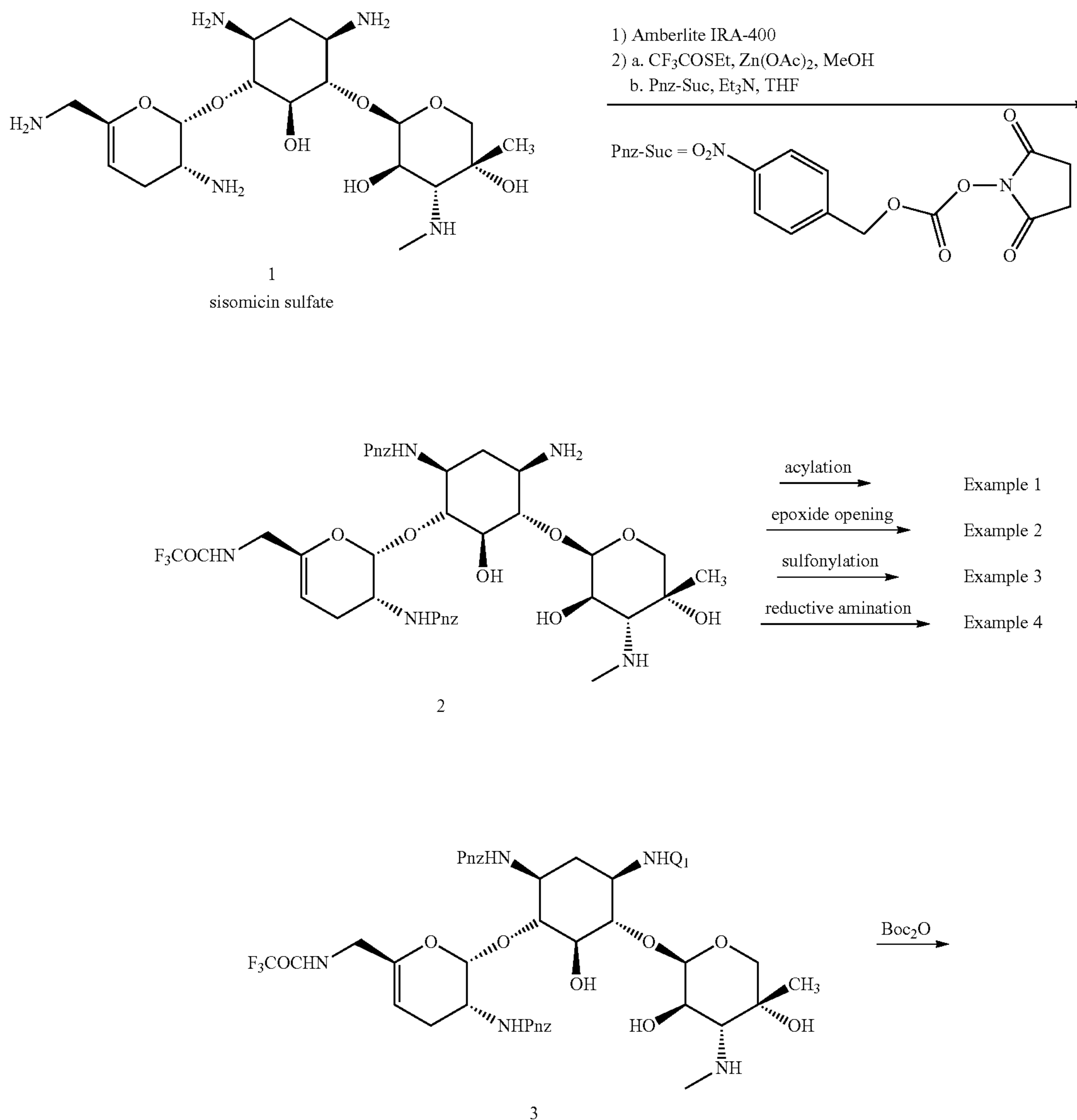
Scheme 1 N-6',N-1 Bis-substituted Sisomicin Analogs
