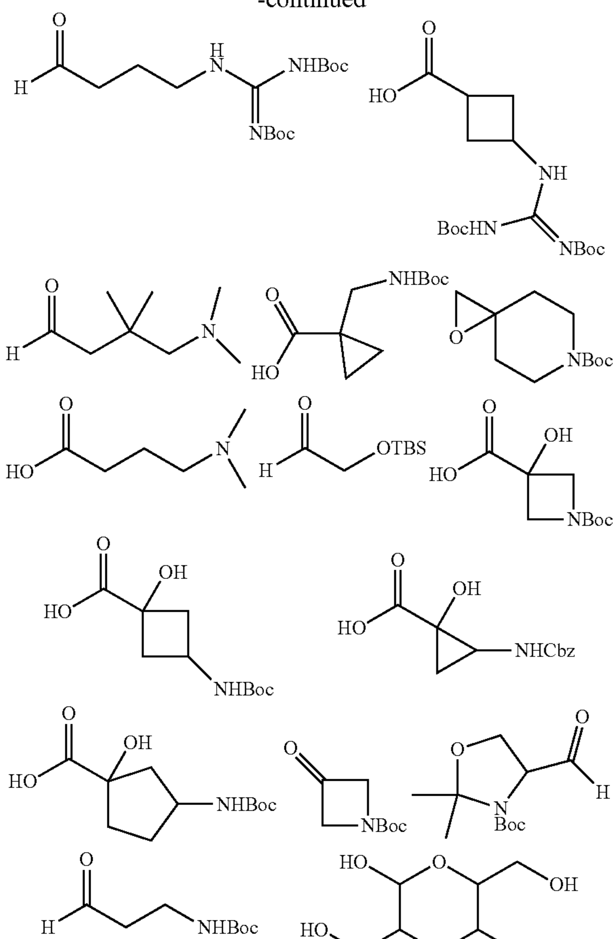
Representative N-6' Coupling Reagents
