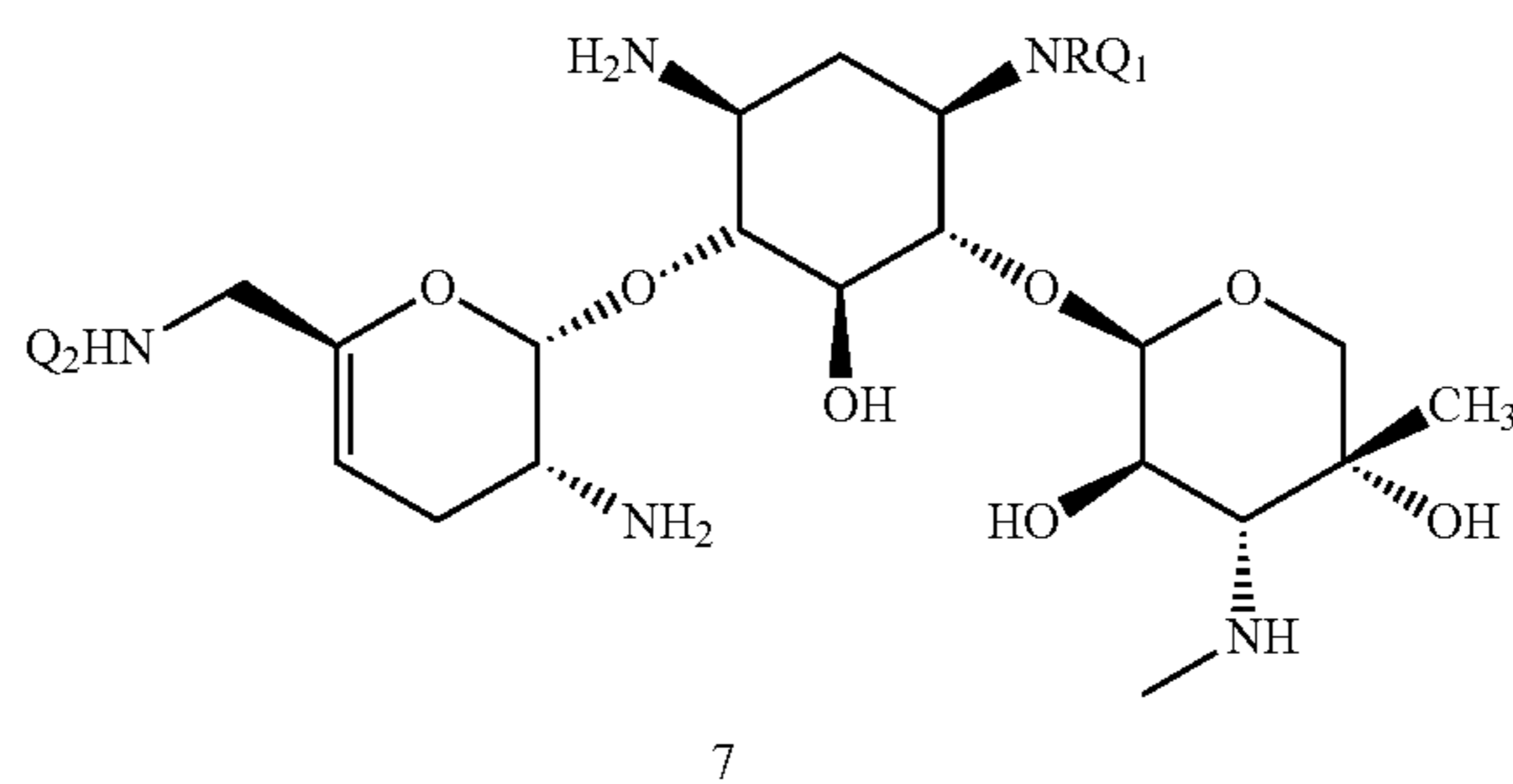
N-1,N-6'-bis-substituted sisomicin
