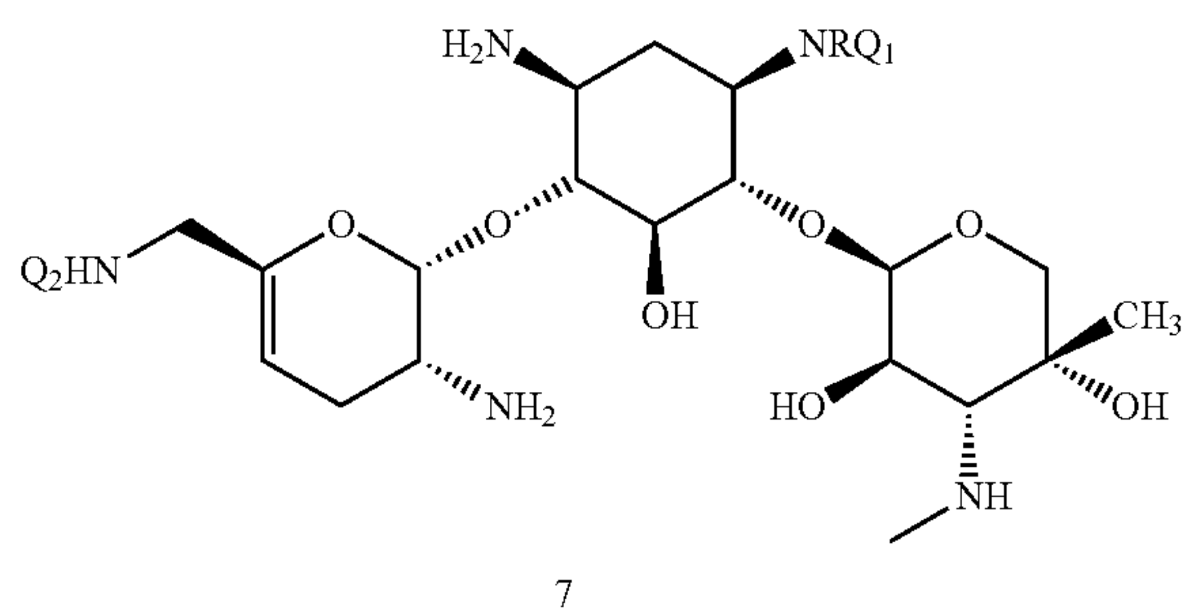
N-1,N-6'-bis-substituted sisomicin
