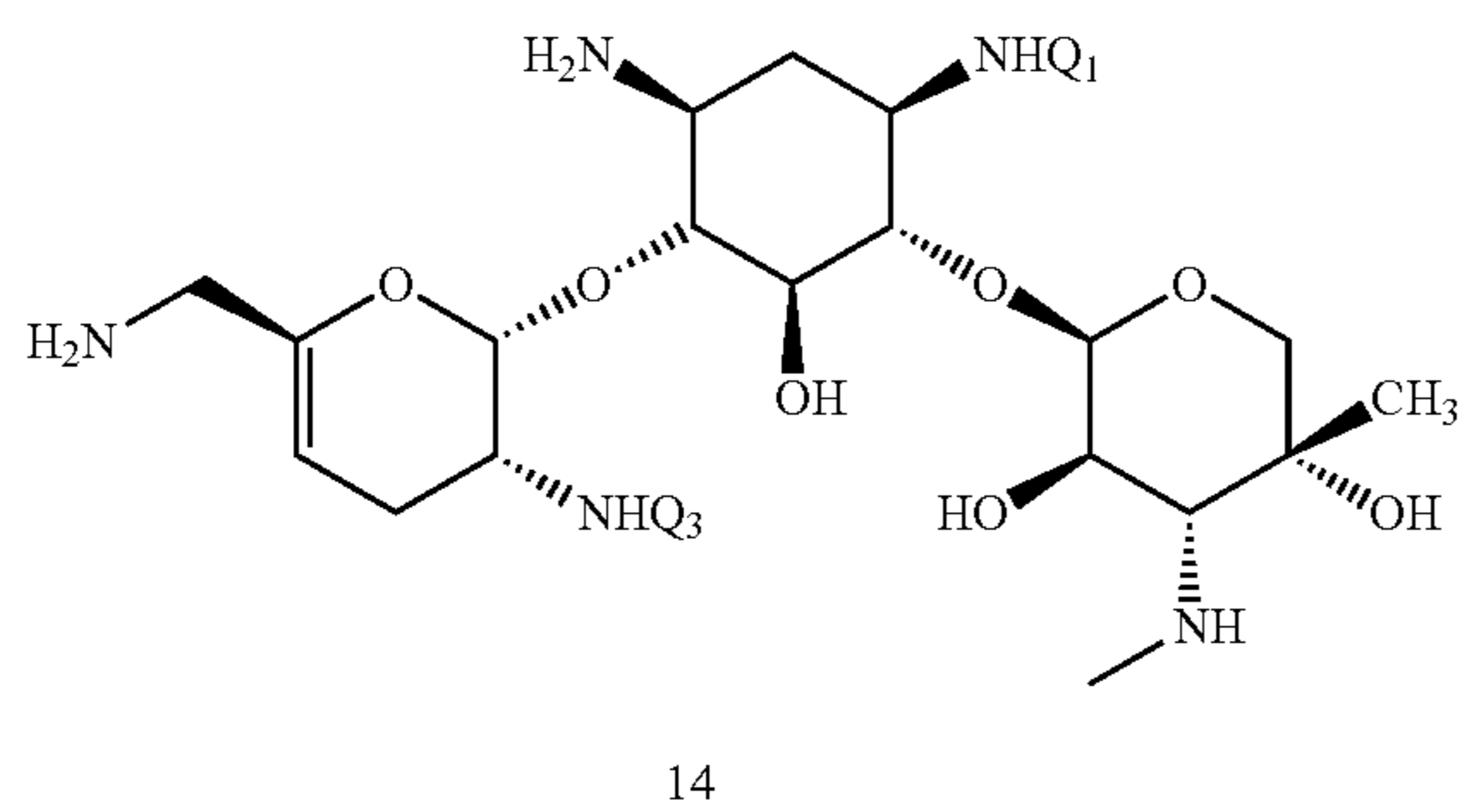
N-1,N-2'-bis-substituted sisomicin
