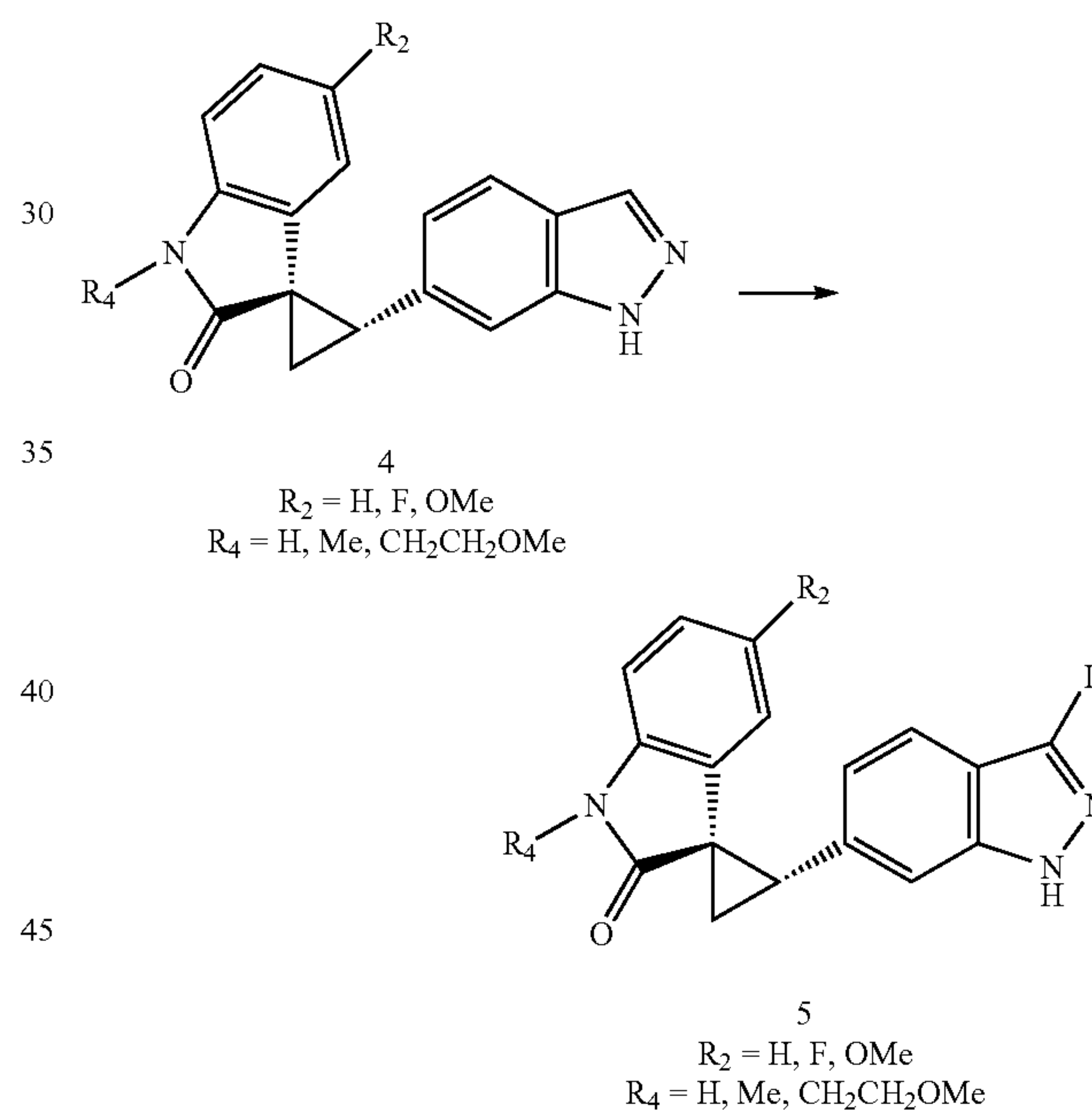
SCHEME 7
