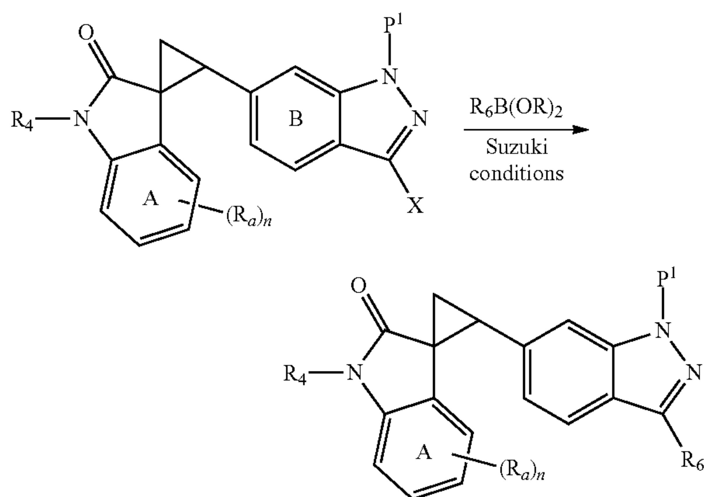
SCHEME 2
