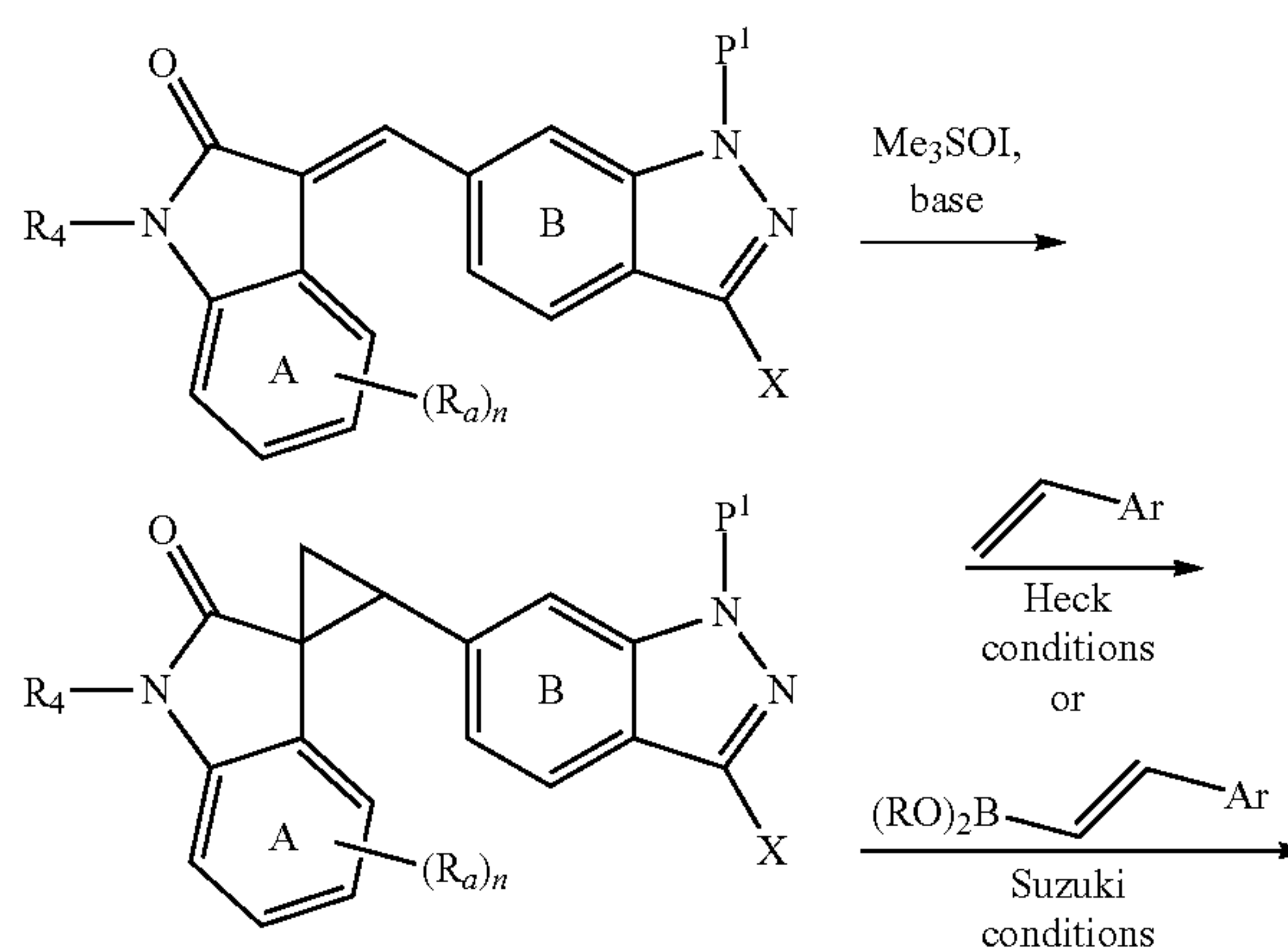
Scheme 1
