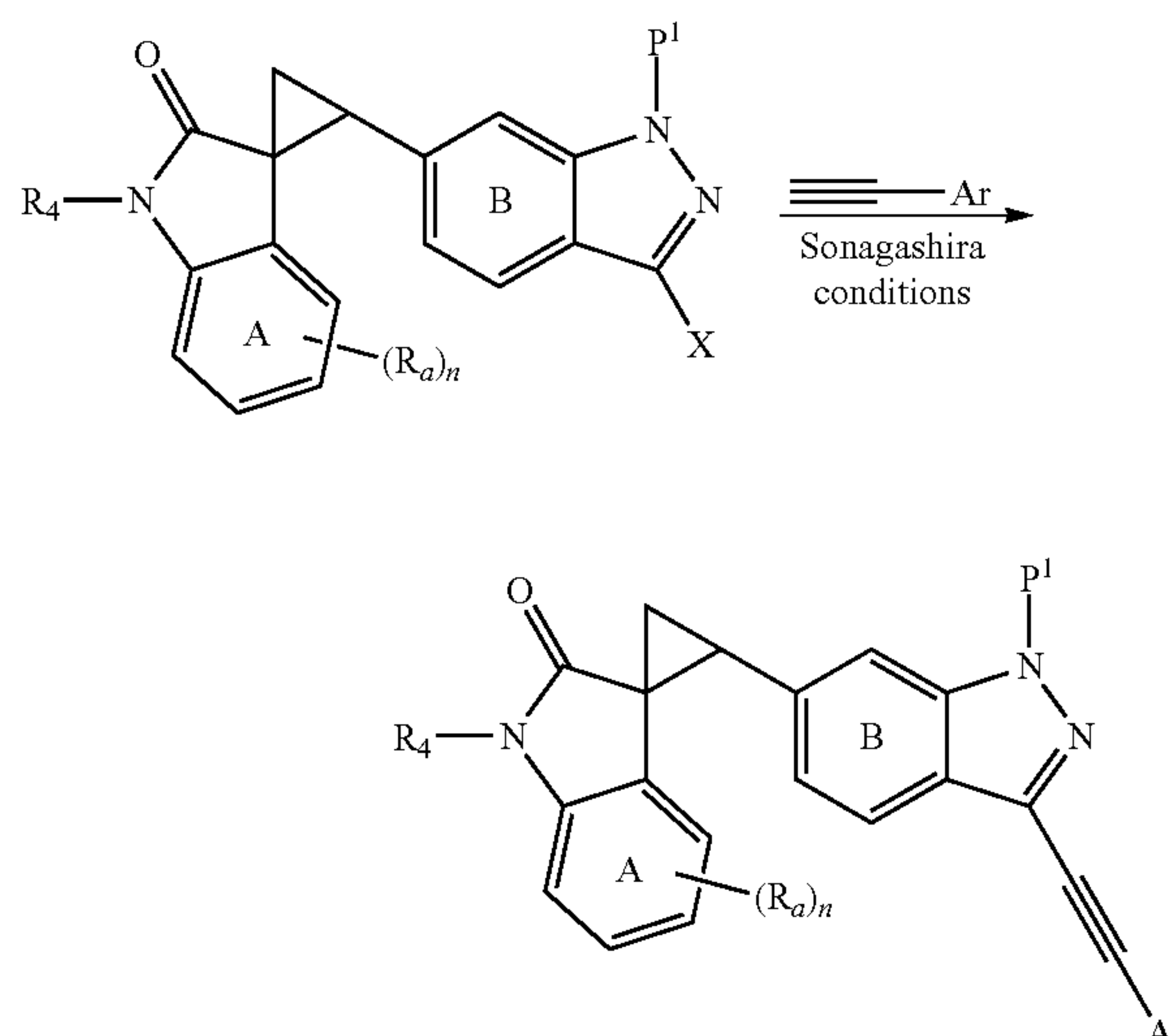
SCHEME 3
