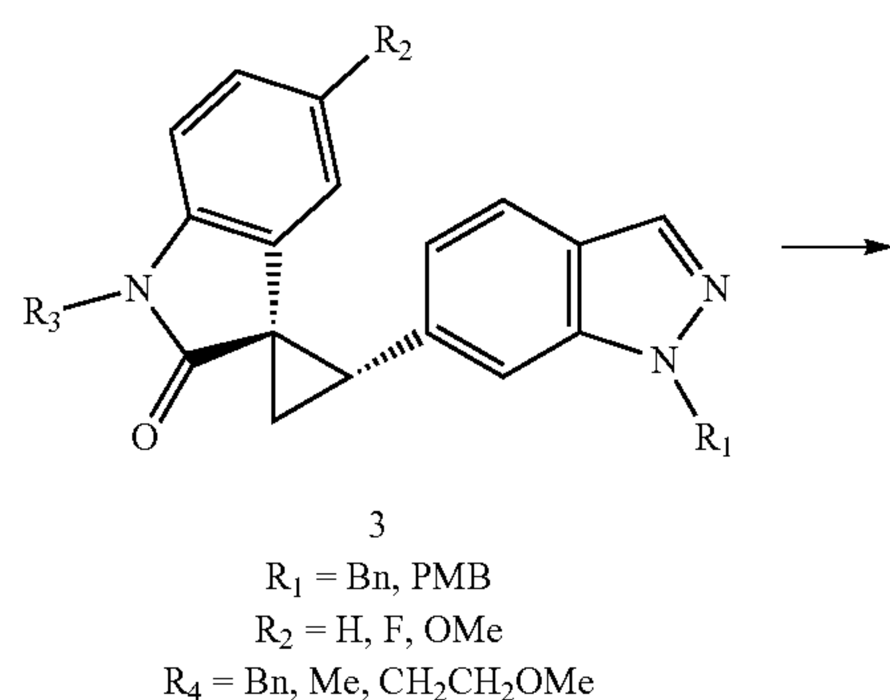
Scheme 6
