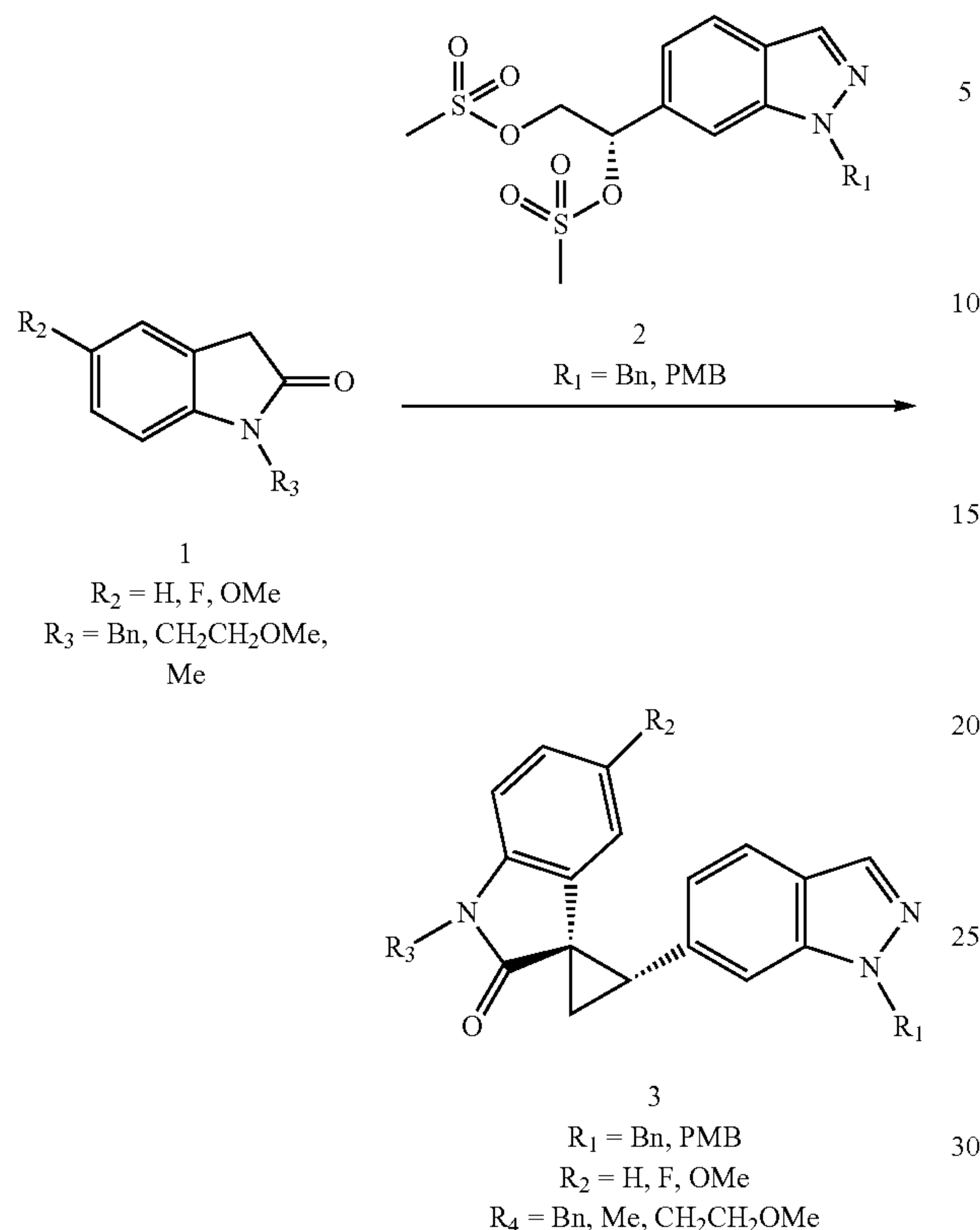
SCHEME 5
