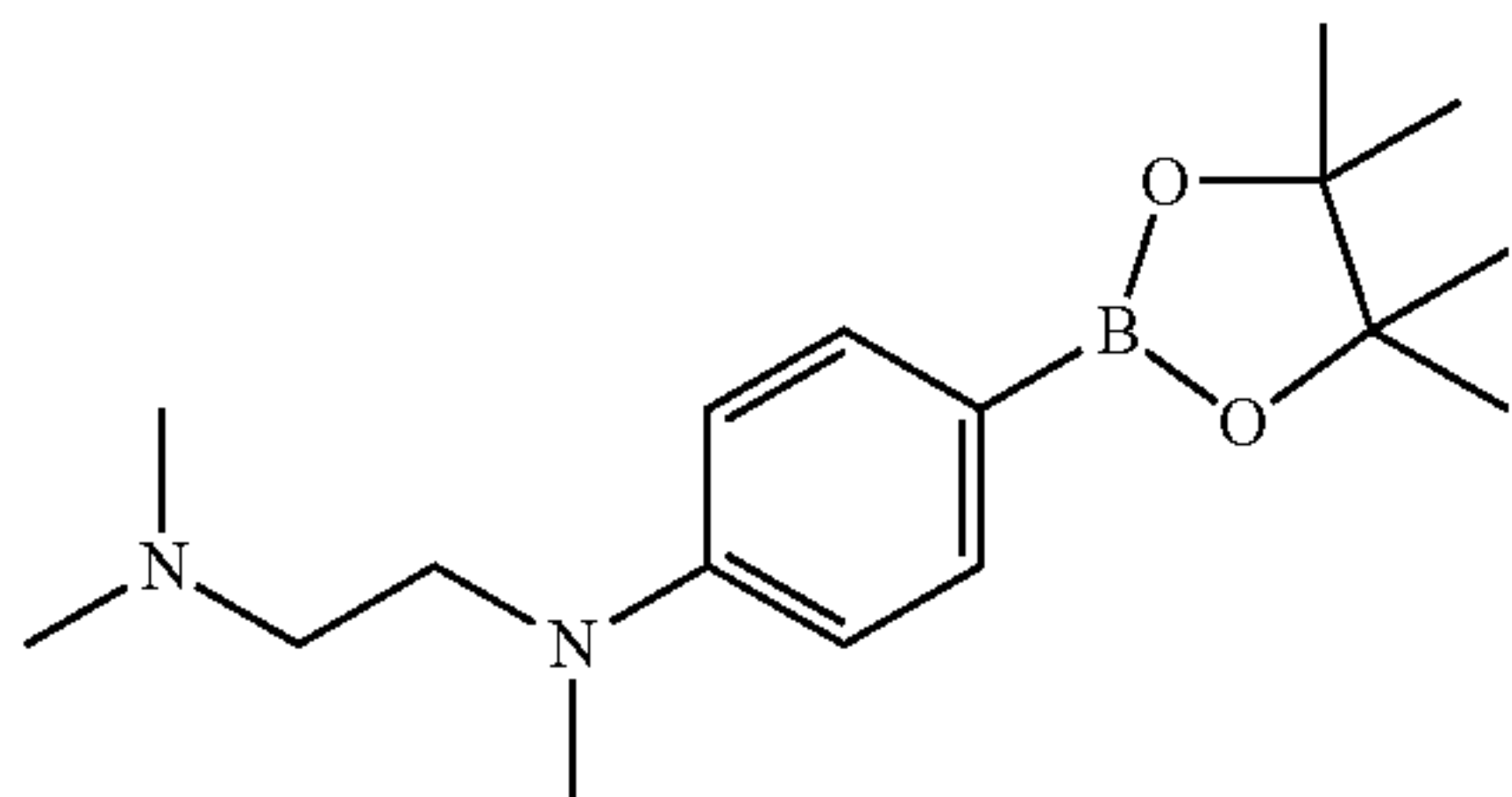
A. N-(4-Iodophenyl)-N,N',N'-trimethylethane-1,2-diamine
