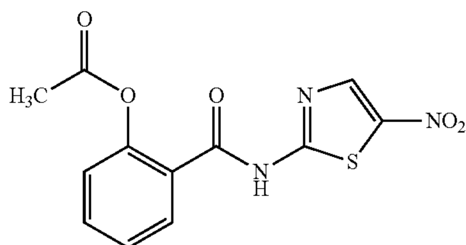
Nitazoxanide
