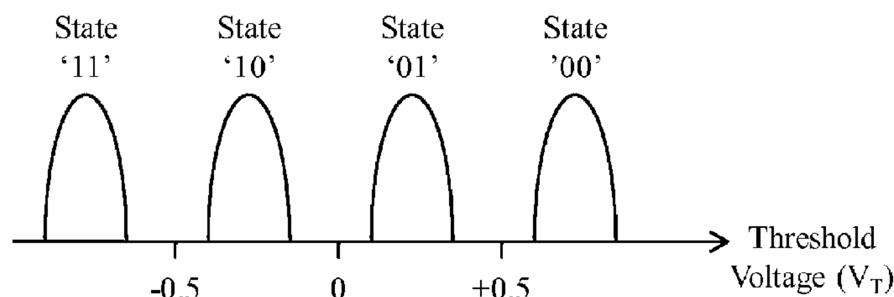
Multi-Level Cell
