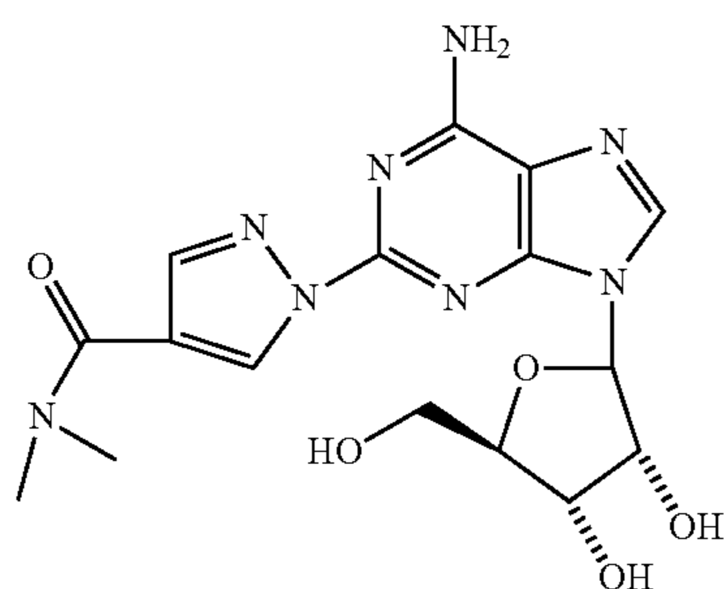
(1-{9-[(4S,2R,3R,5R)-3,4-dihydroxy-5-(hydroxymethyl)oxolan-2-yl]-6-aminopurin-2-yl}pyrazol-4-yl)-N,N-dimethylcarboxamide (18)
