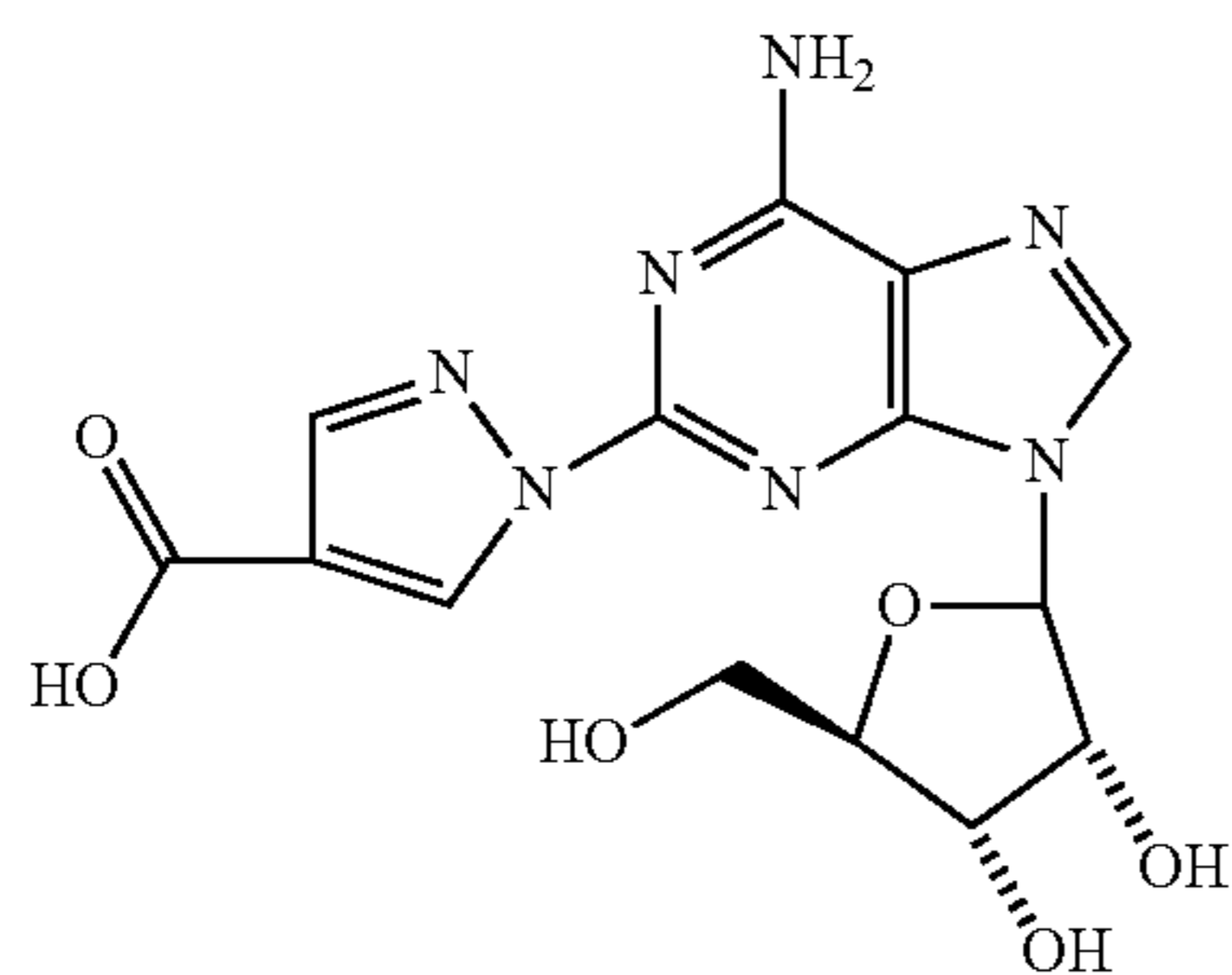
1-{9-[(4S,2R,3R,5R)-3,4-dihydroxy-5-(hydroxymethyl)oxolan-2-yl]-6-aminopurin-2-yl}pyrazole-4-carboxylic acid (17)
