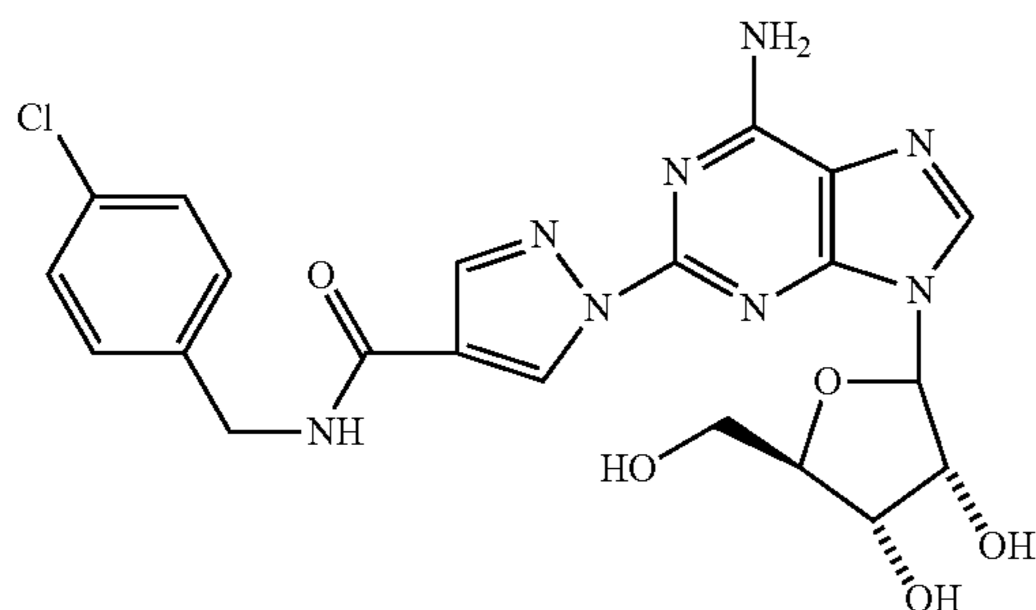
(1-{9-[(4S,2R,3R,5R)-3,4-dihydroxy-5-(hydroxymethyl)oxolan-2-yl]-6-aminopurin-2-yl}pyrazol-4-yl)-N-[(4-chlorophenyl)methyl]carboxamide (22)
