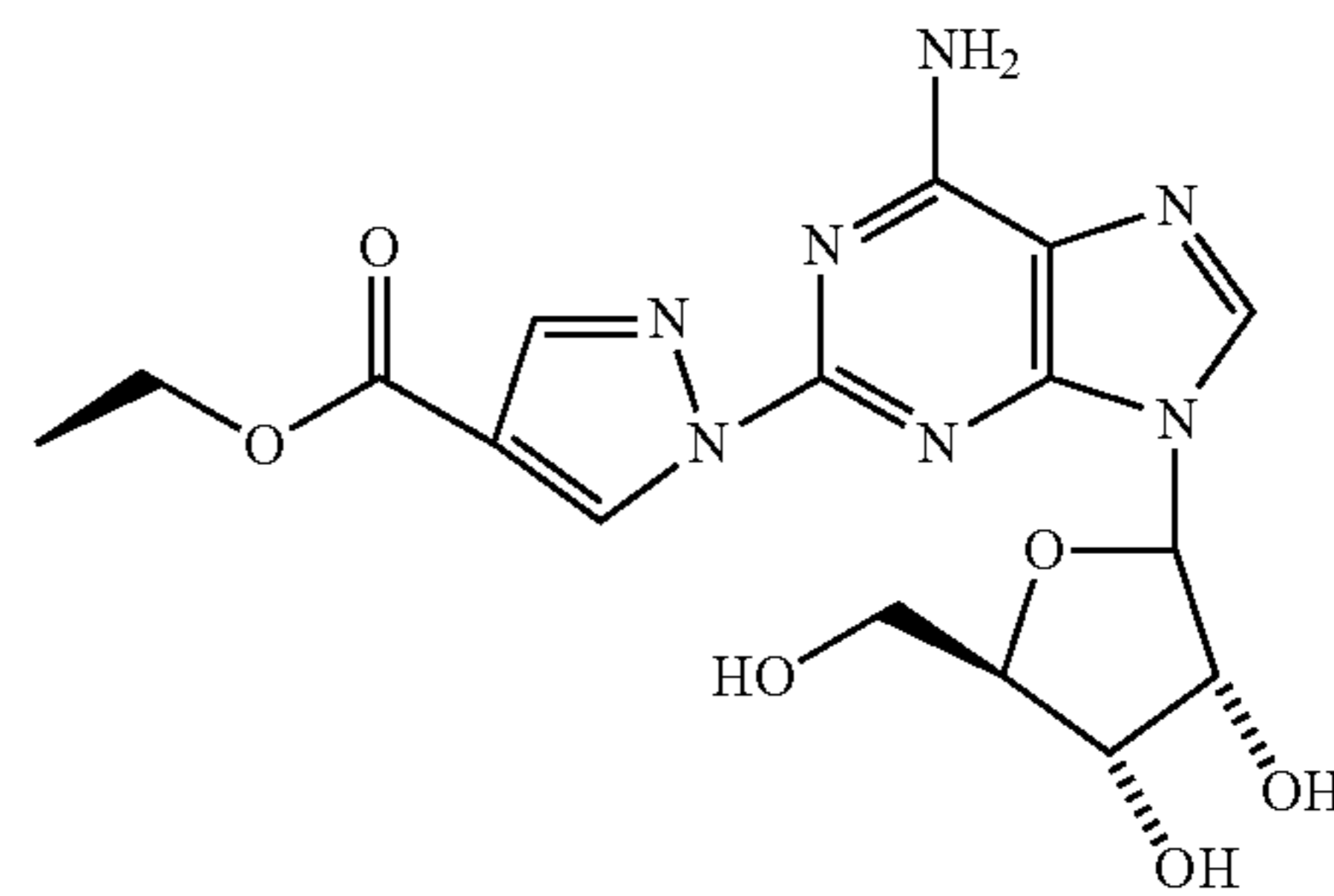
Ethyl 1-{9-[(4S,2R,3R,5R)-3,4-dihydroxy-5-(hydroxymethyl)oxolan-2-yl]-6-aminopurin-2-yl}pyrazole-4-carboxylate (12)
