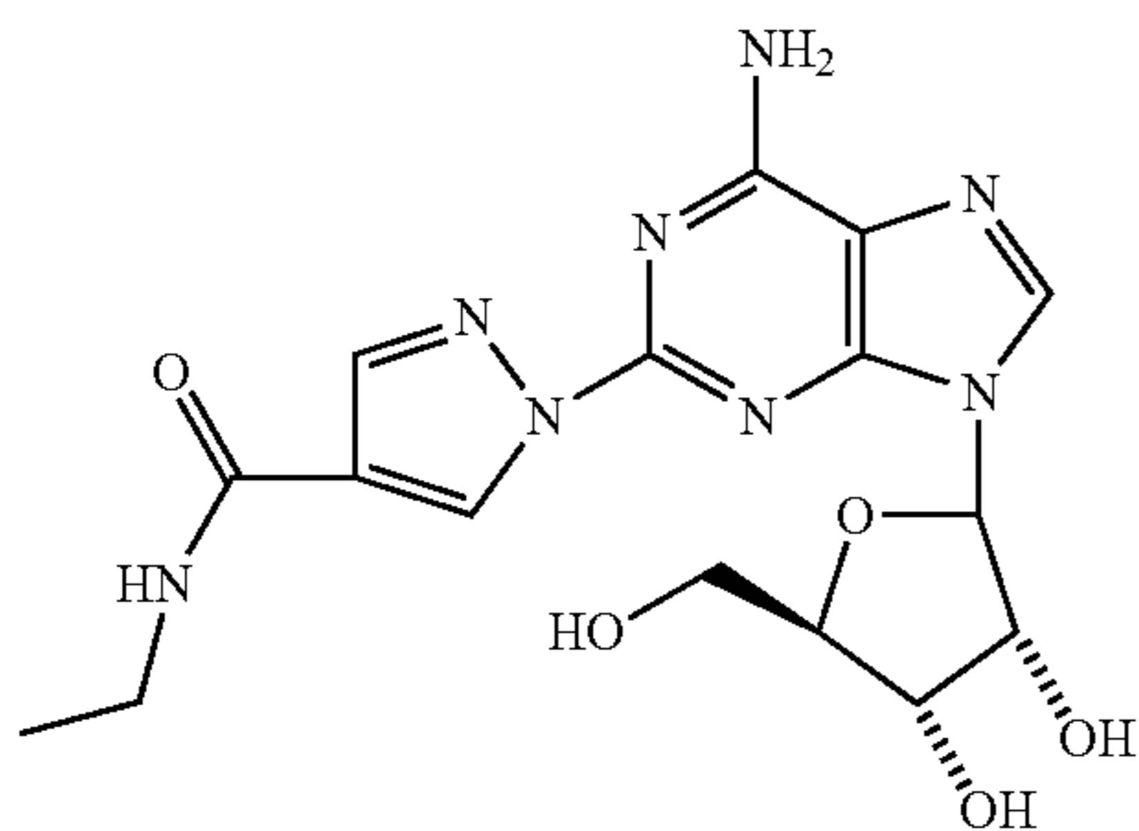
(1-{9-[(4S,2R,3R,5R)-3,4-dihydroxy-5-(hydroxymethyl)oxolan-2-yl]-6-aminopurin-2-yl}pyrazol-4-yl)-N-ethylcarboxamide (19)
