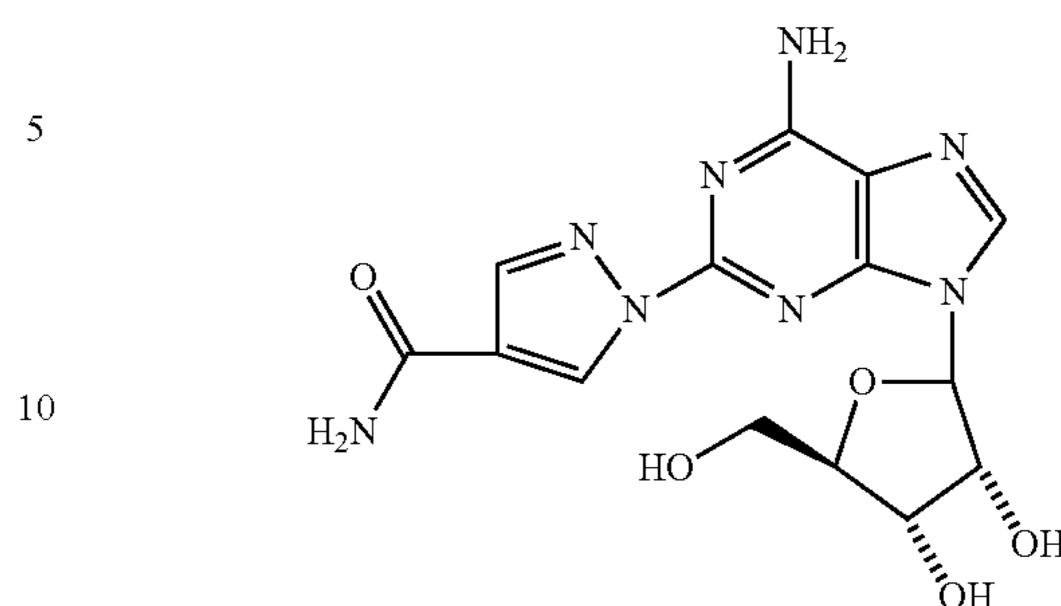
1-{9-[(4S,2R,3R,5R)-3,4-dihydroxy-5-(hydroxymethyl)oxolan-2-yl]-6-aminopurin-2-yl}pyrazole-4-carboxamide (20)
