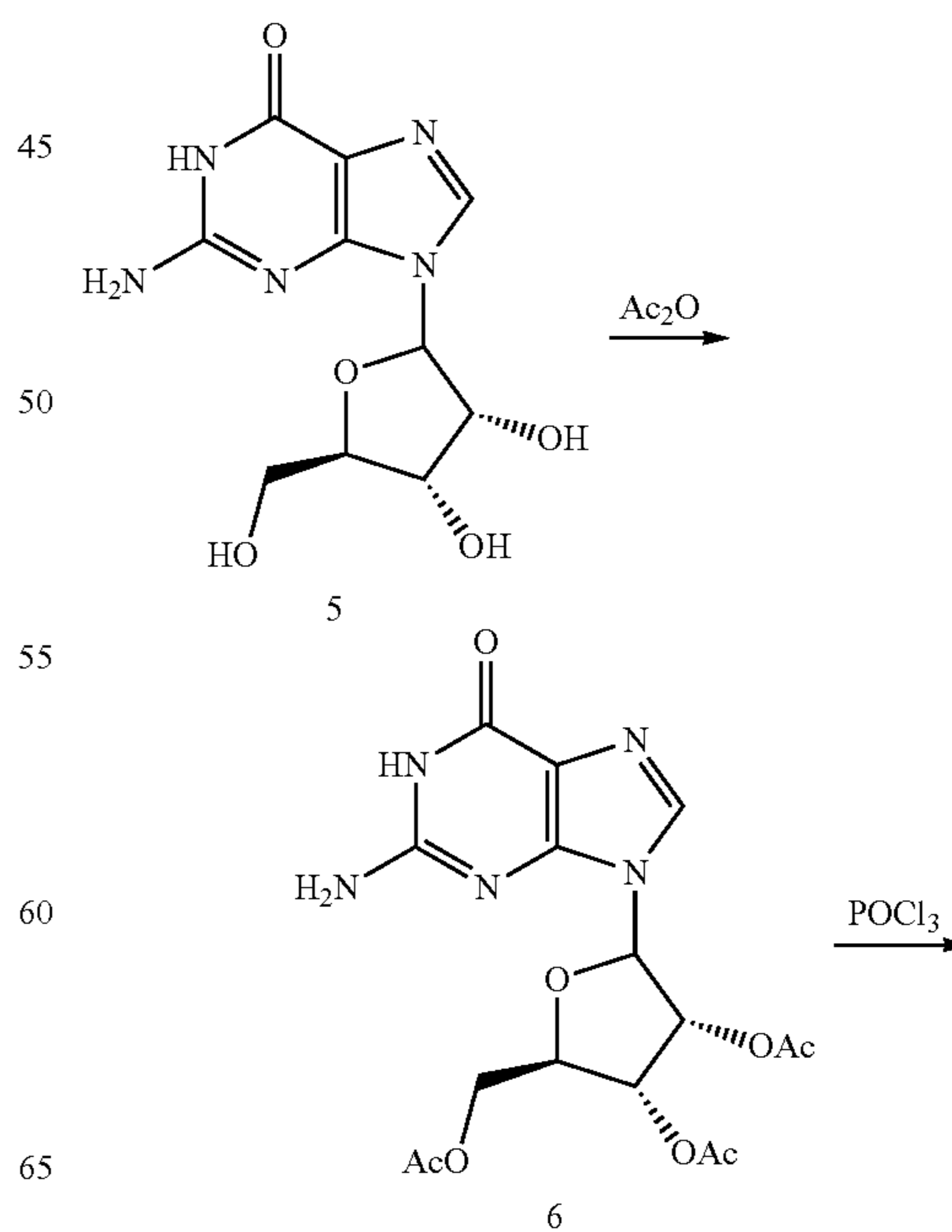
Scheme 3
