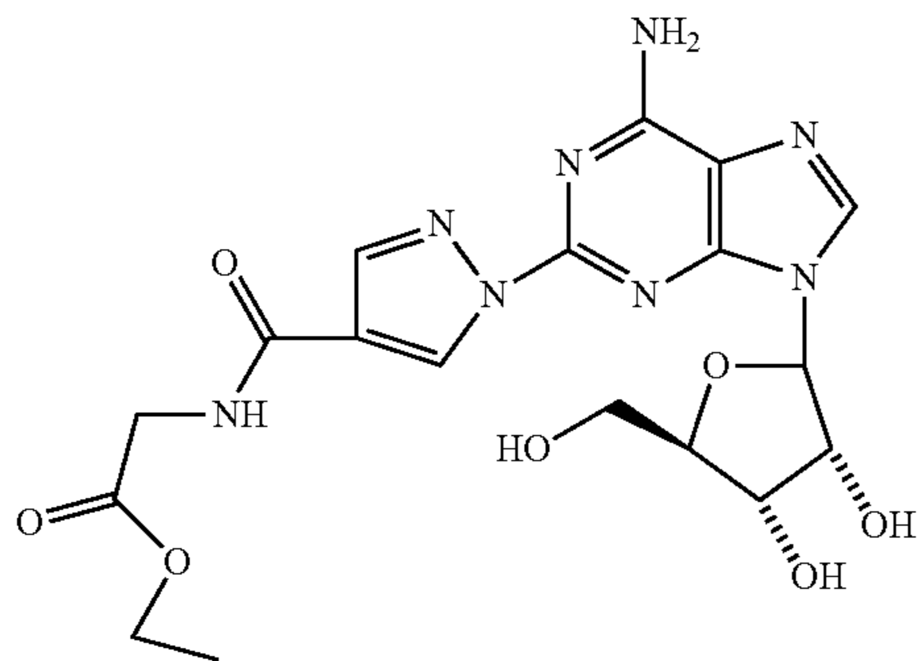
Ethyl 2-[(1-{9-[(4S,2R,3R,5R)-3,4-dihydroxy-5-(hydroxymethyl)oxolan-2-yl]-6-aminopurin-2-yl}pyrazol-4-yl)carbonylamino]acetate (23)
