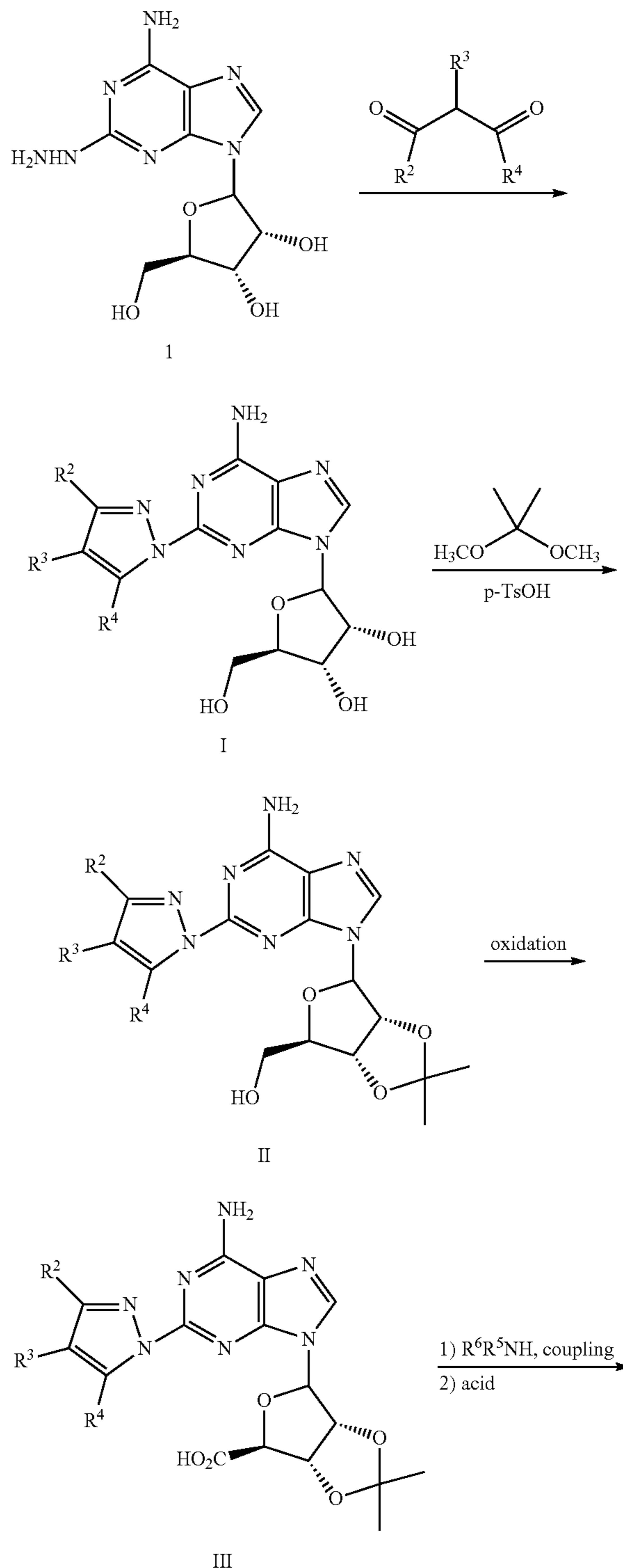
Scheme 1
