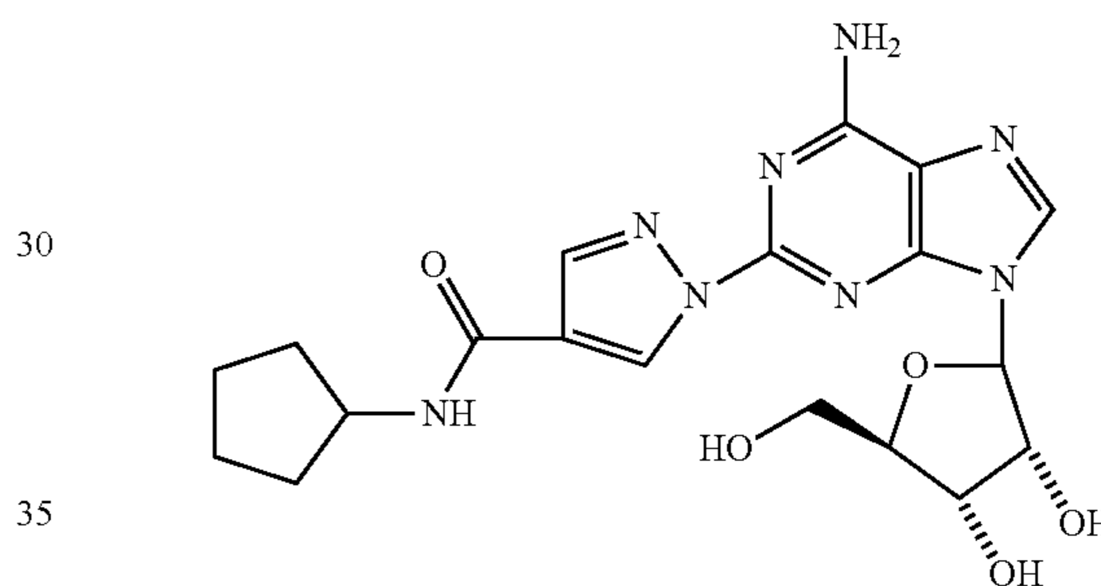
(1-{9-[(4S,2R,3R,5R)-3,4-dihydroxy-5-(hydroxymethyl)oxolan-2-yl]-6-aminopurin-2-yl}pyrazol-4-yl)-N-(cyclopentyl)carboxamide (21)
