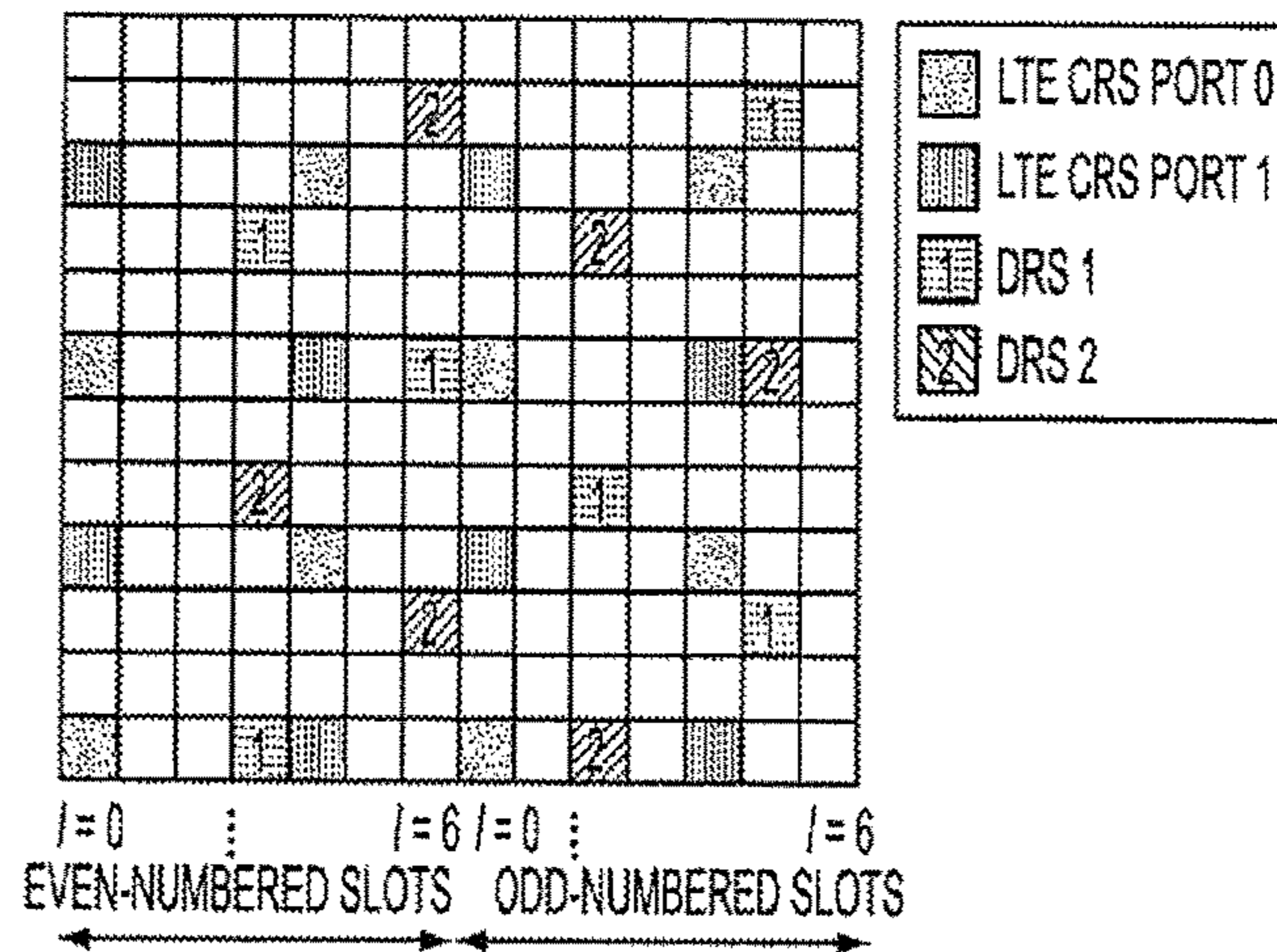
FIG. 5 RELATED ART
