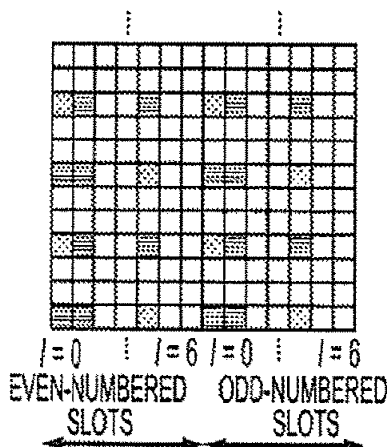
ANTENNA PORT 1 FIG. 2E RELATED ART
