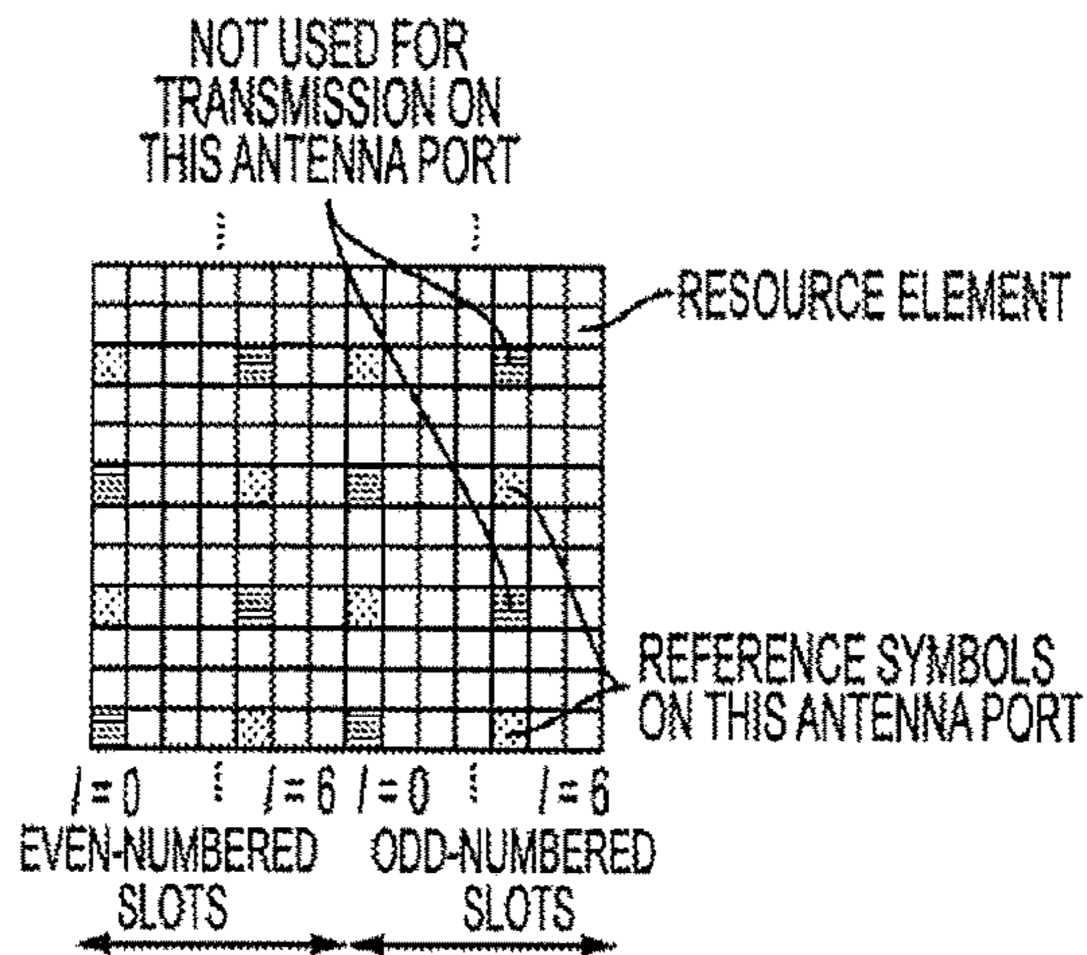
FIG. 2C RELATED ART
