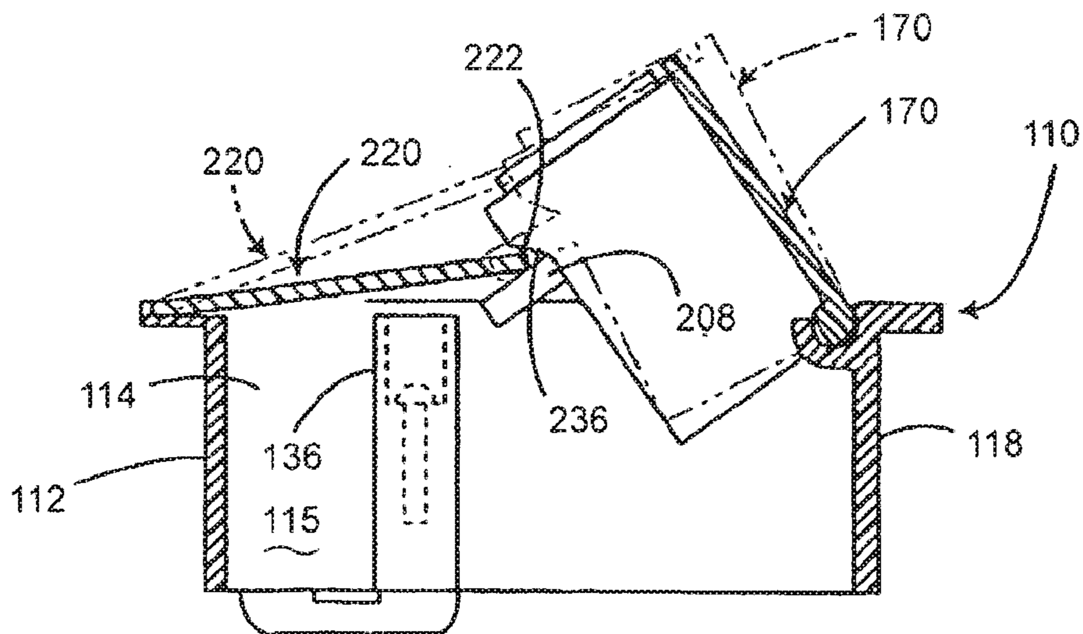
Fig. 15 (Prior Art)
