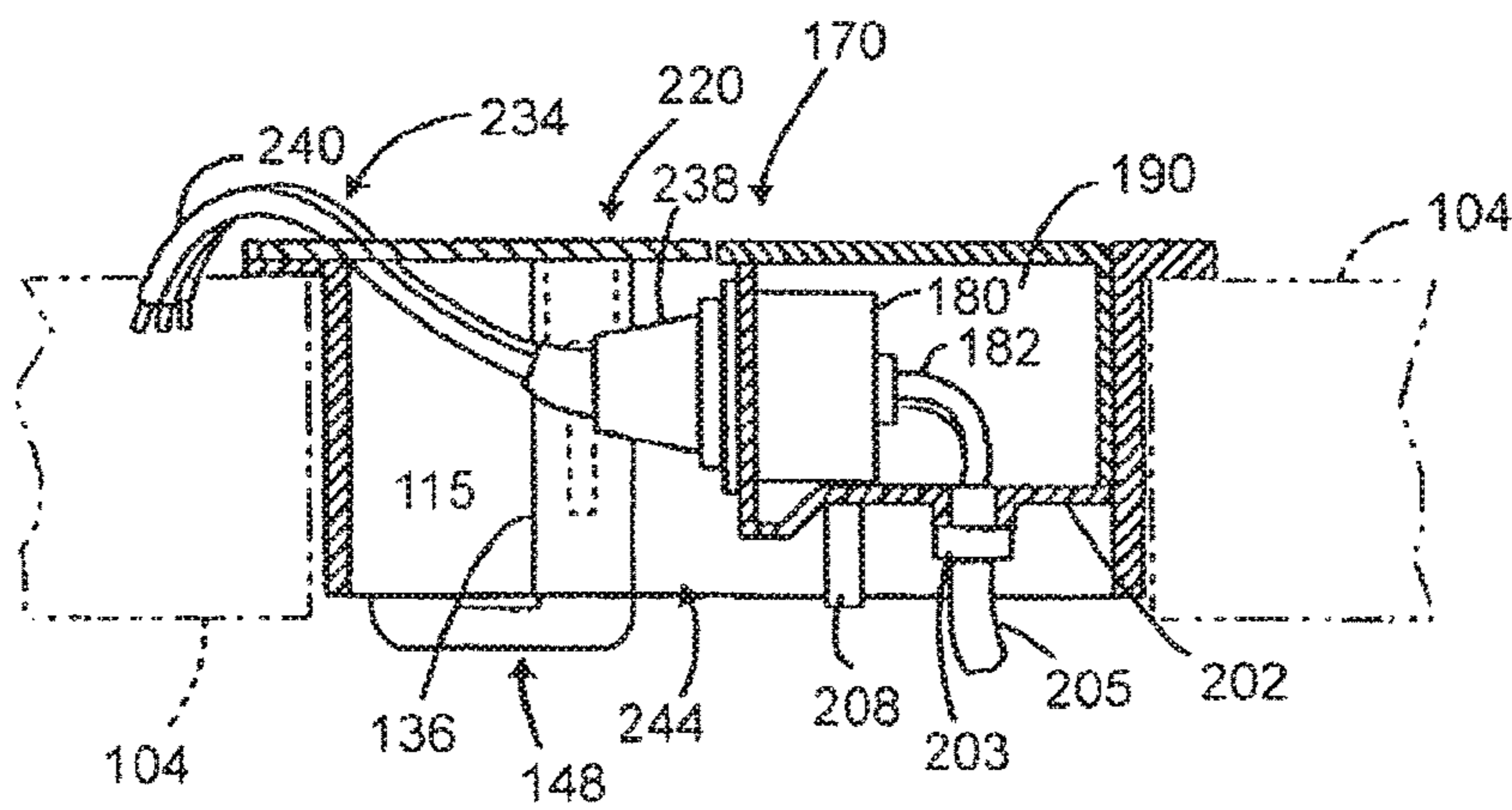
Fig. 13 (Prior Art)
