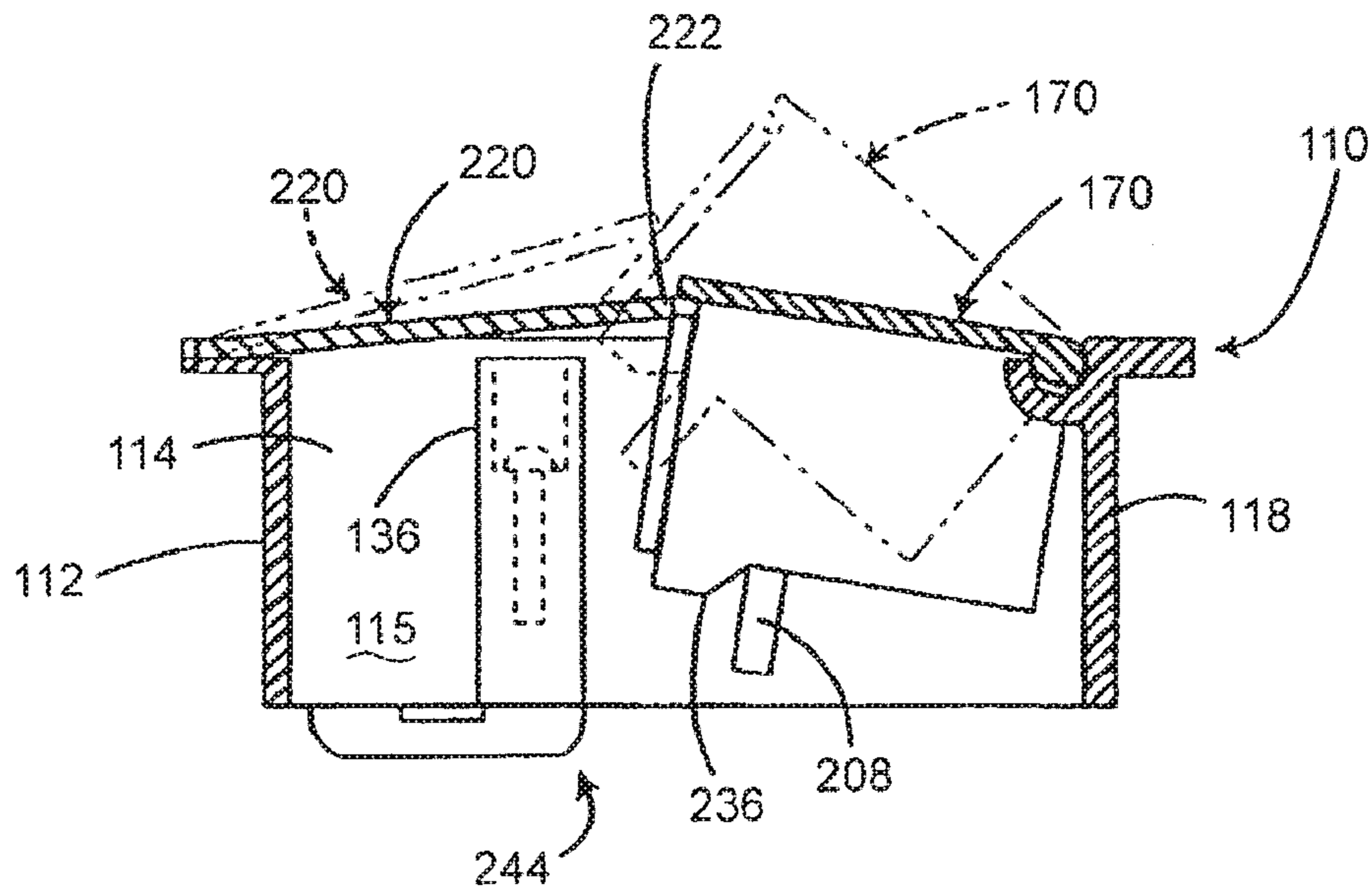
Fig. 15 (Prior Art)
