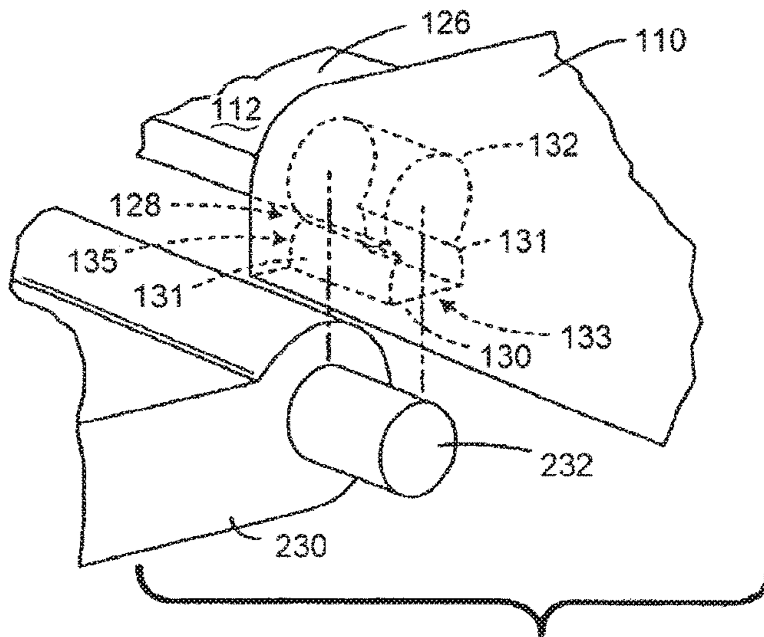
Fig. 10 (Prior Art)
