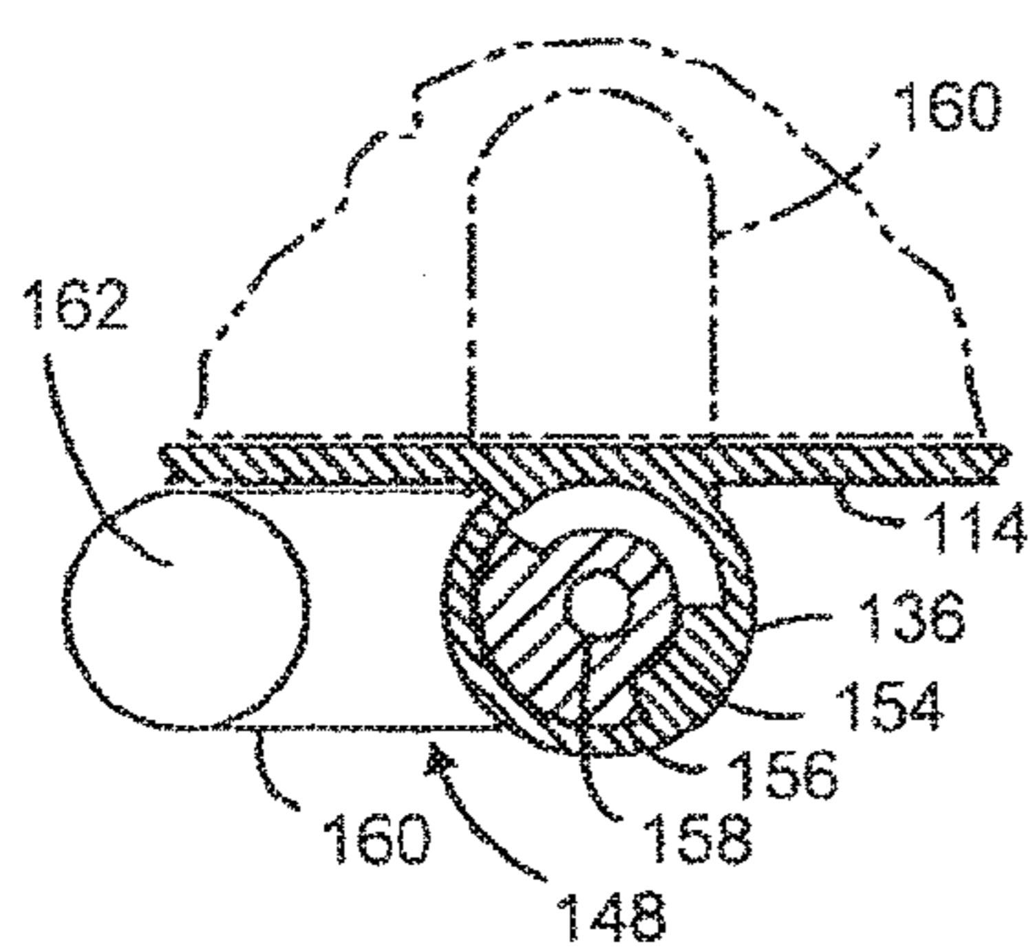
Fig. 8 (Prior Art)
