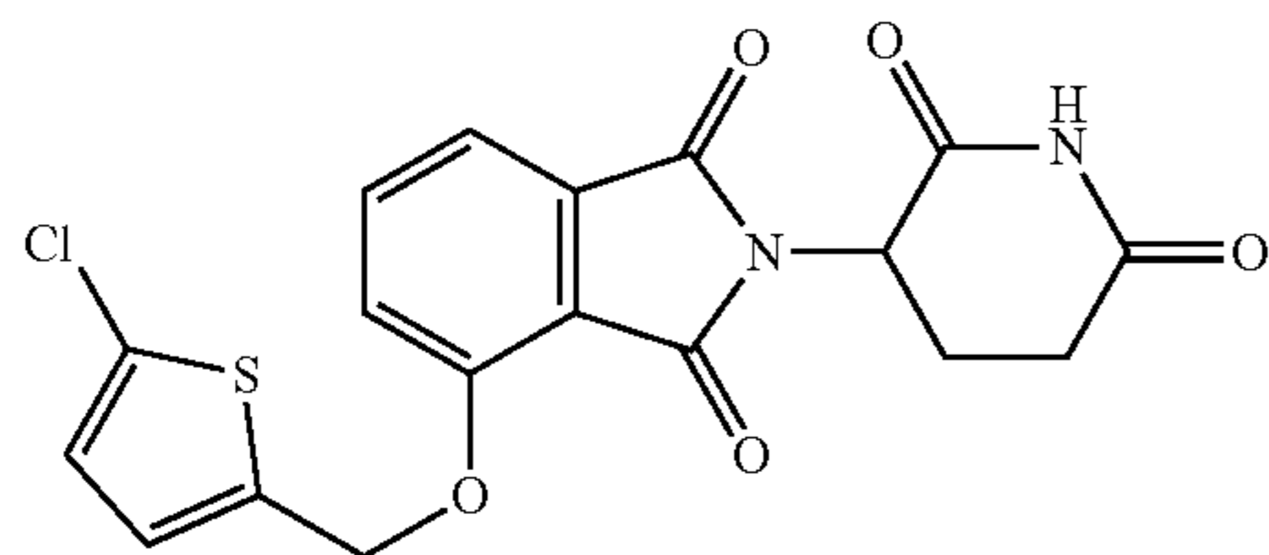
1-(5-Chloro-thiophen-2-ylmethoxy)-2-(2,6-dioxo-piperidin-3-yl)-isoindole-1,3-dione
