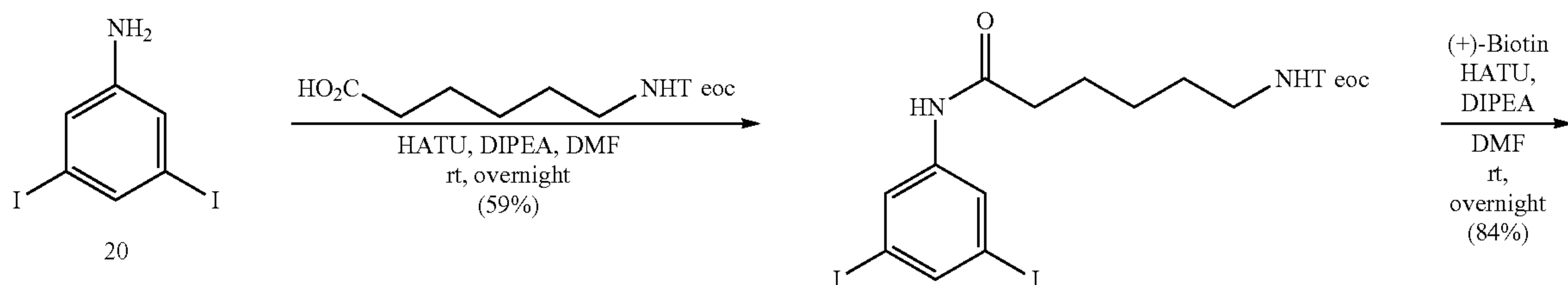
Scheme 7
