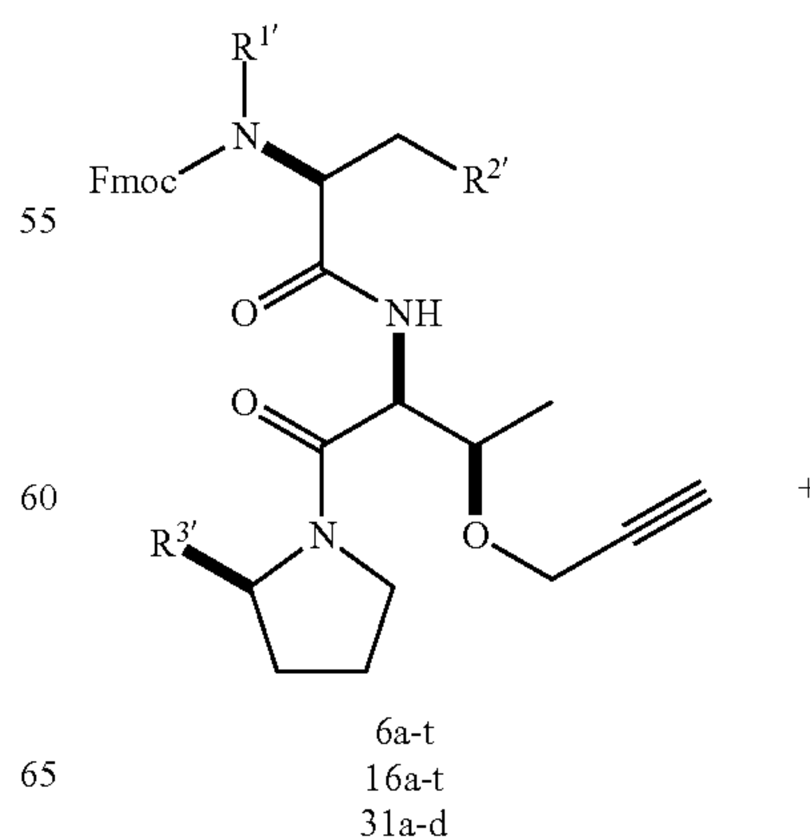
Scheme 12
