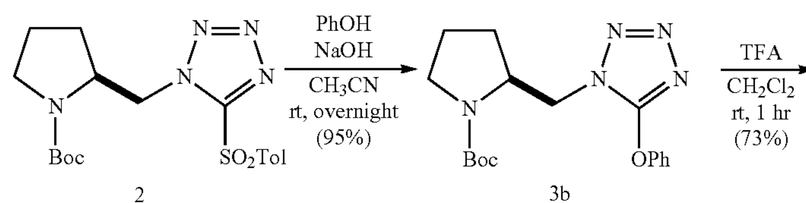
Scheme 2
