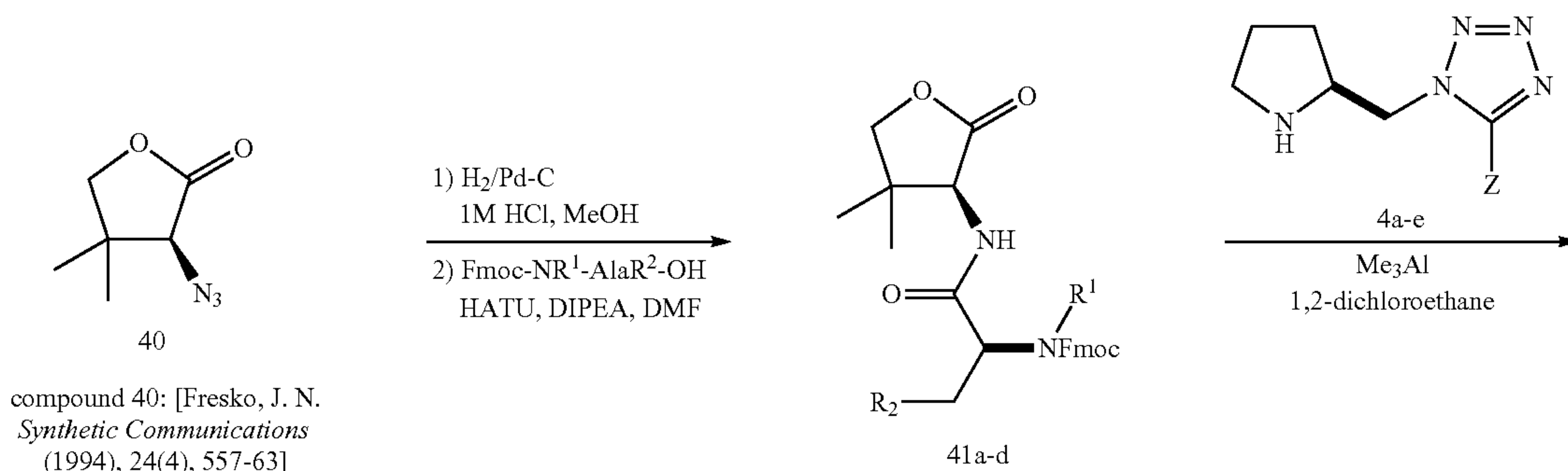
Scheme 14
