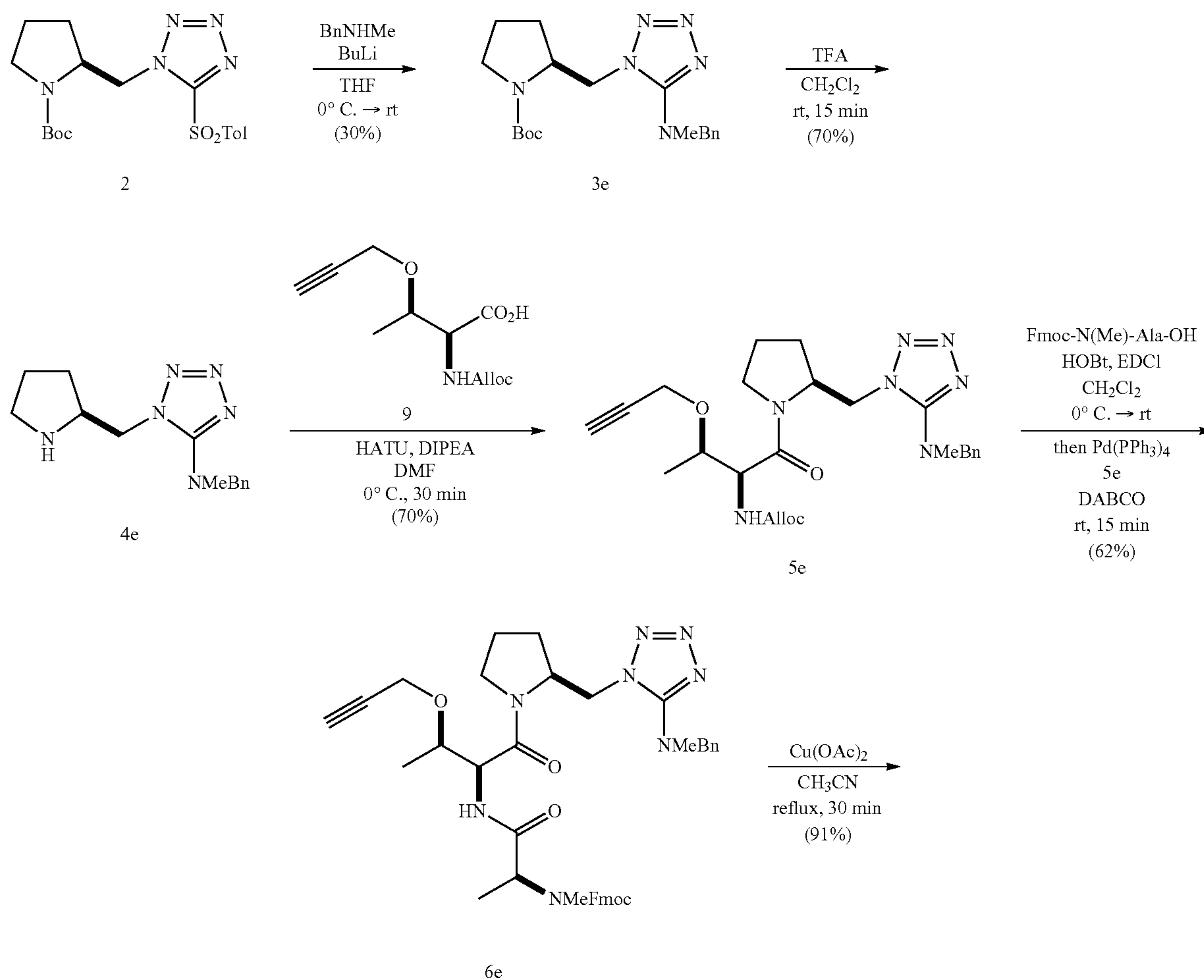
Scheme 5
