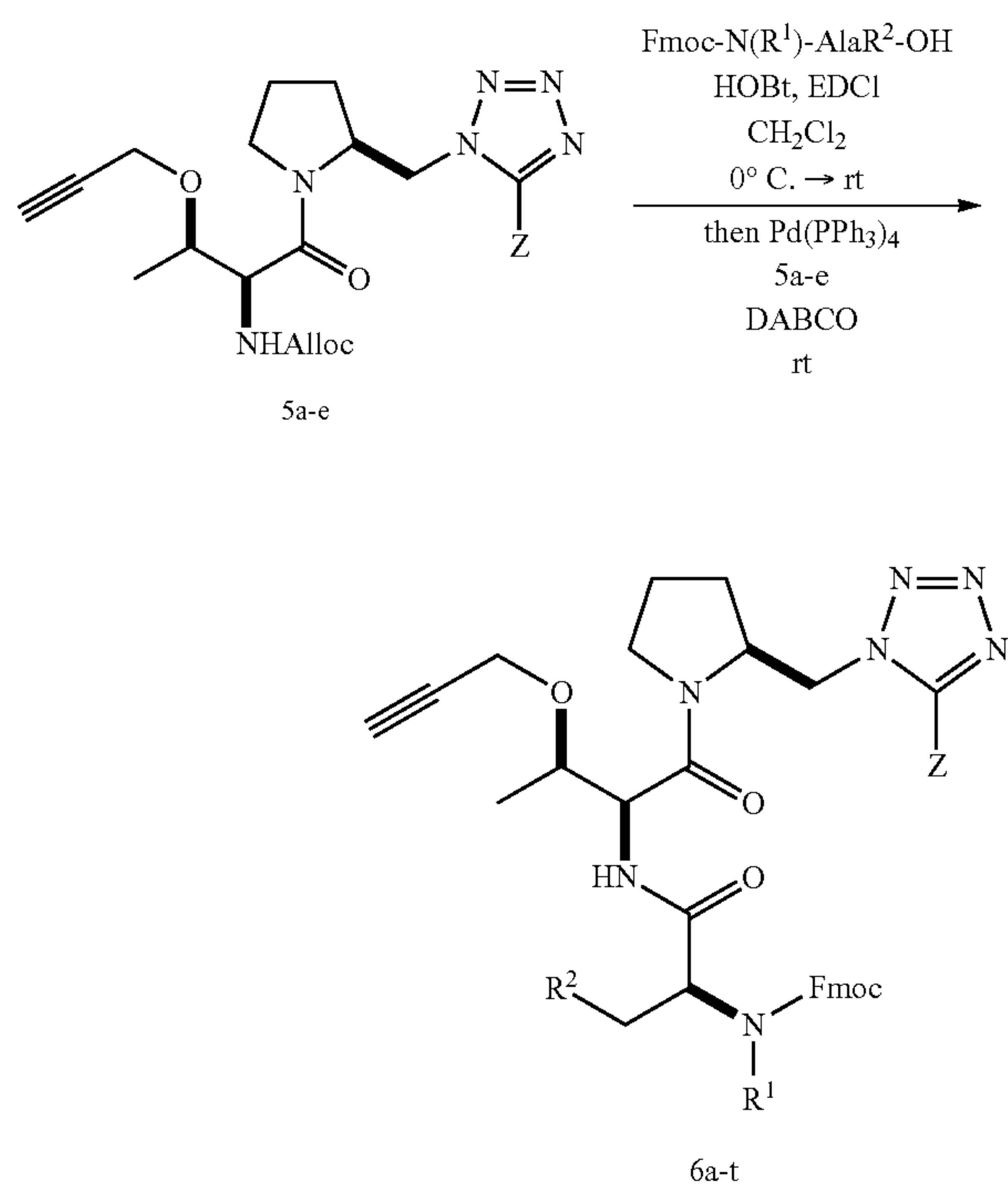
Scheme 9
