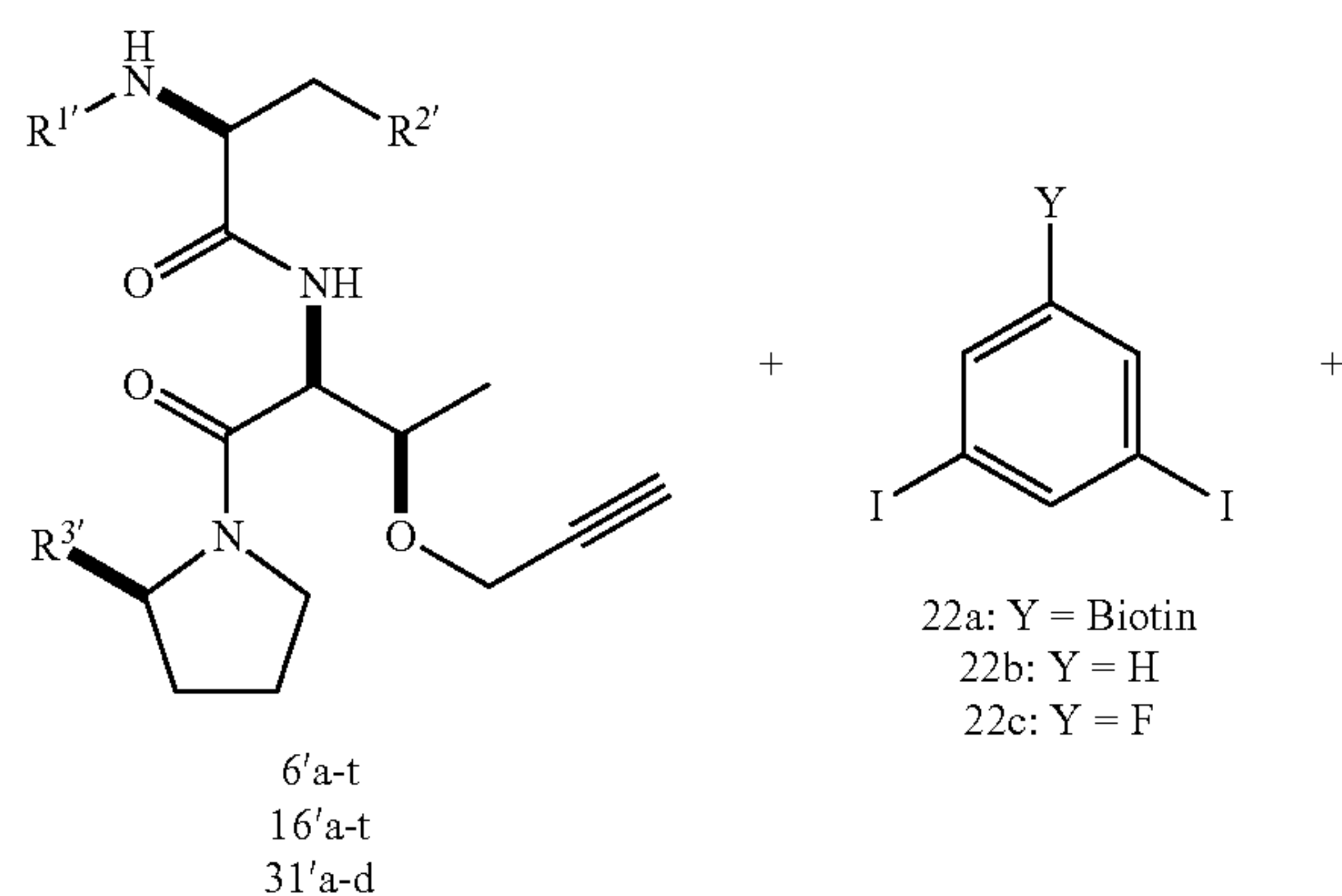
Scheme 13
