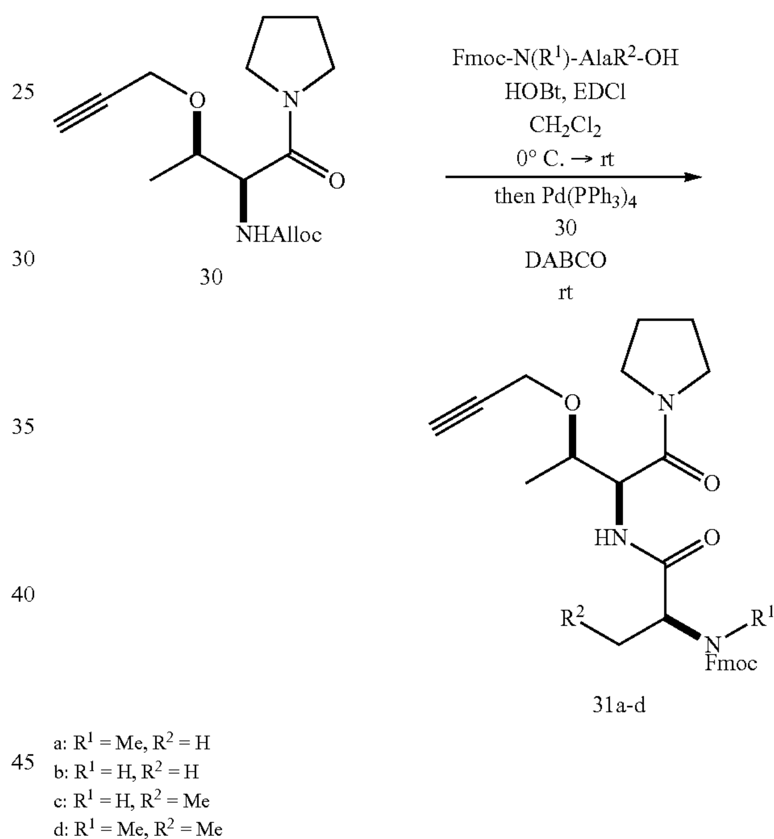
Scheme 11
