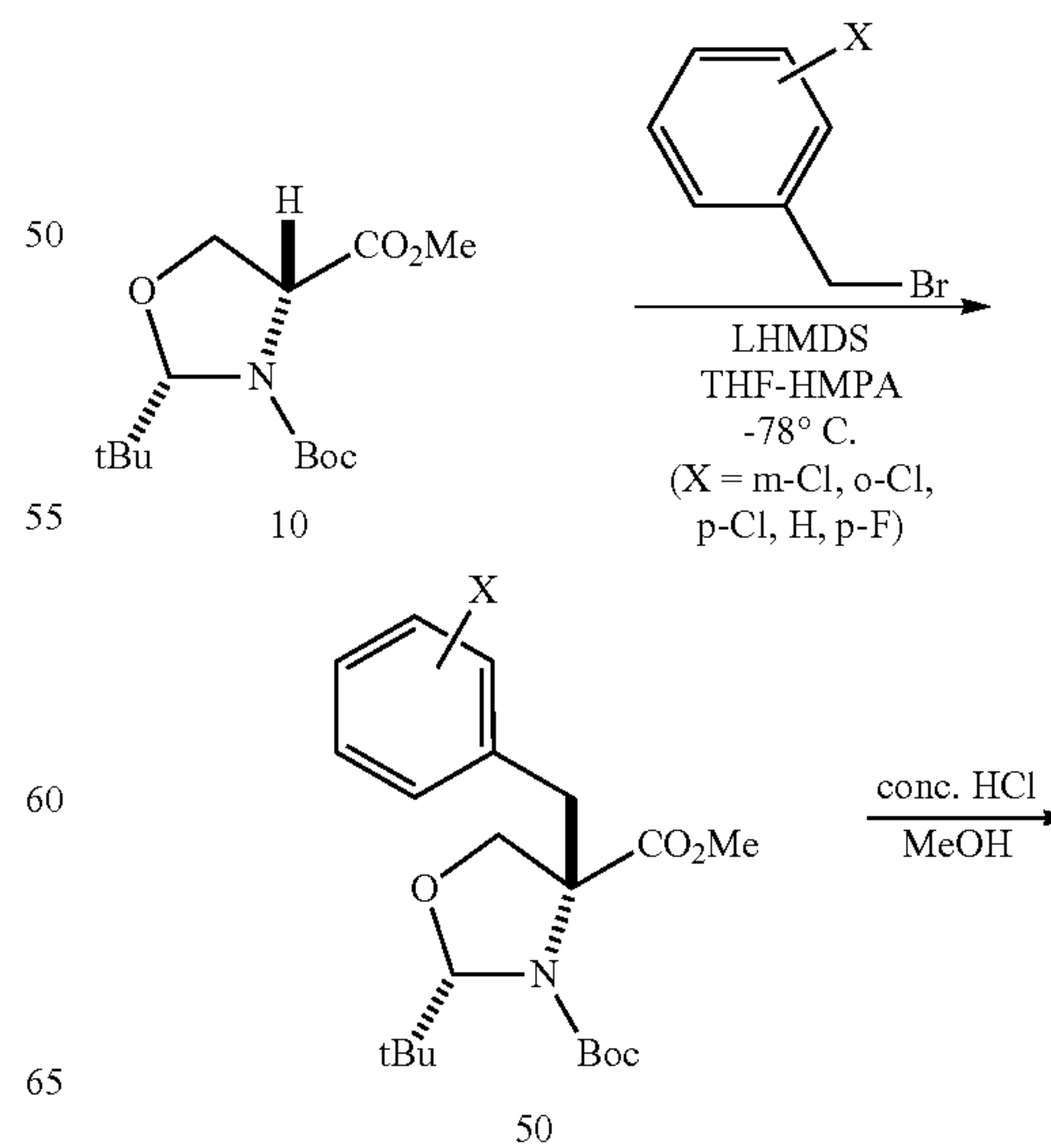
Scheme 10
