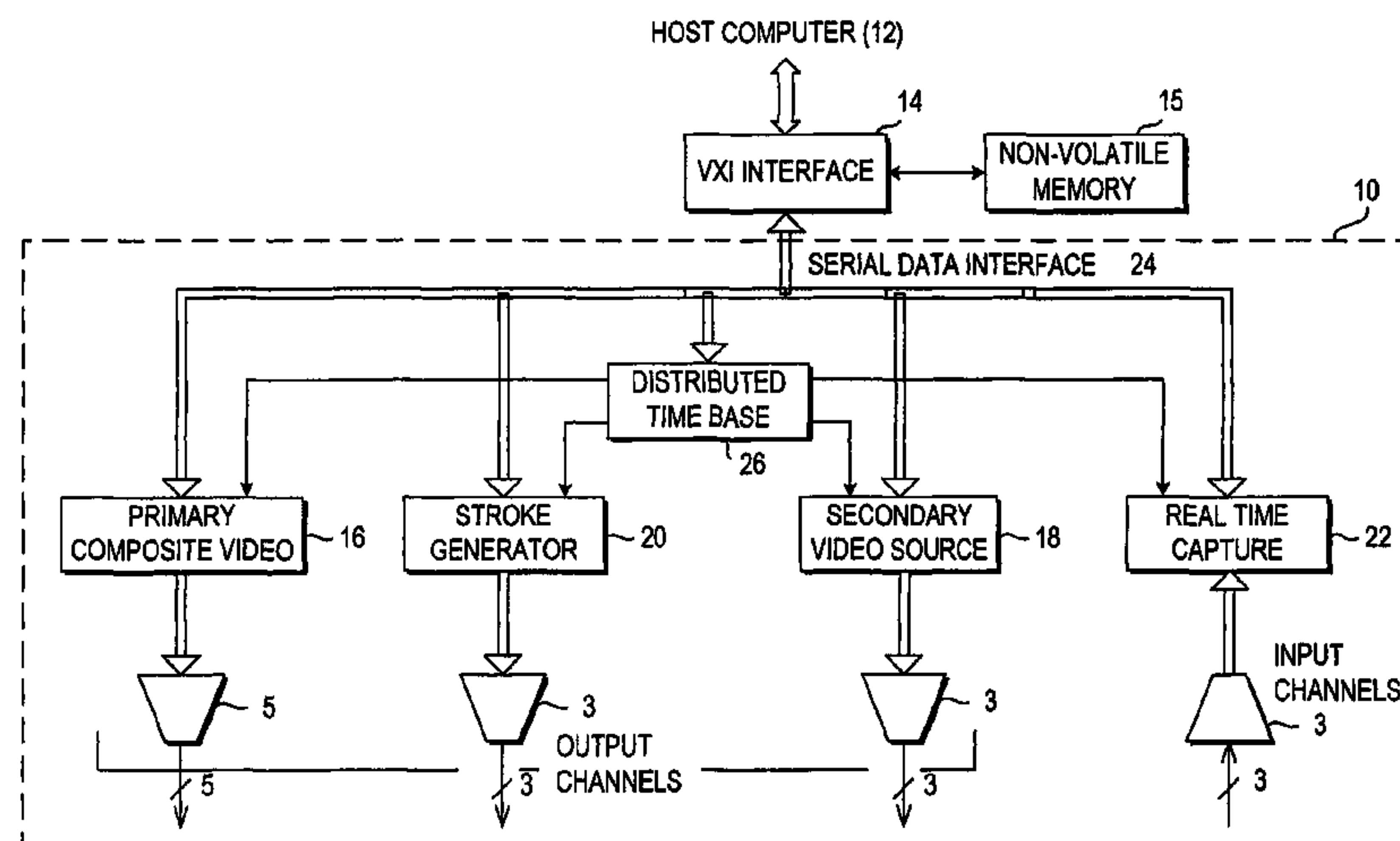
GENERAL ARRANGEMENT
