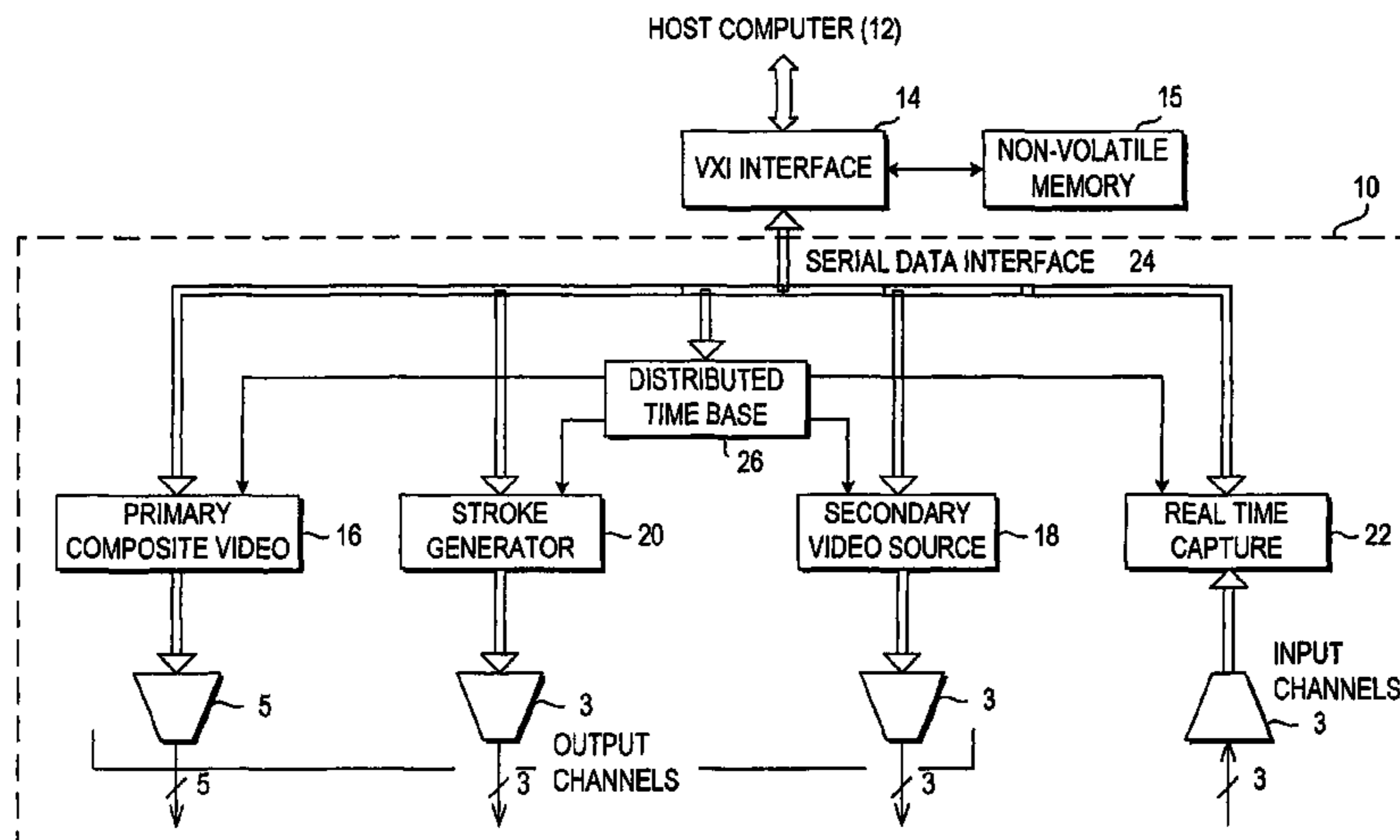
GENERAL ARRANGEMENT
