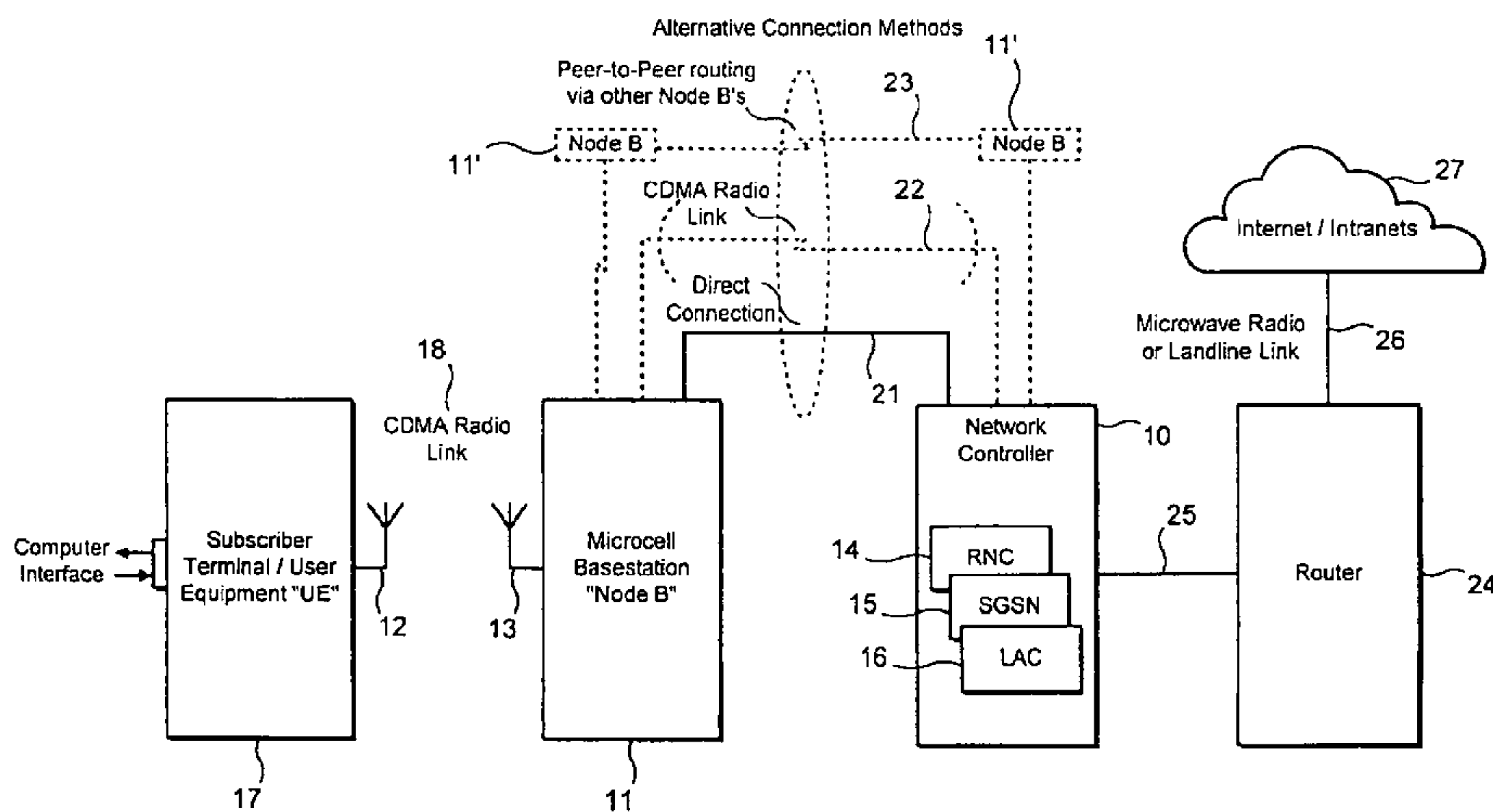
System Architecture
