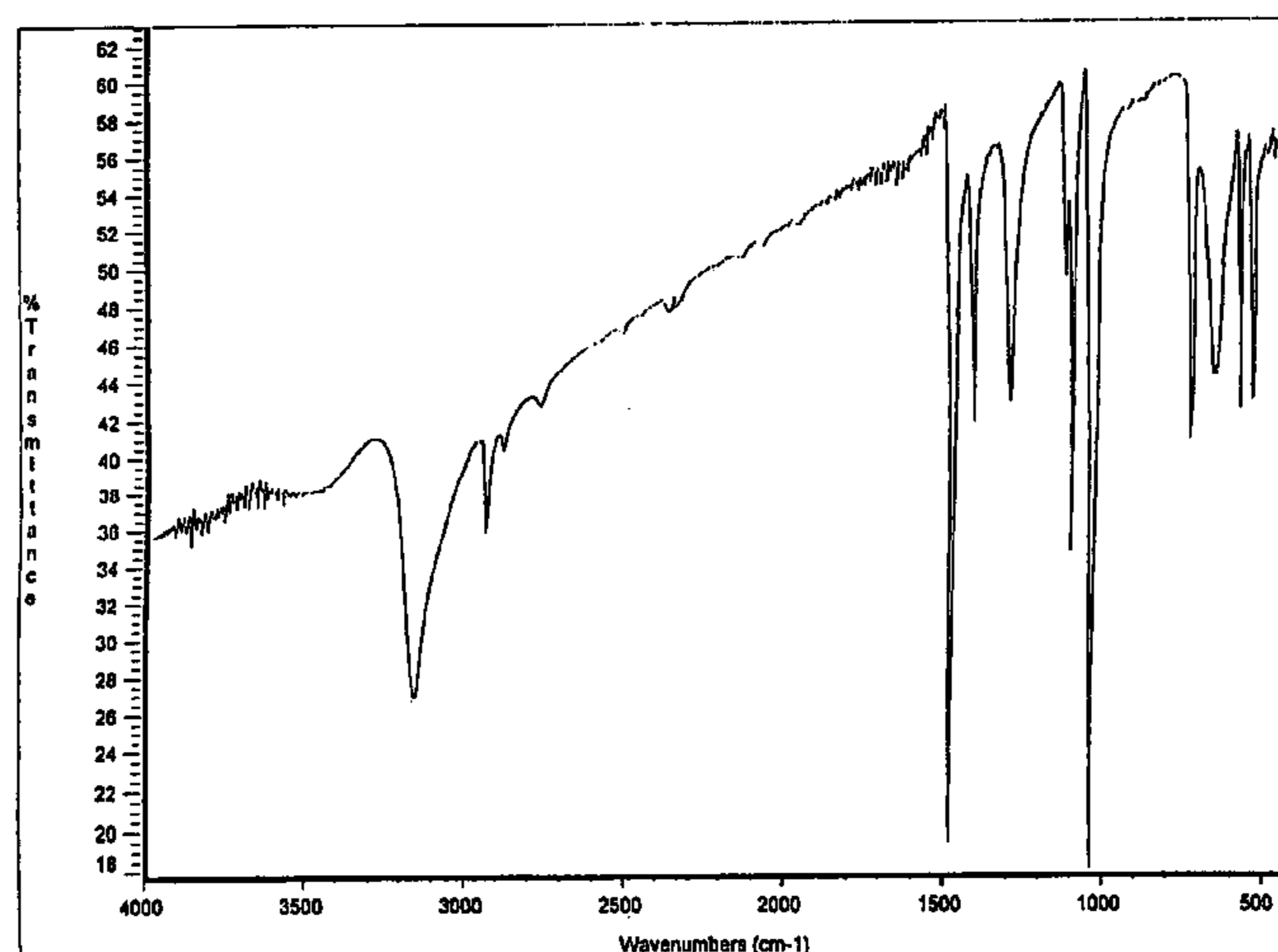
IR Spectrum of Zn-DMTD, 1:2, according to Example 1.
