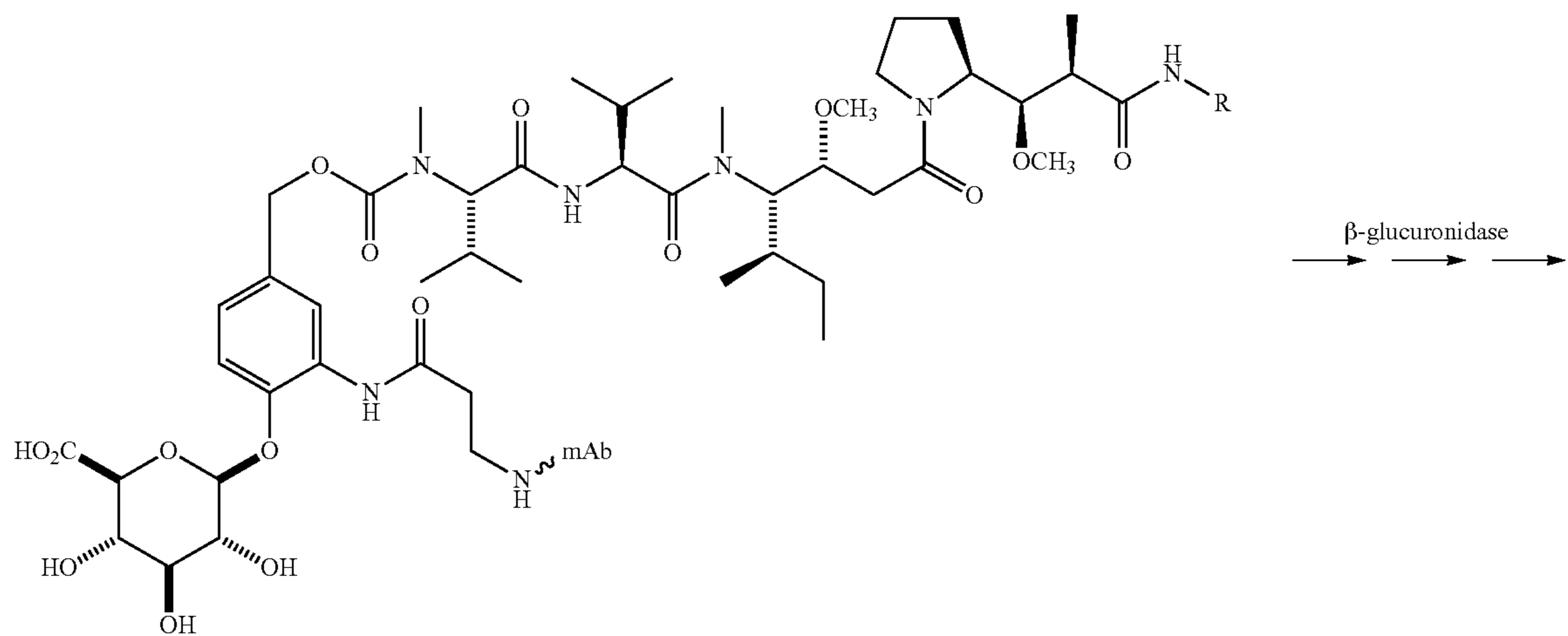
Scheme 2.
