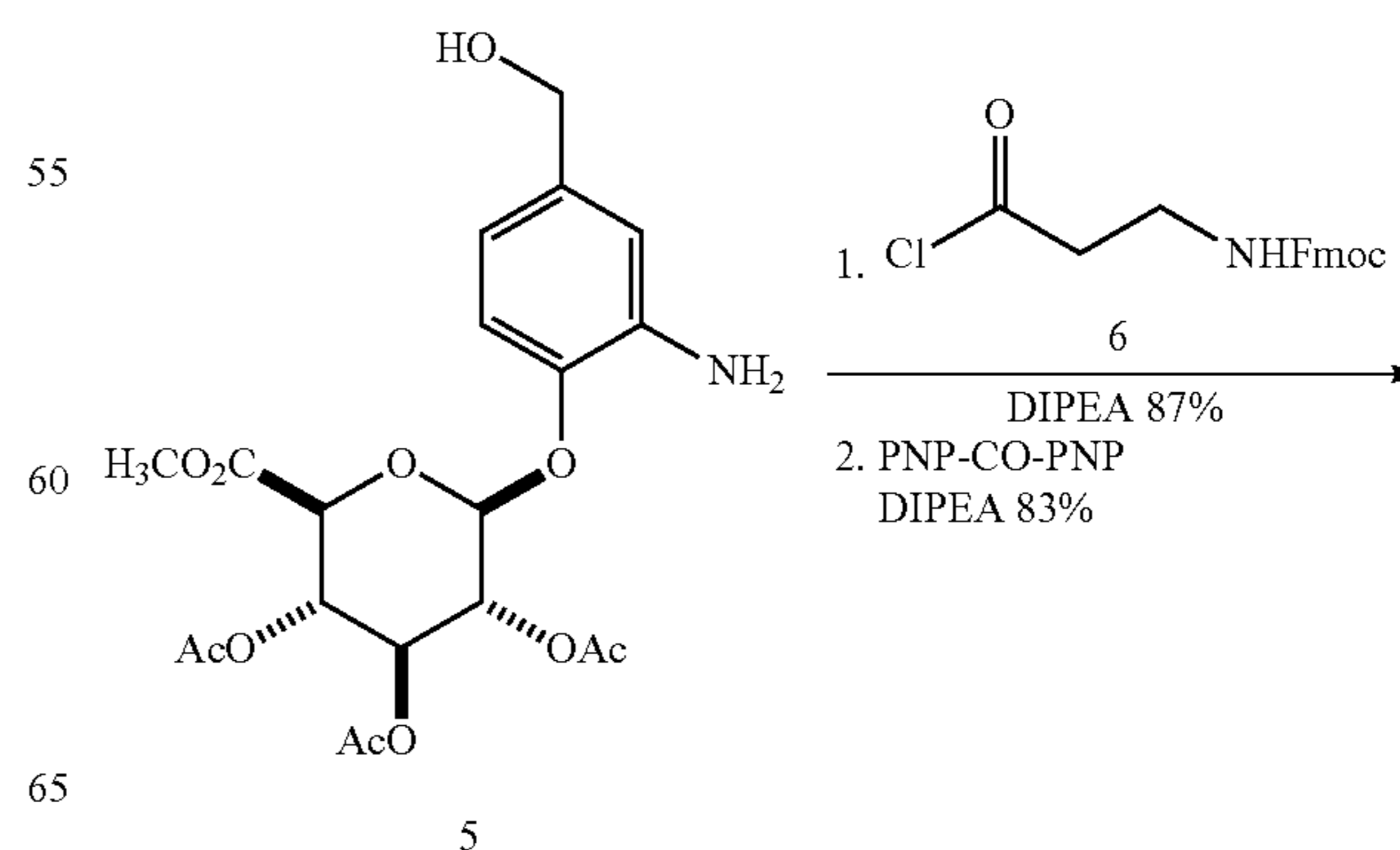
Scheme 3
