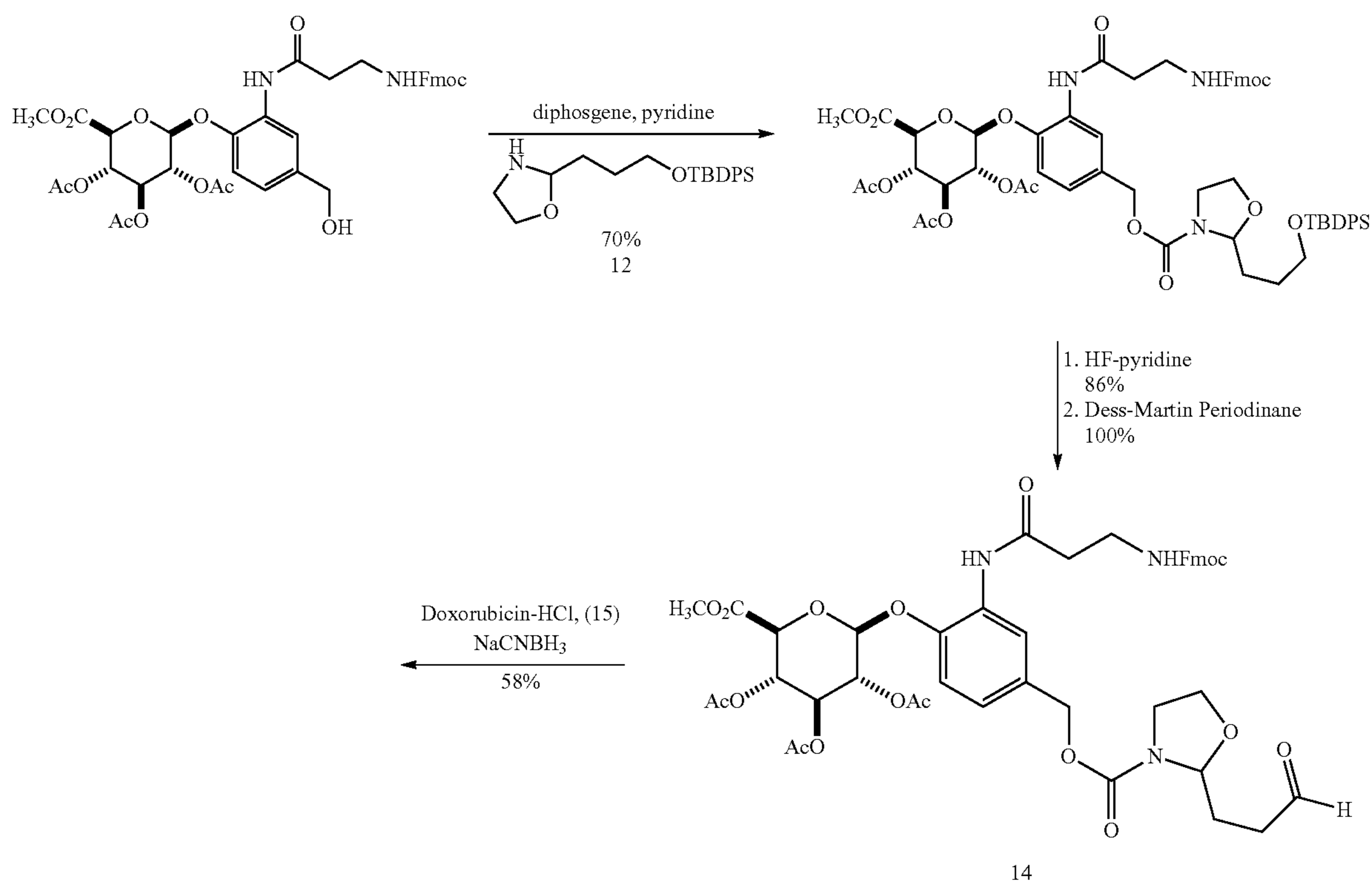
Scheme 4
