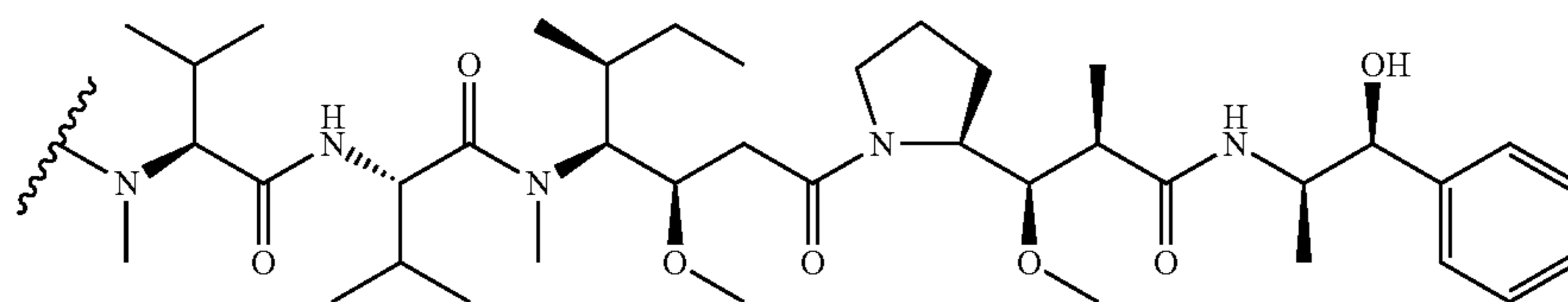
MMAE
