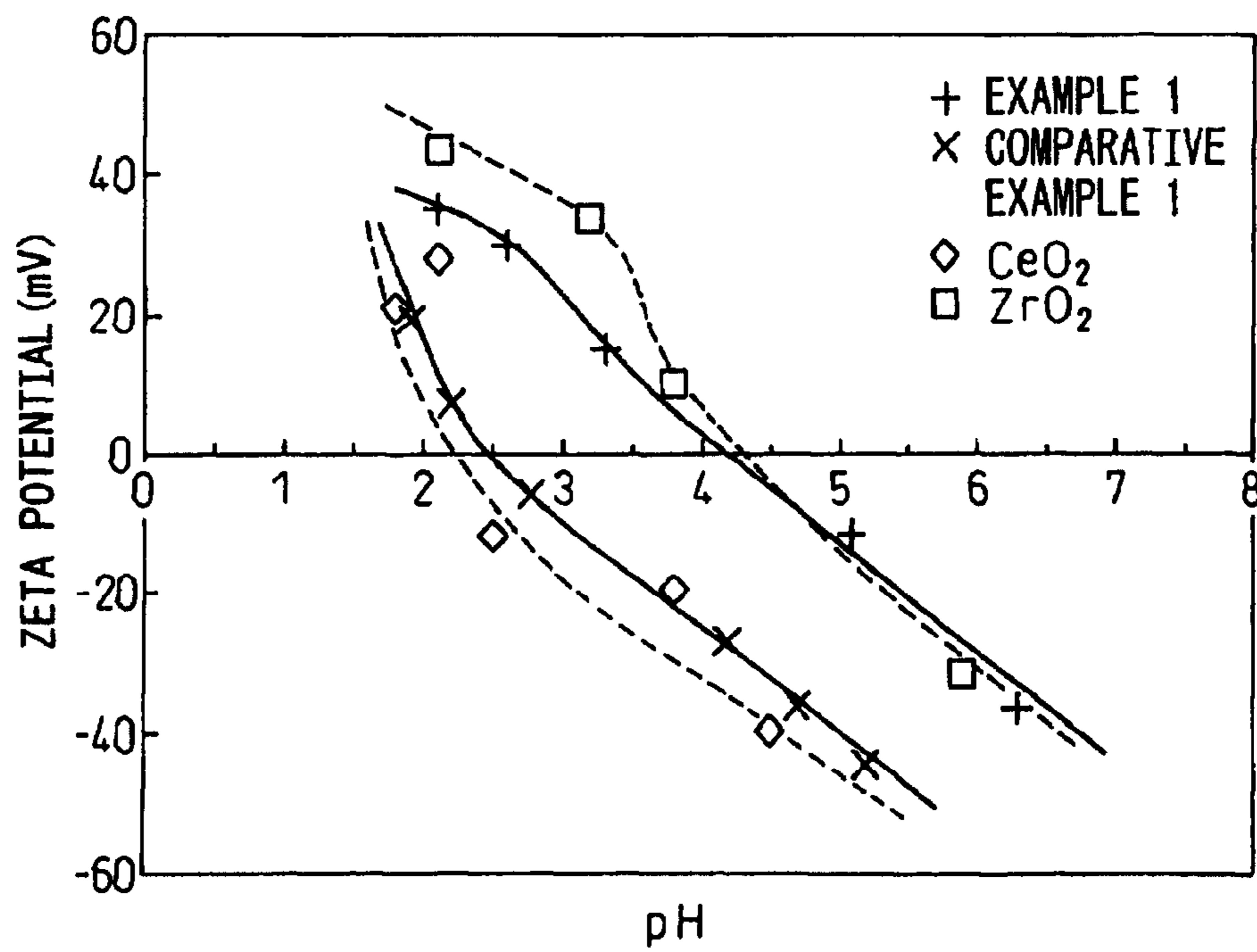
RELATIONSHIP BETWEEN pH AND ZETA POTENTIAL
