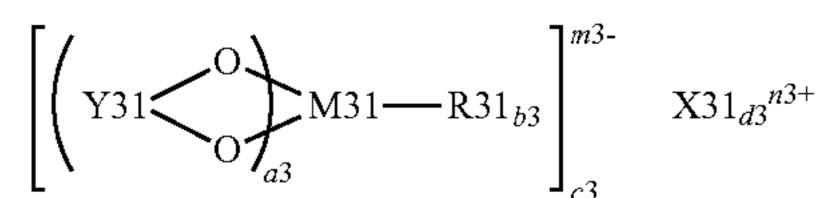
Chemical formula 4
