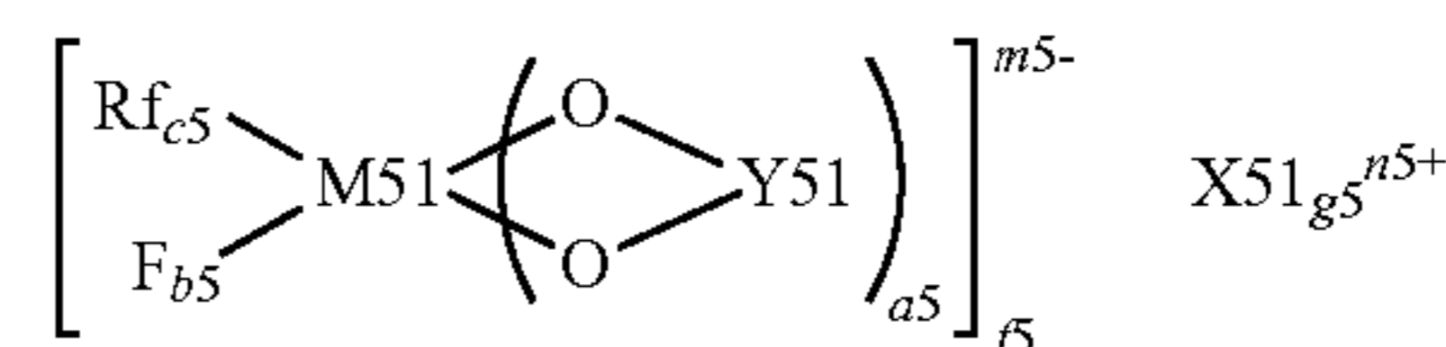
Chemical formula 10
