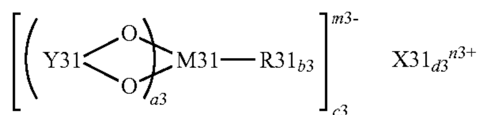
Chemical formula 8
