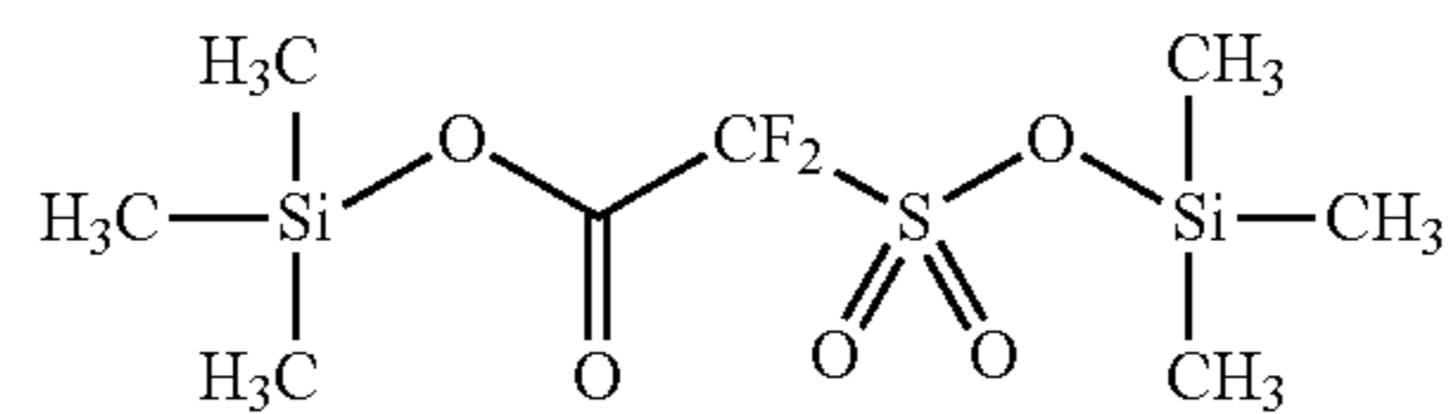
Chemical formula 2
