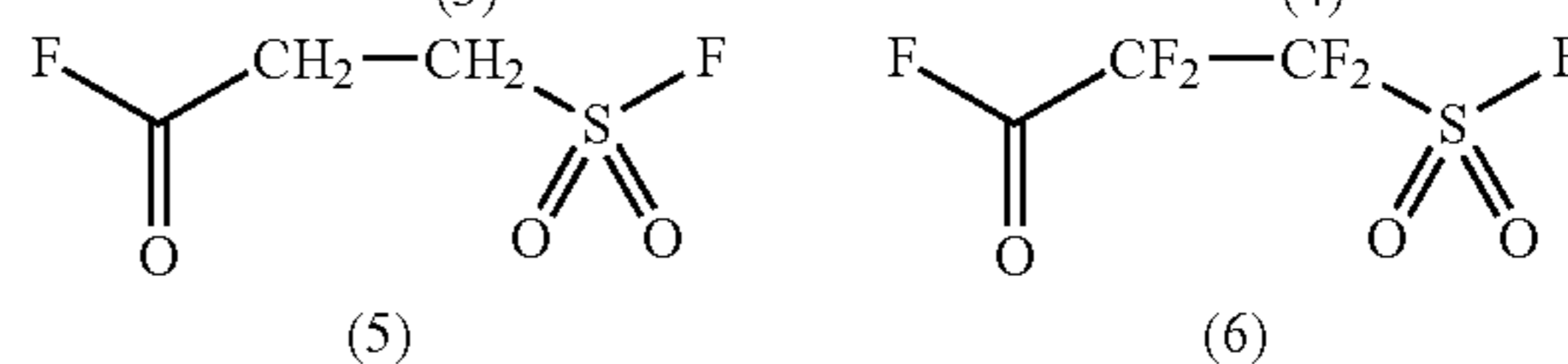
Chemical formula 3
