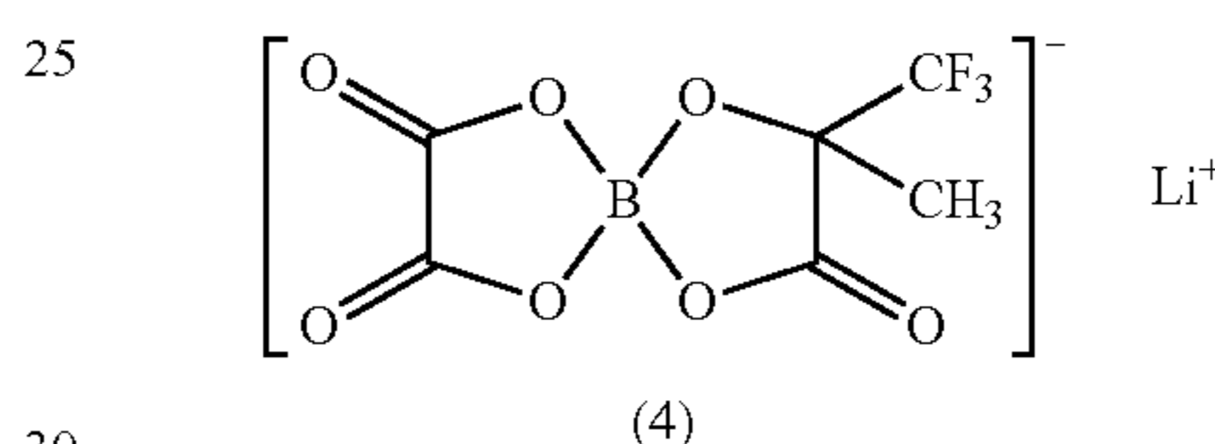
Chemical formula 18
