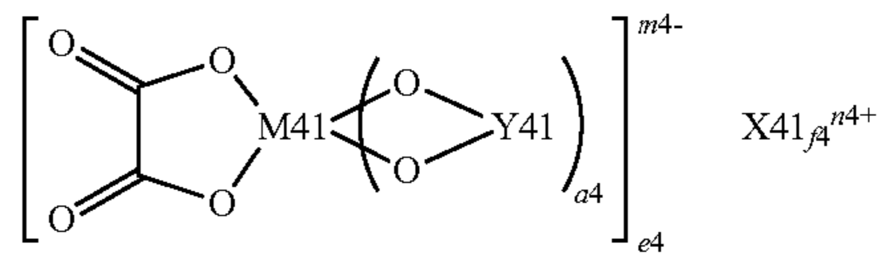
Chemical formula 9
