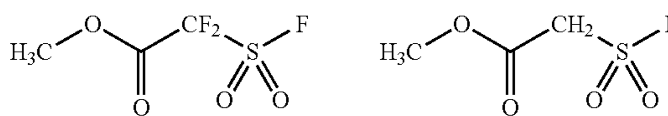
Chemical formula 3
