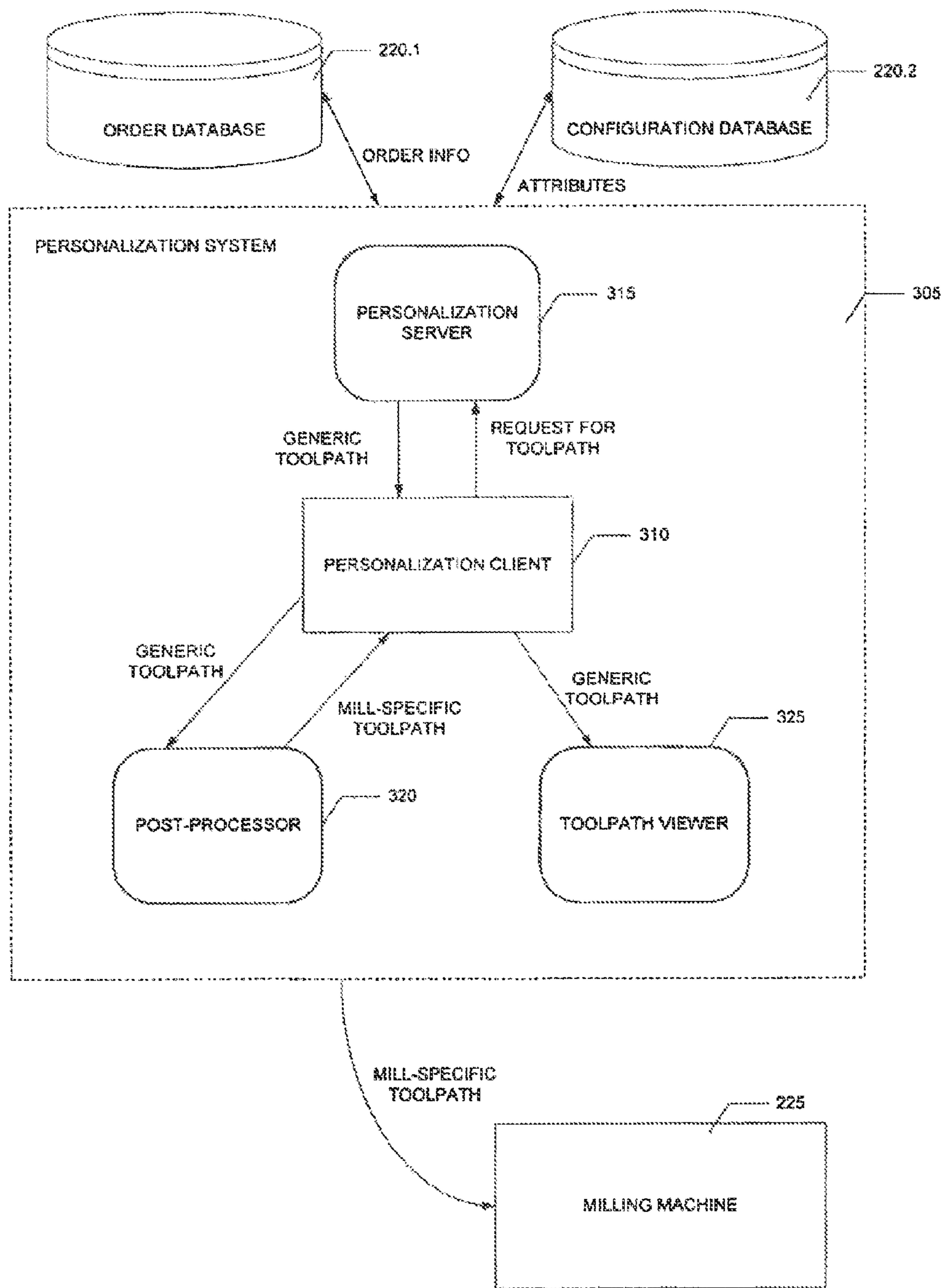
FIG. 3 SYSTEM ARCHITECTURE
