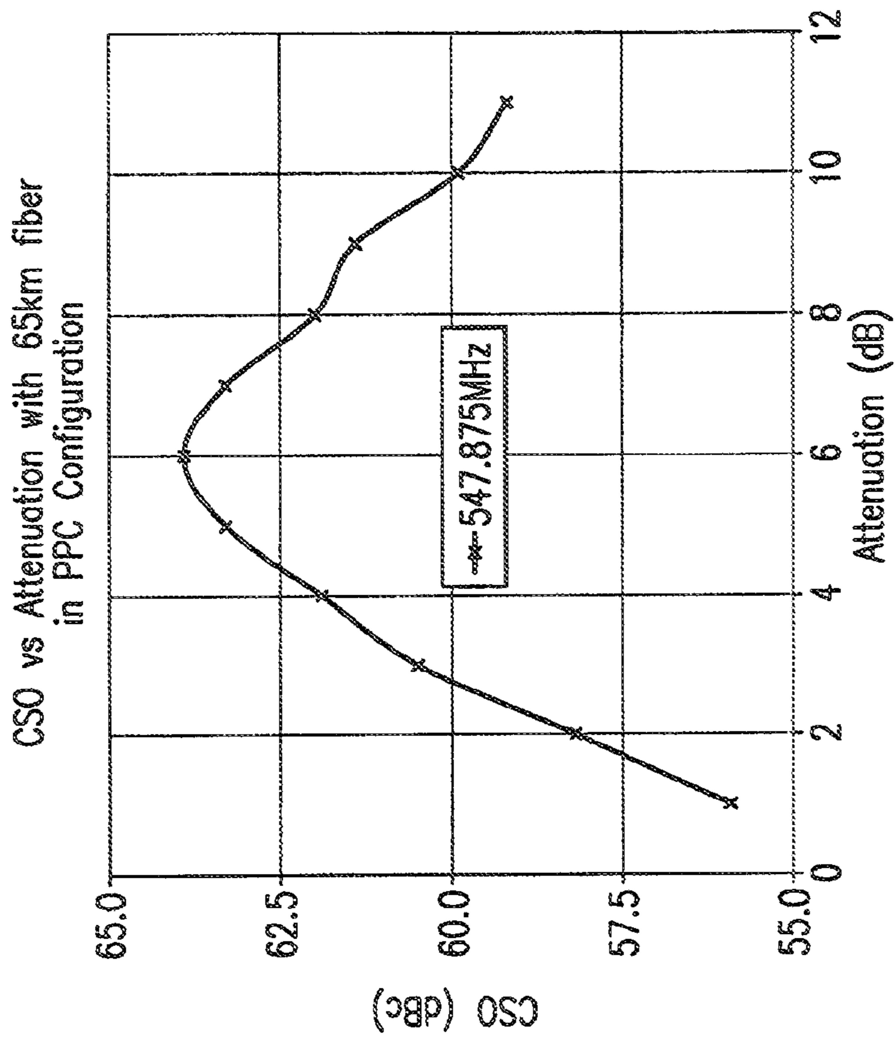
Test Condition: CSO was tested with 72 NTSC Channels from 115.25MHz to 547.875MHz over 65km SMF-28 fiber at 17dBm optical launching power and 0dBm receiving power
