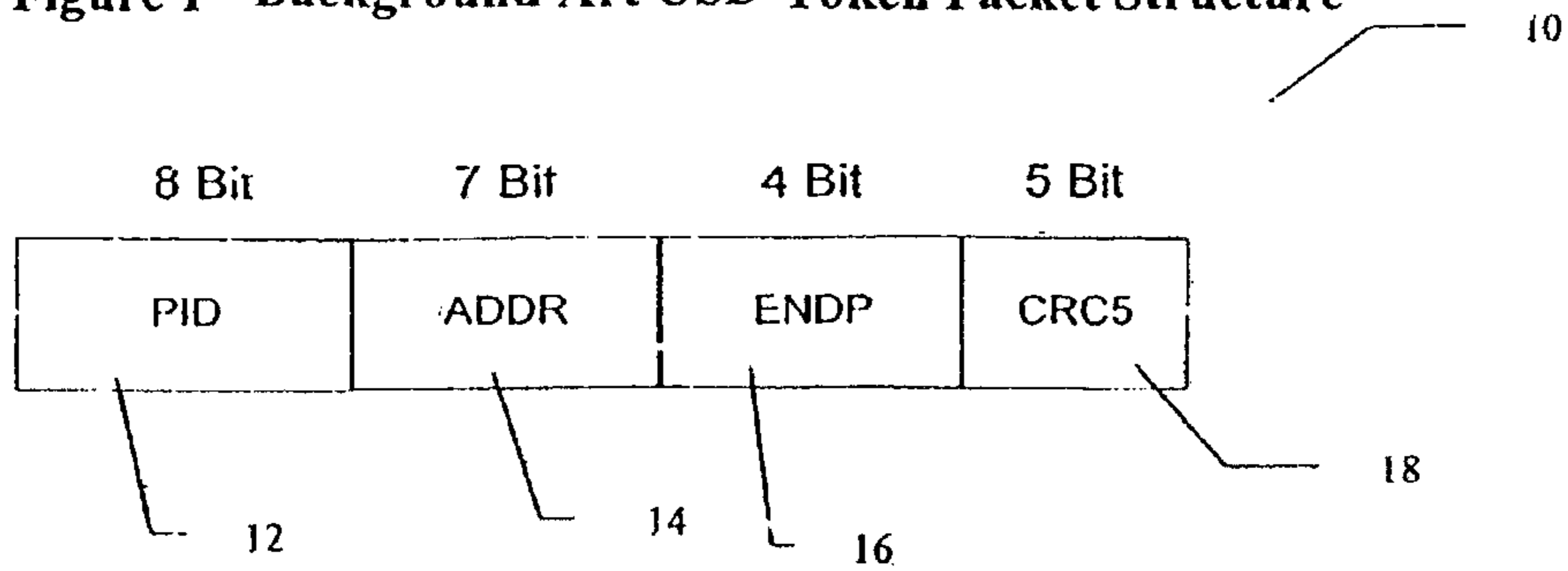
Figure 1-- Background Art USB Token Packet Structure
