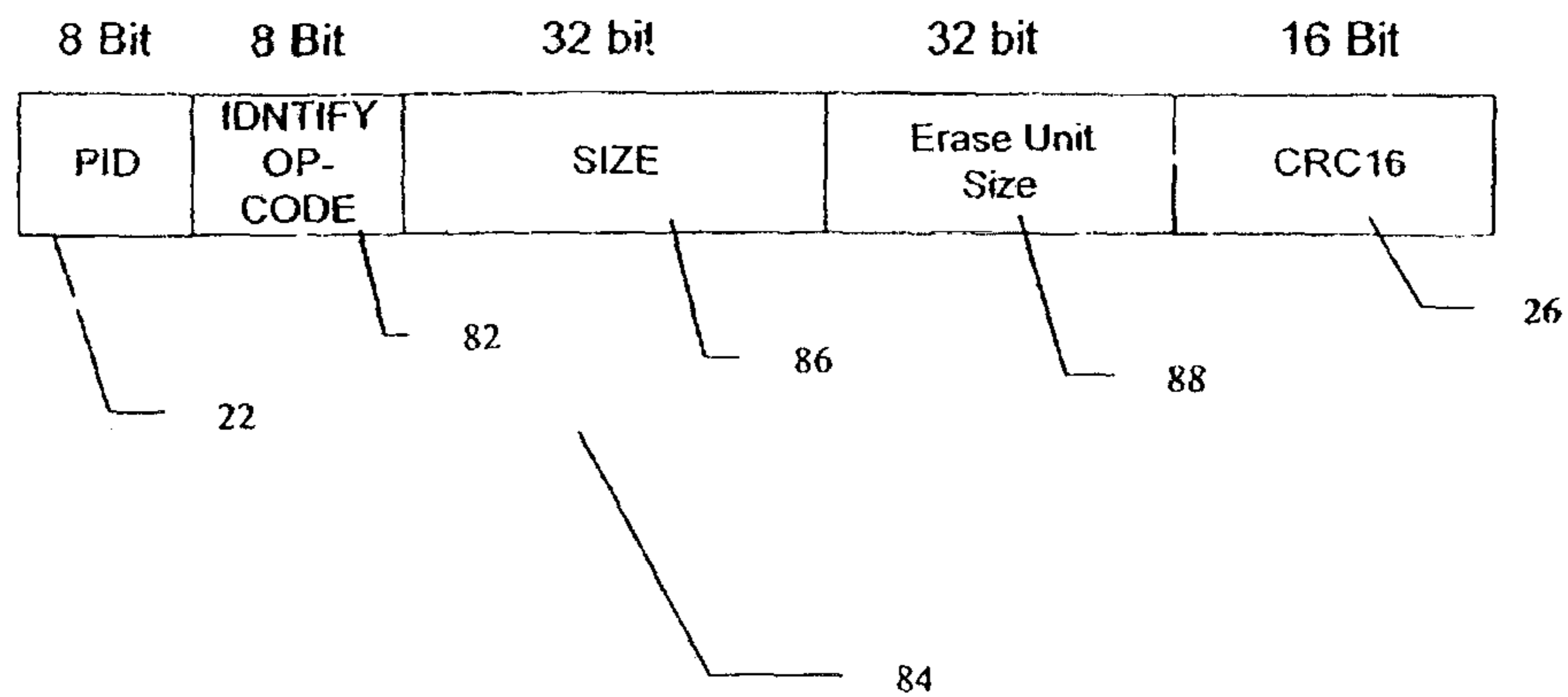
Fig 8 – Flash Identification Replay Packet
