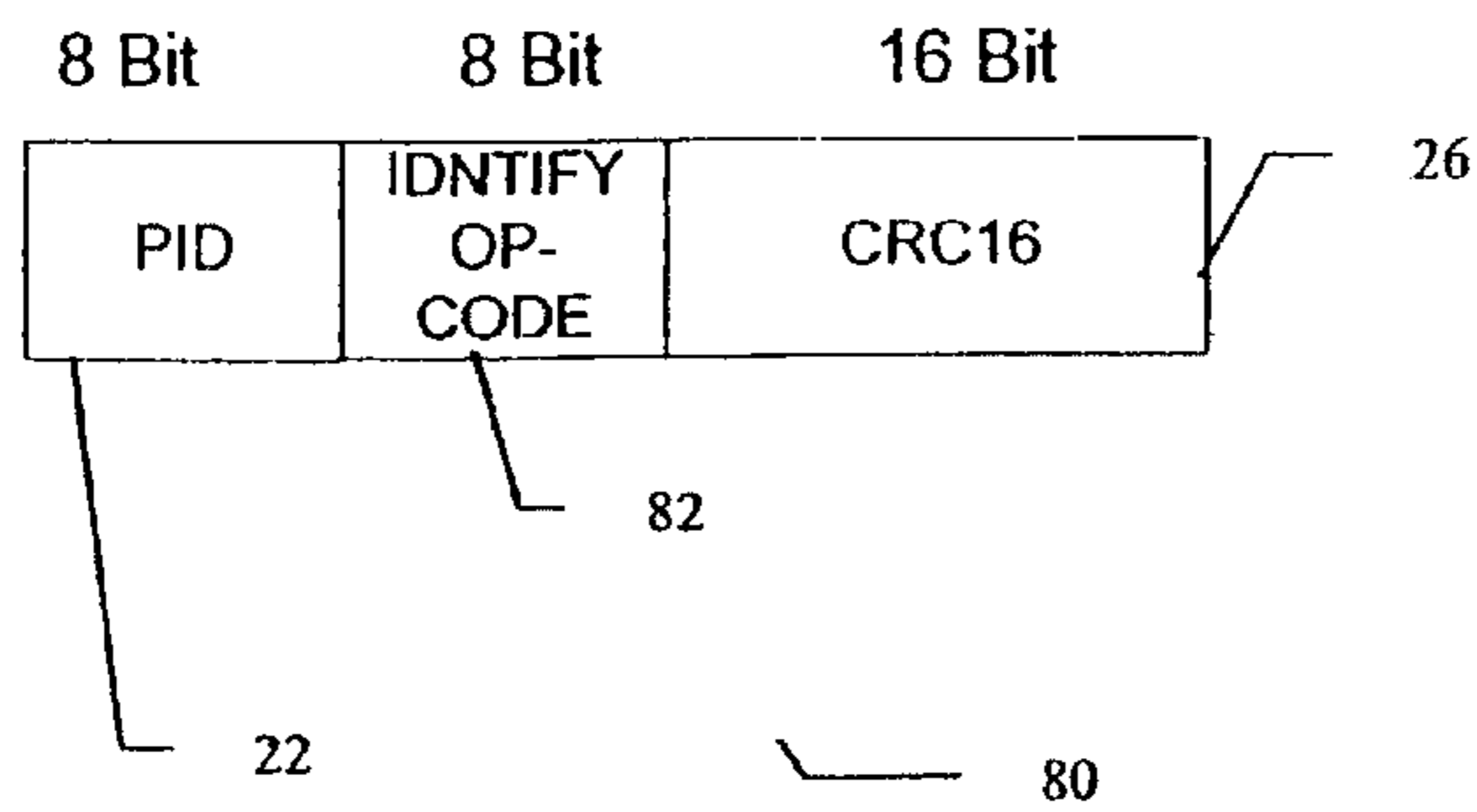
Fig 7 – Flash Identification Request Packet
