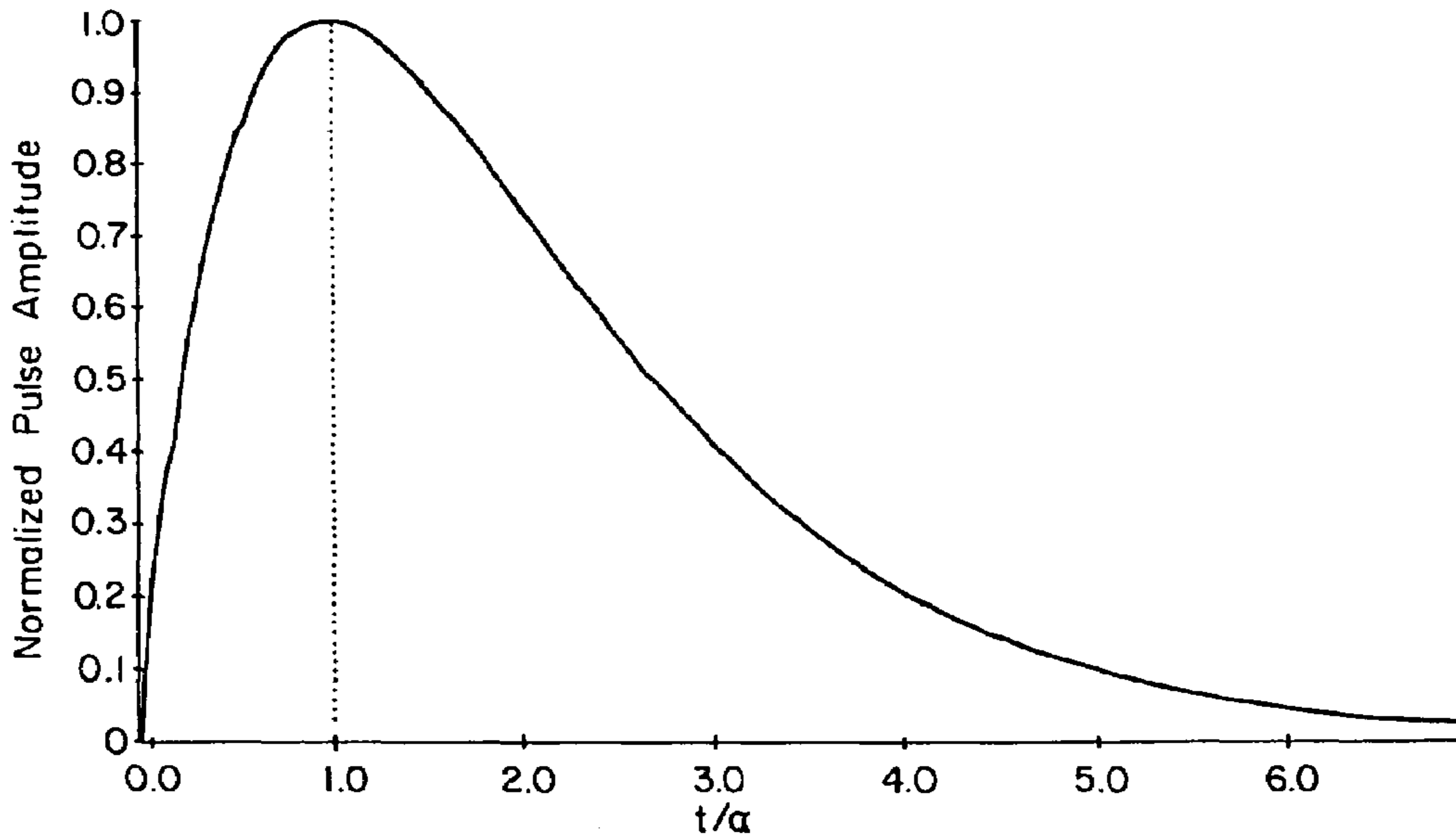
FIG. 10 PRIOR ART
