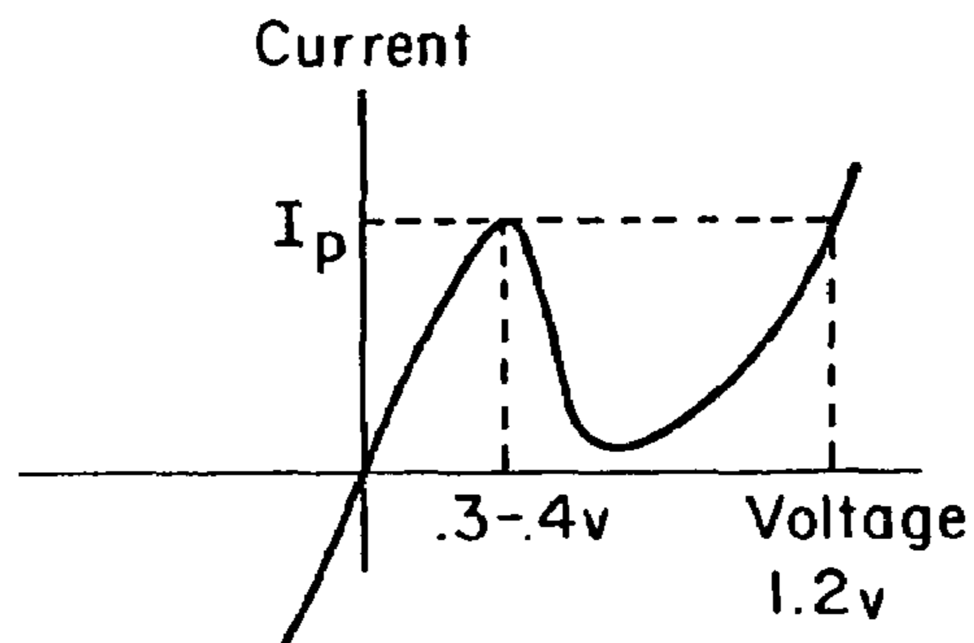
TUNNEL DIODE
