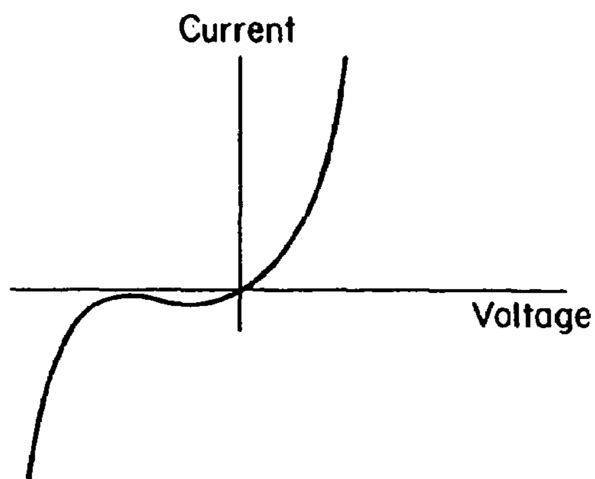
BACK TUNNEL DIODE
