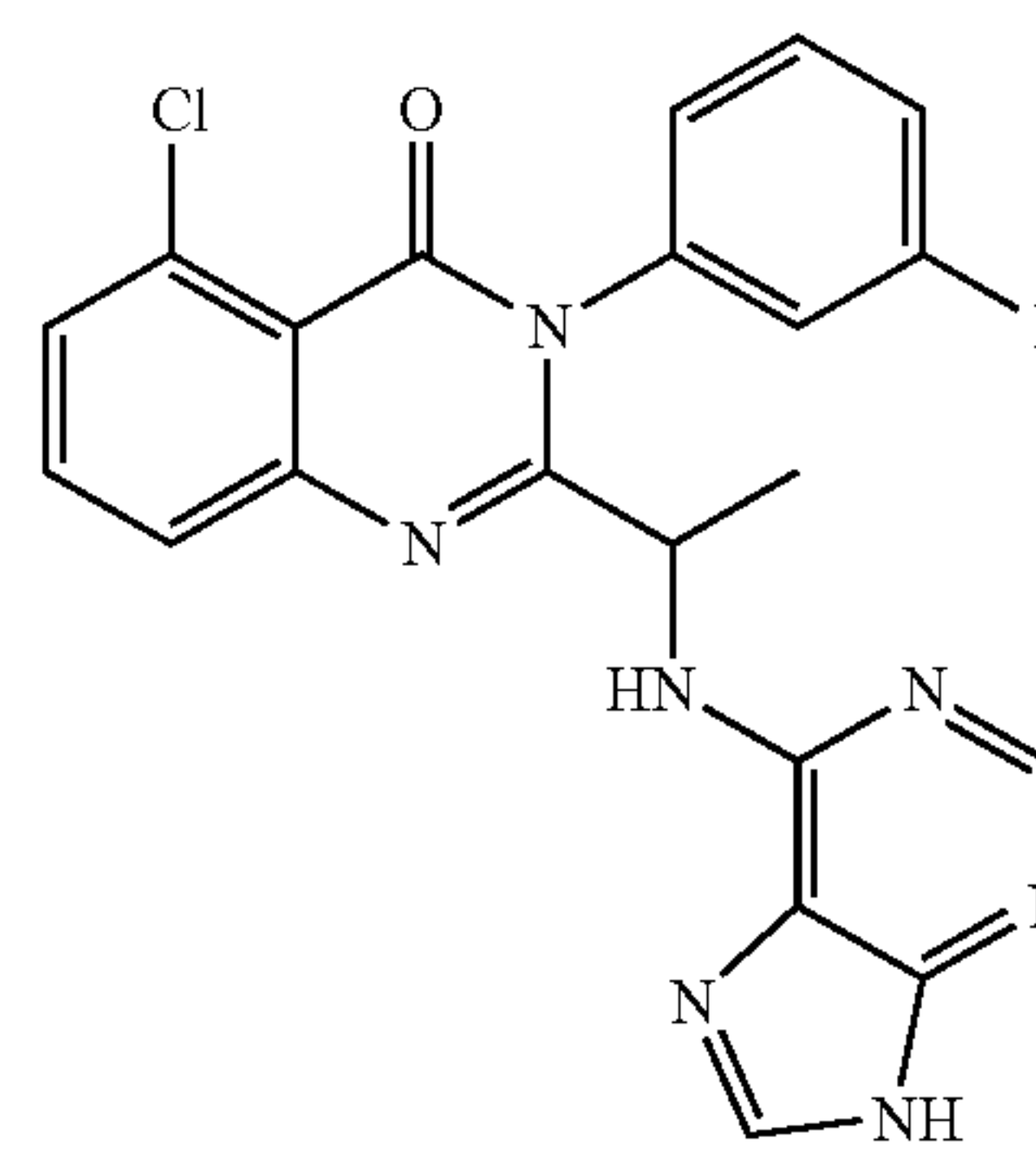
2-[1-(2-amino-9H-purin-6-ylamino)-ethyl]-5-chloro-3-(3-fluoro-phenyl)-3H-quinazolin-4-one (73)
