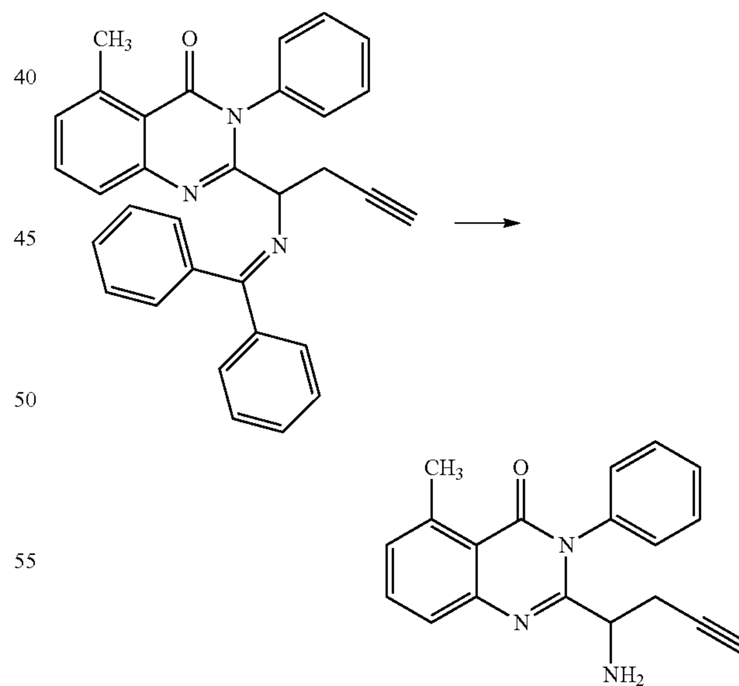
5-methyl-3-phenyl-2-[1-(9H-purin-6-ylamino)-but-3-ynyl]-3H-quinazolin-4-one (161)
