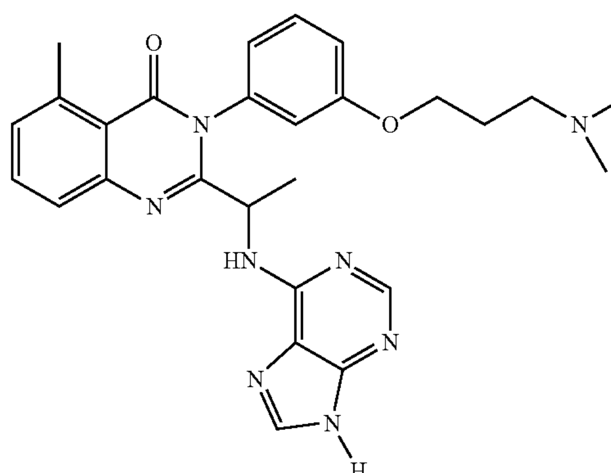
3-[3-(3-Dimethylamino-propoxy)-phenyl]-5-methyl-2-[1-(9H-purin-6-ylamino)-ethyl]-3H-quinazolin-4-one
