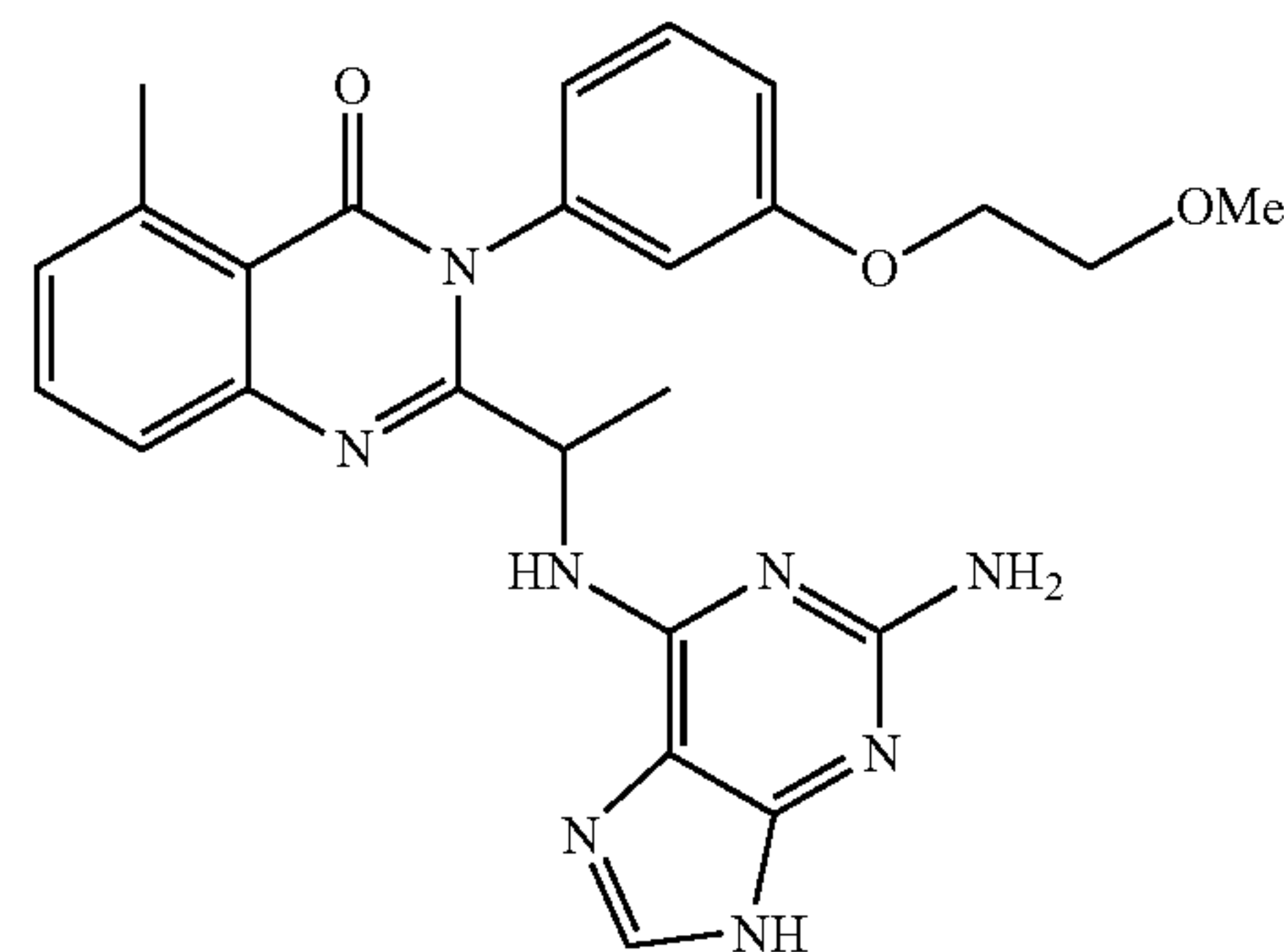
2-[1-(2-Amino-9H-purin-6-ylamino)-ethyl]-3-[3-(2-methoxy-ethoxy)-phenyl]-5-methyl-3H-quinazolin-4-one
