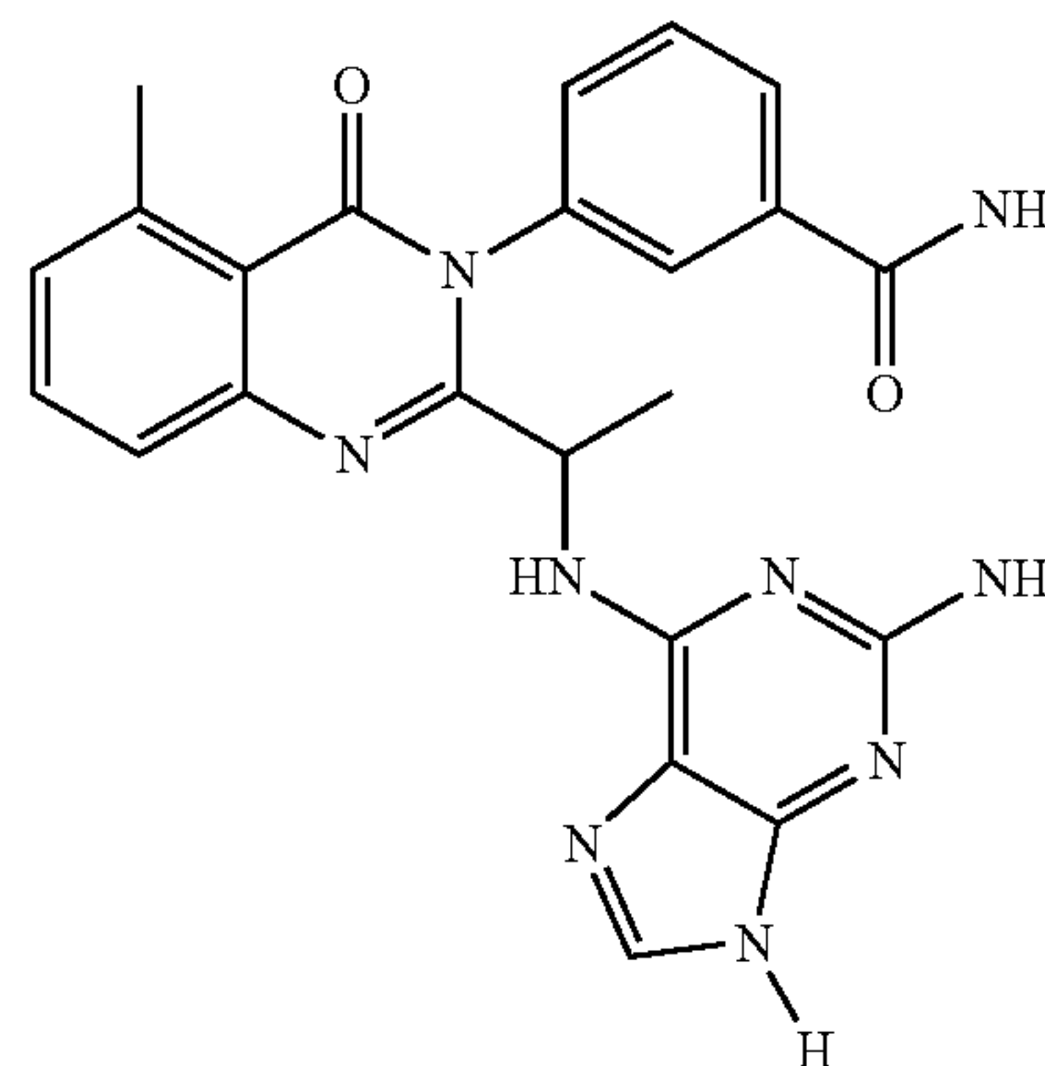
3-{2-[1-(2-Amino-9H-purin-6-ylamino)-ethyl]-5-methyl-4-oxo-4H-quinazolin-3-yl}-benzamide
