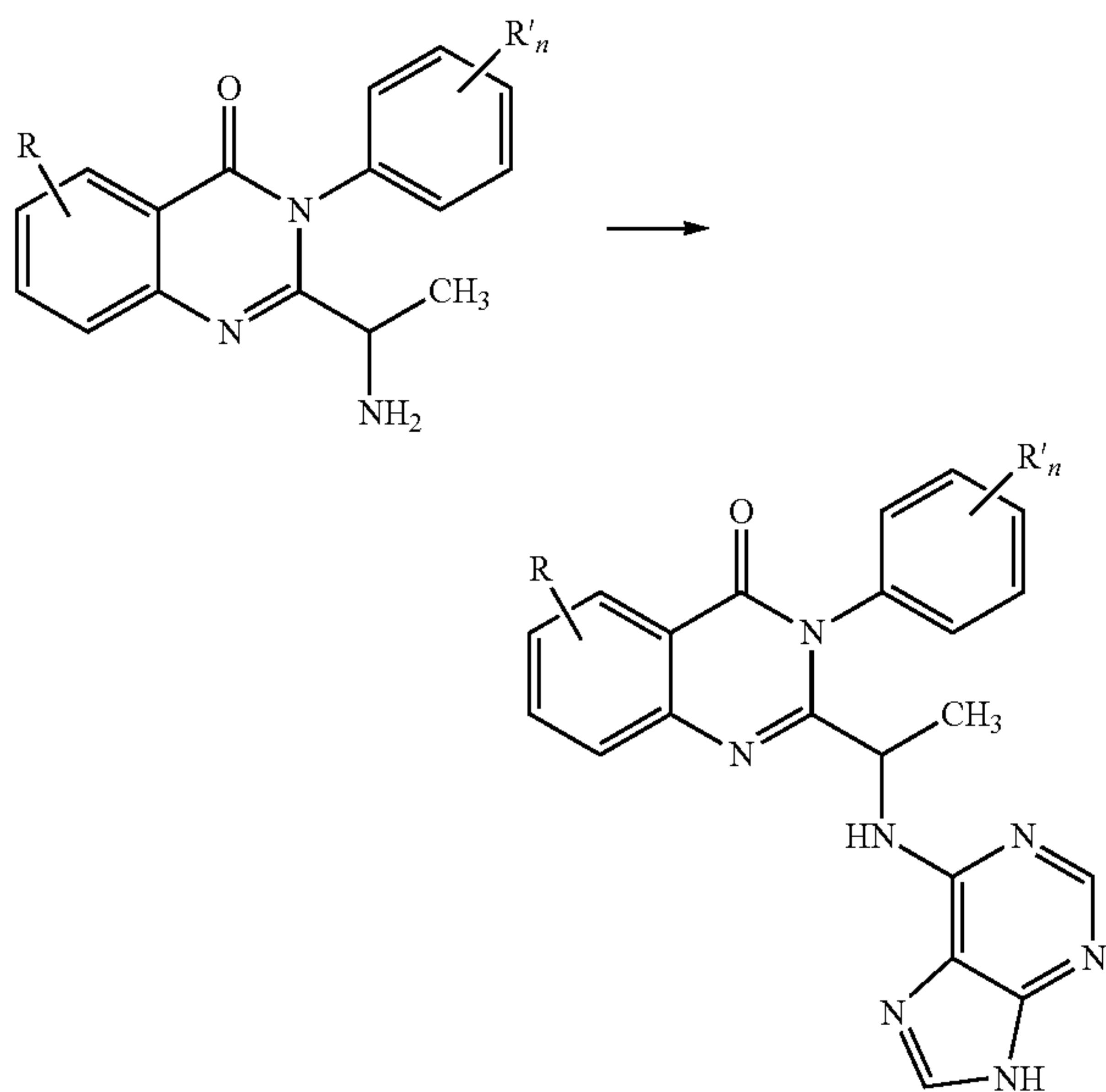
5-chloro-3-(3,5-difluoro-phenyl)-2-[1-(9H-purin-6-ylamino)-ethyl]-3H-quinazolin-4-one (166)
