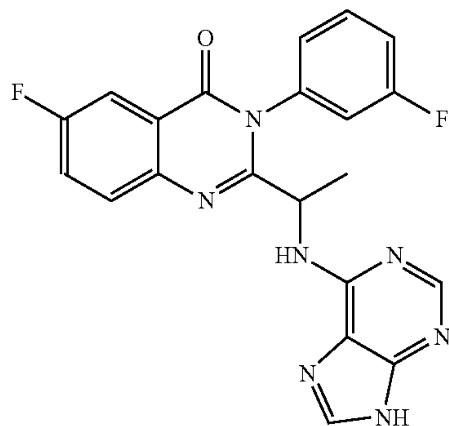
2-[4-diethylamino-1-(9H-purin-6-ylamino)-butyl]-5-methyl-3-phenyl-3H-quinazolin-4-one (103)
