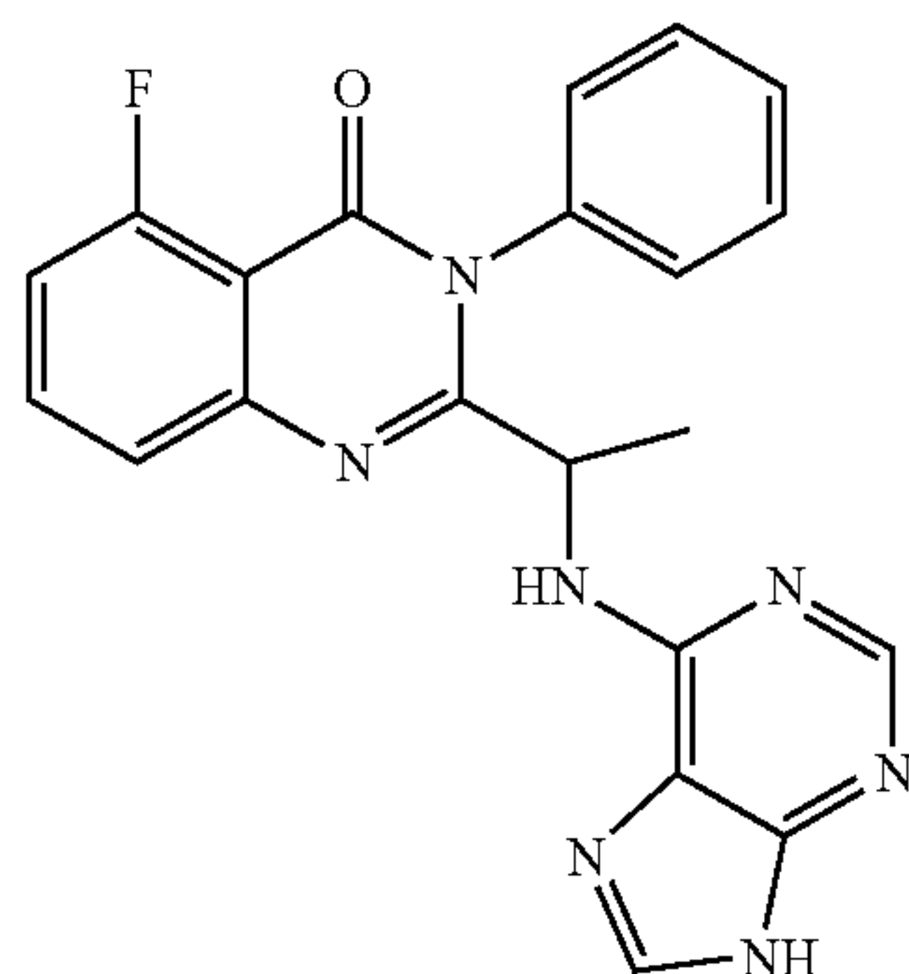
2-[1-(2-amino-9H-purin-6-ylamino)-ethyl]-5-fluoro-3-phenyl-3H-quinazolin-4-one (47)
