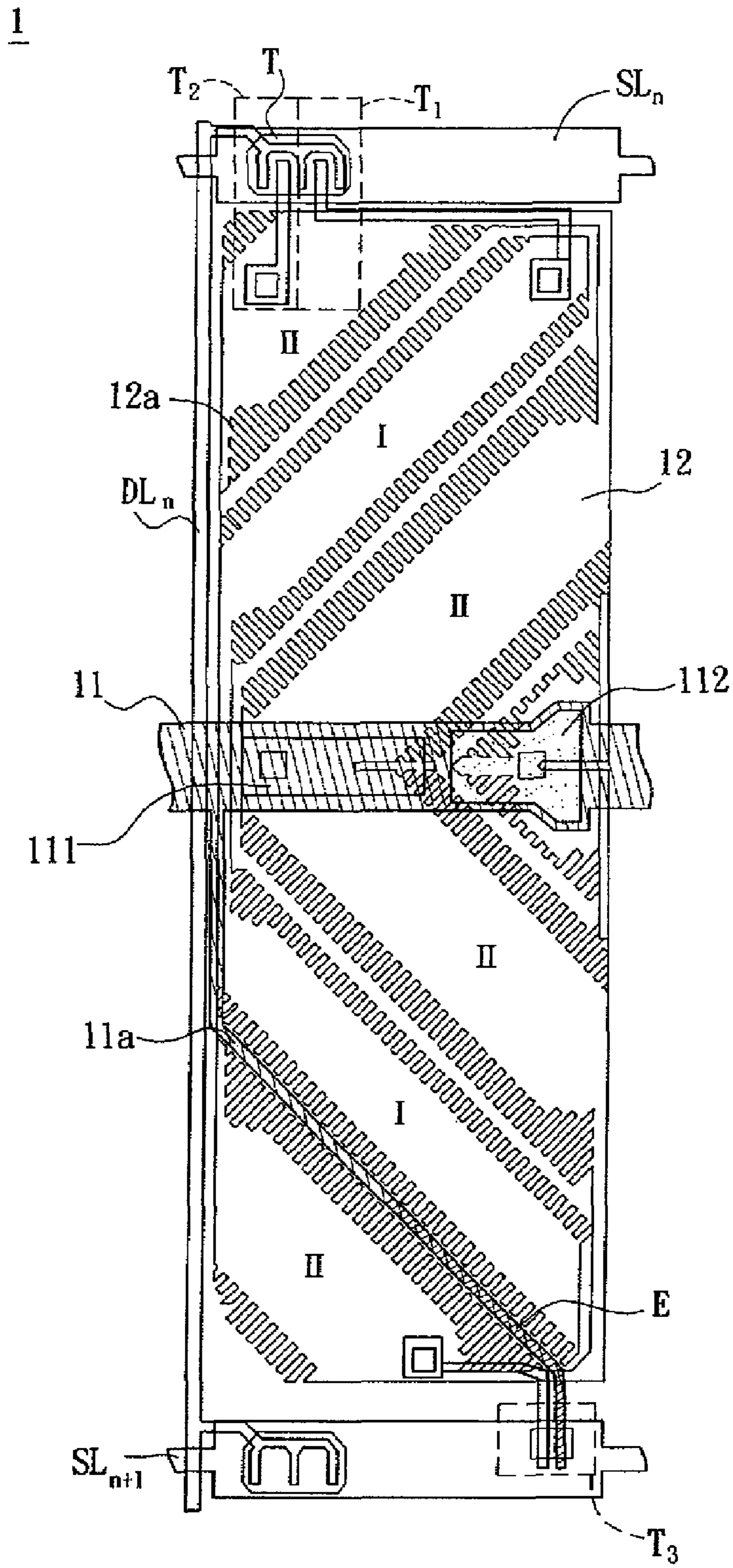
FIG. 2(PRIOR ART)
