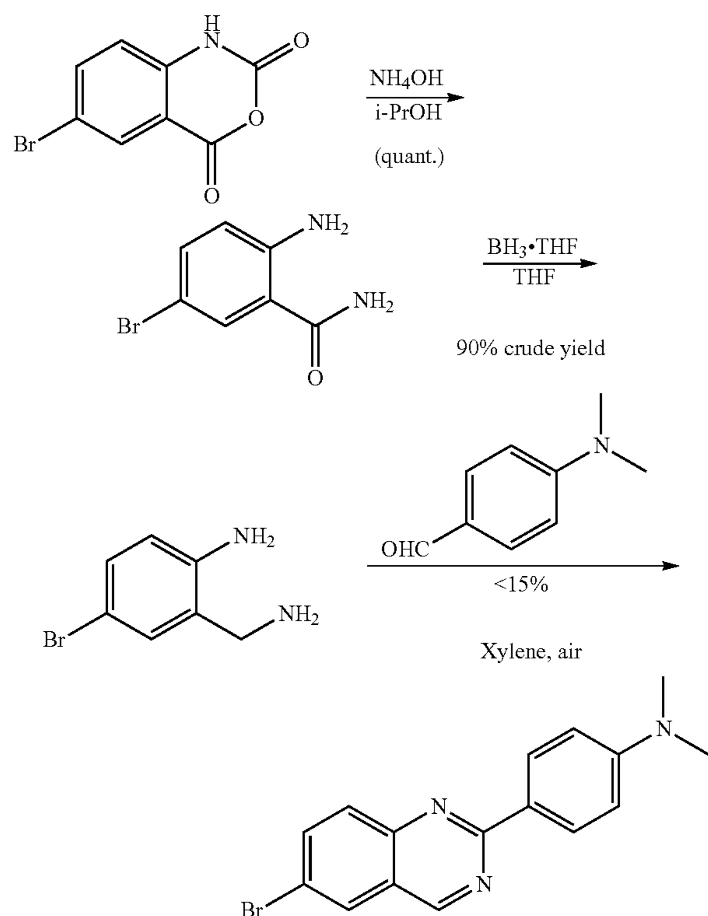
SCHEME 18
