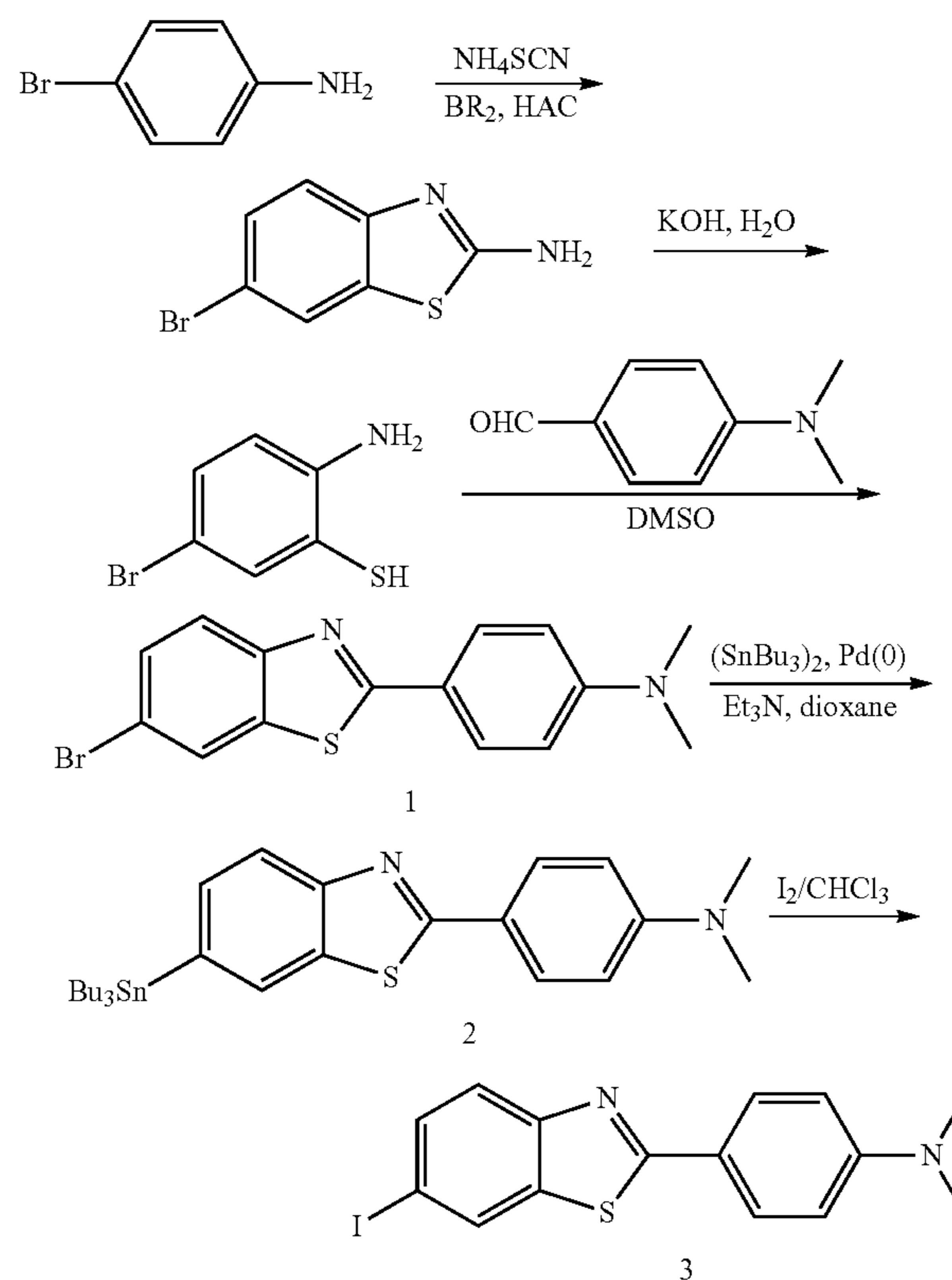
SCHEME 1
