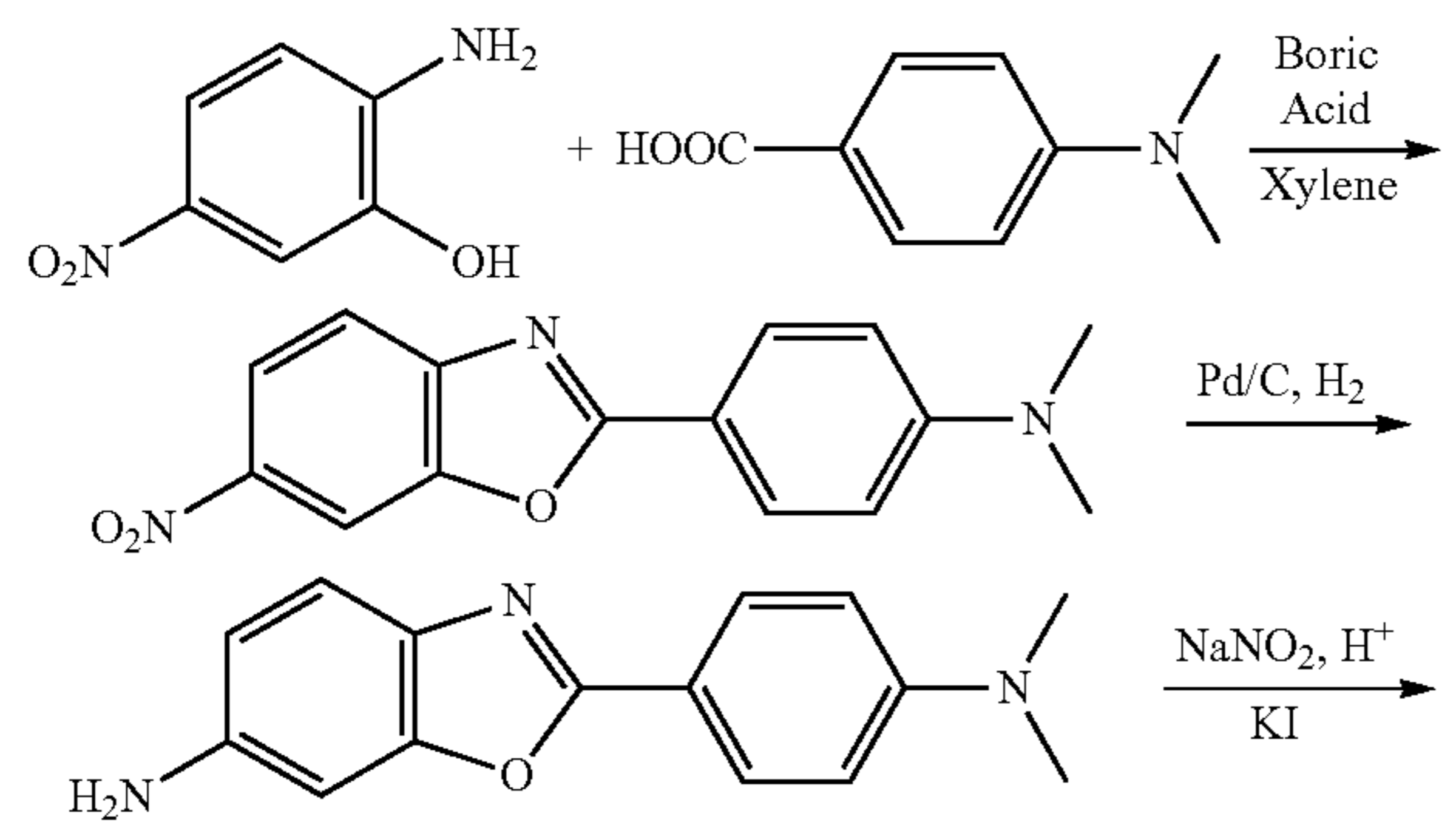
SCHEME 4
