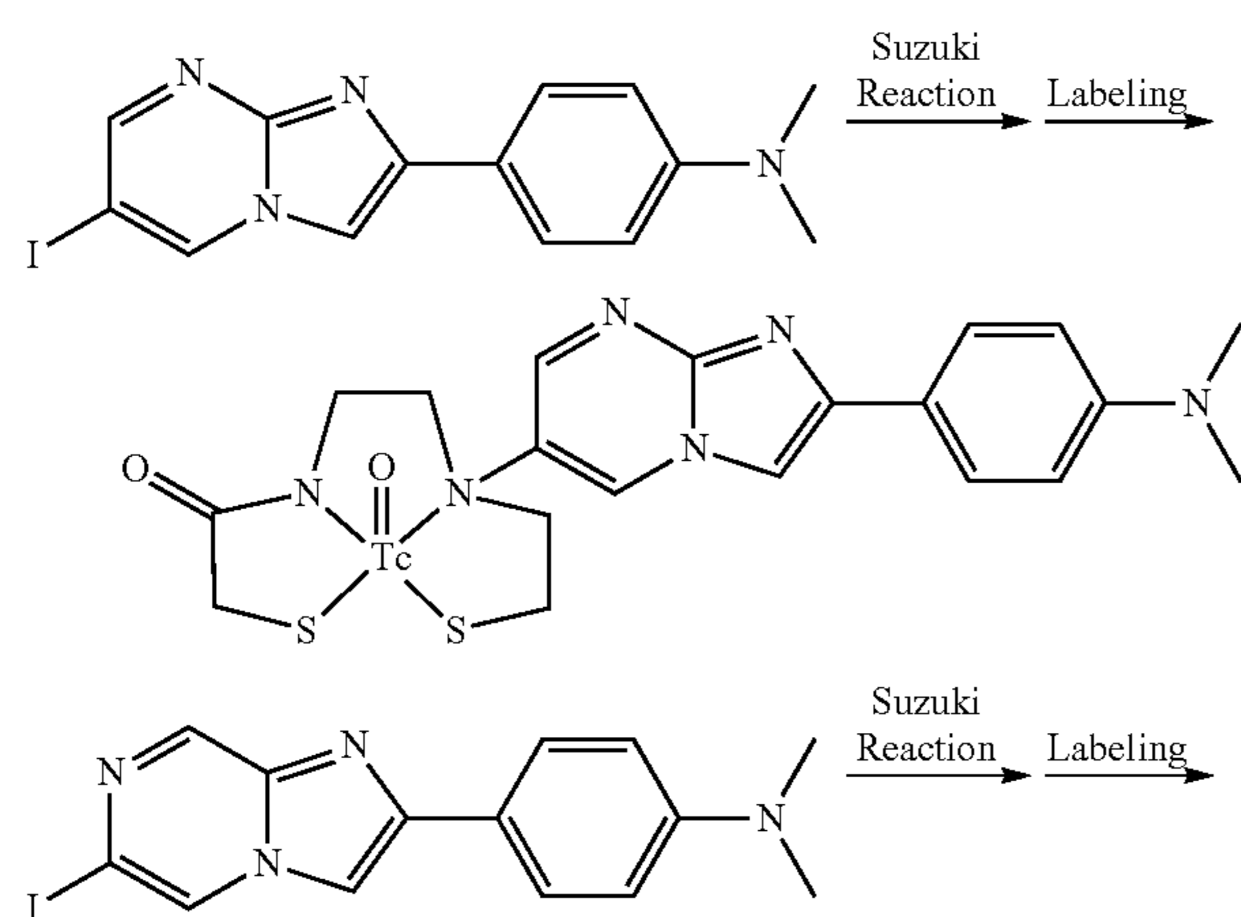
SCHEME 23
