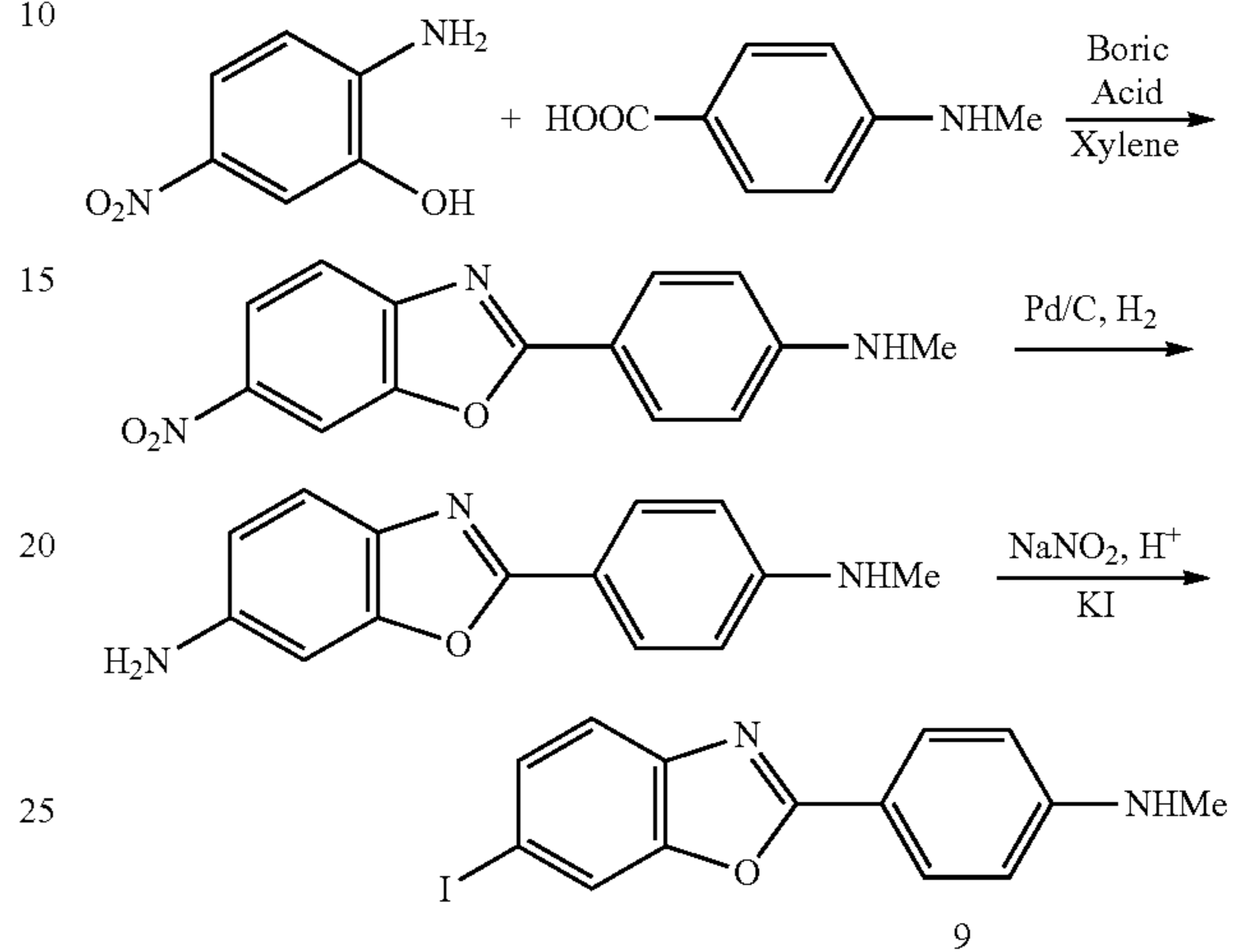
SCHEME 5
