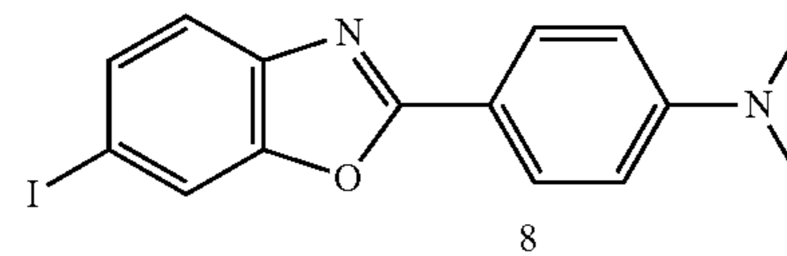
SCHEME 5
