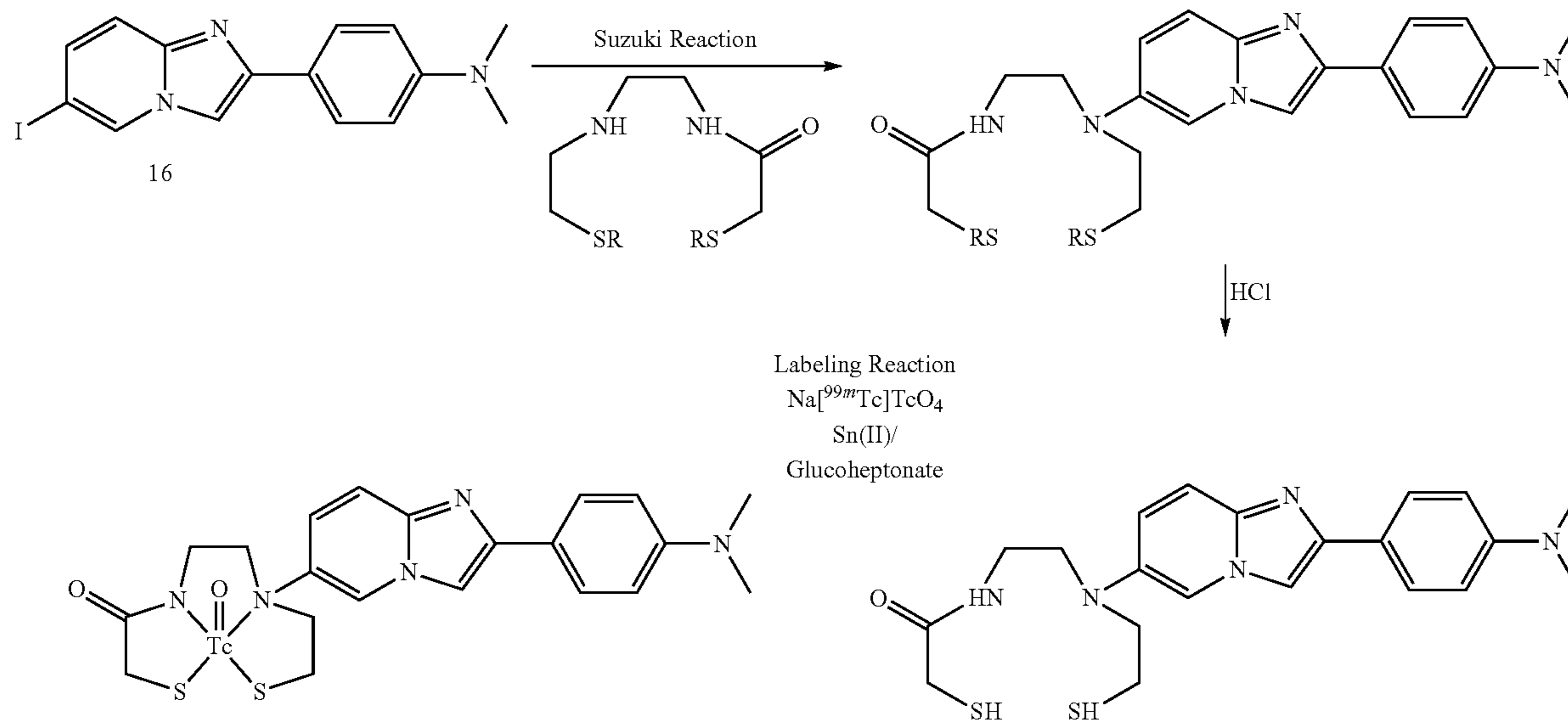
SCHEME 17
