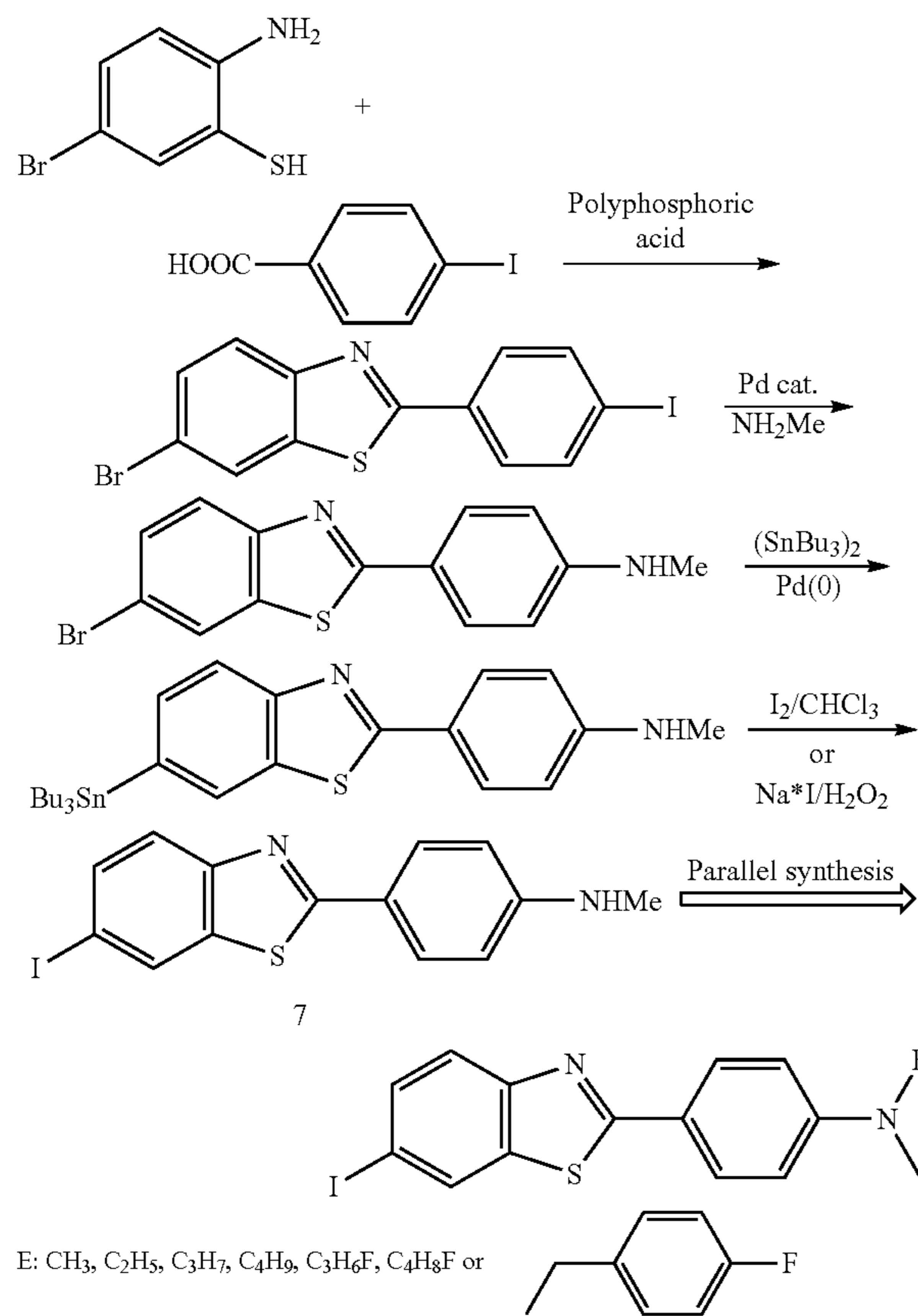
SCHEME 3
