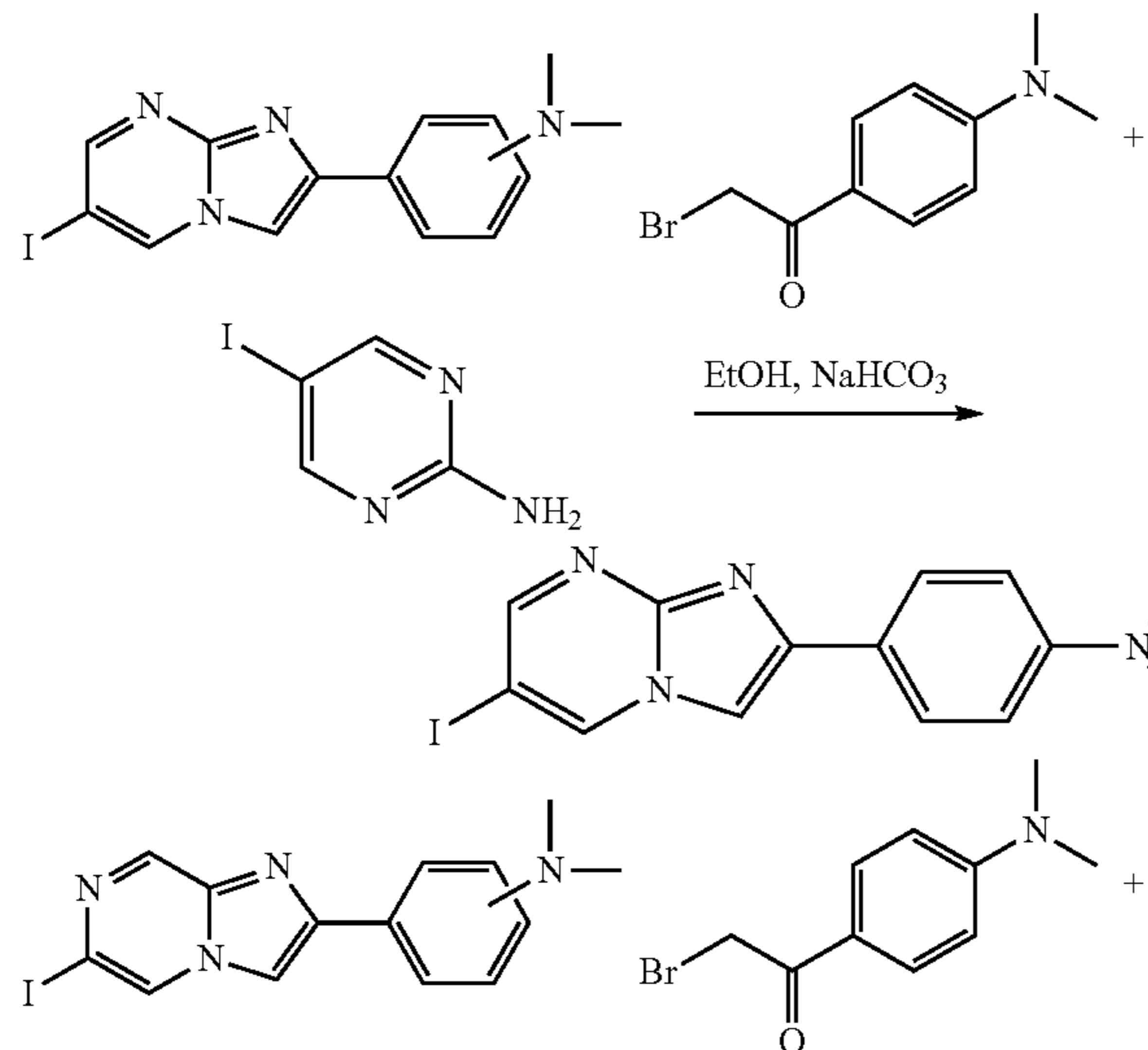
SCHEME 21
