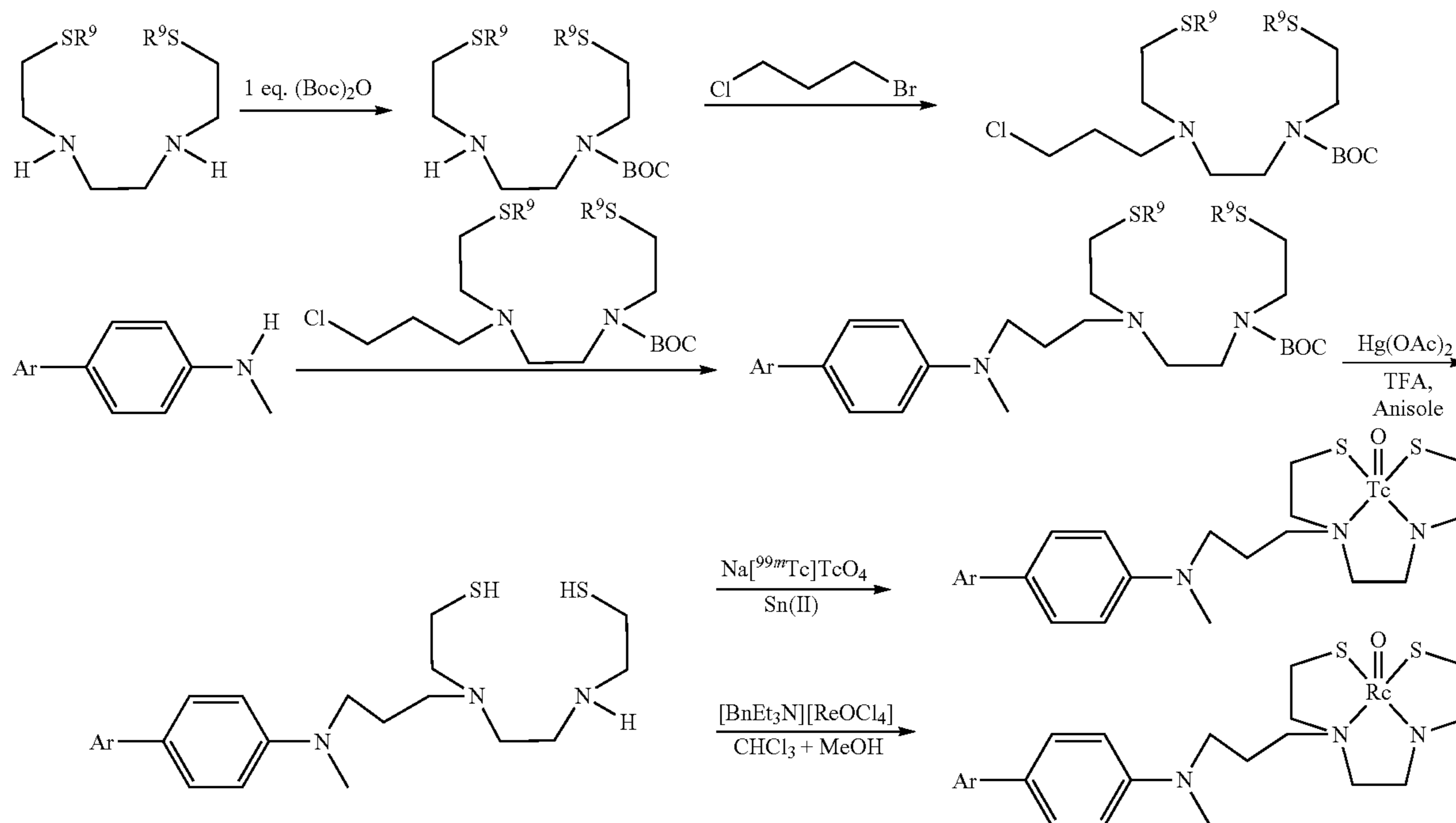
SCHEME 20
