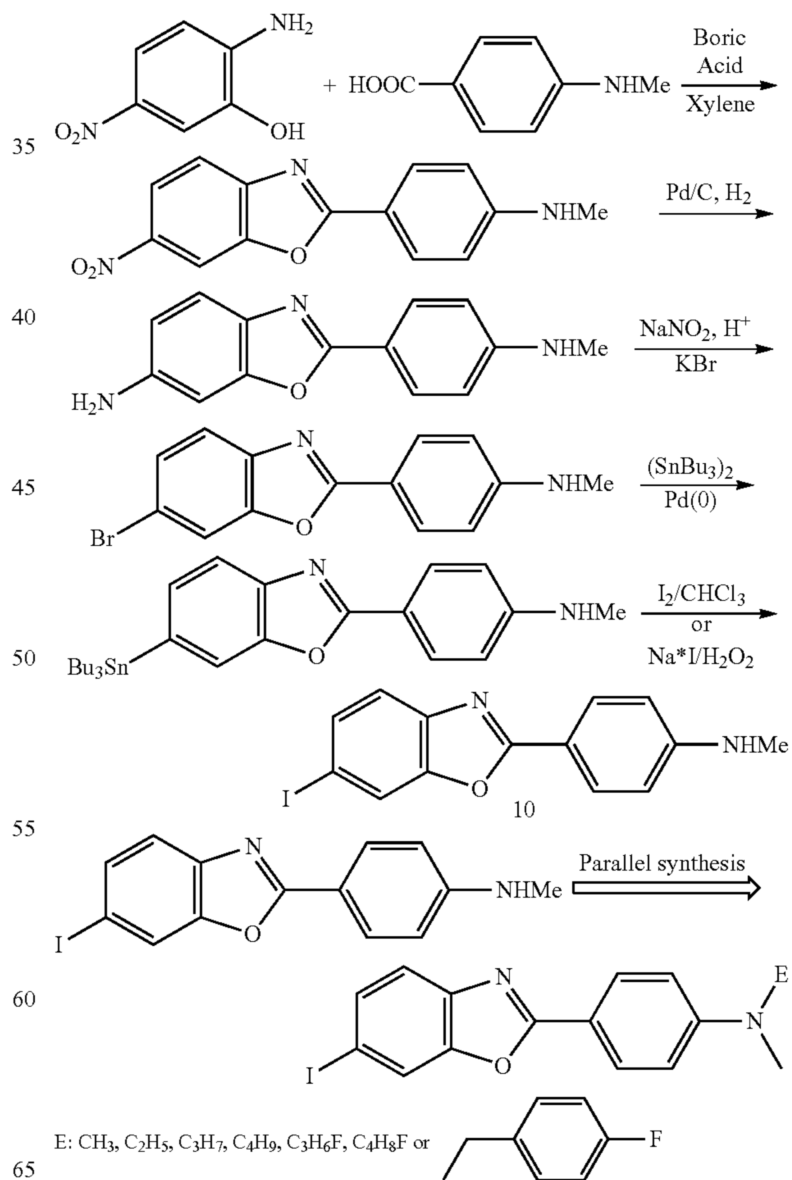
SCHEME 6
