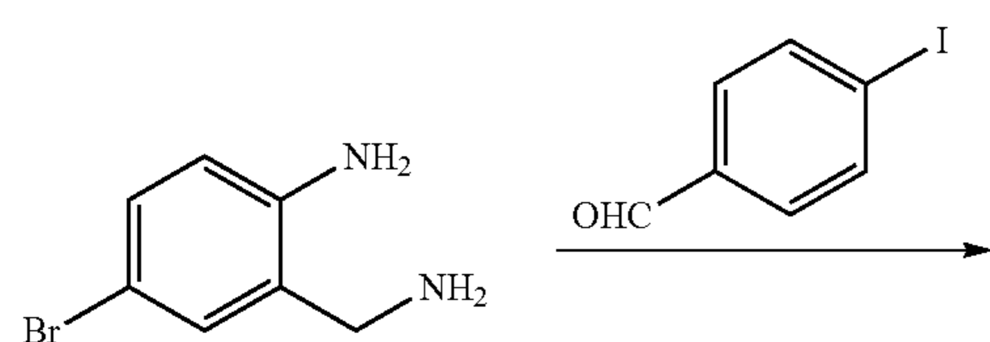
SCHEME 19
