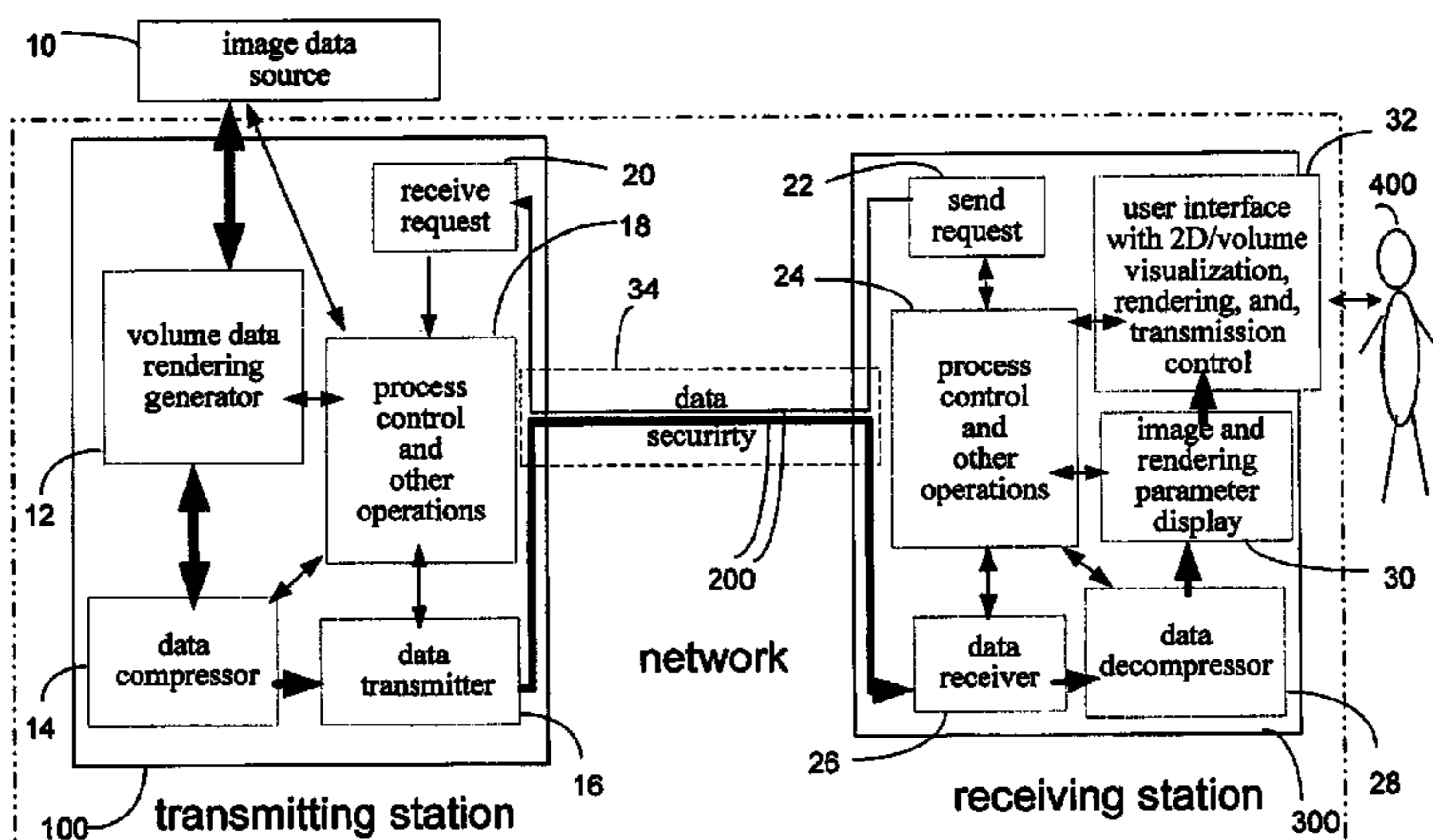
teleradiology system with remote volume data rendering / visualization capability
