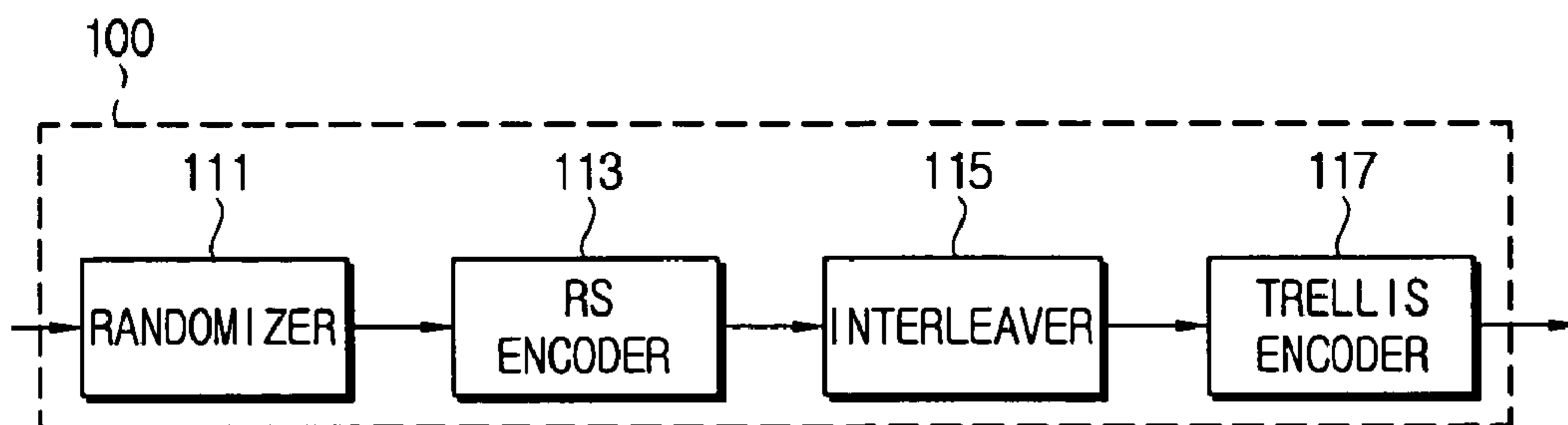
FIG. 1 (PRIOR ART)
