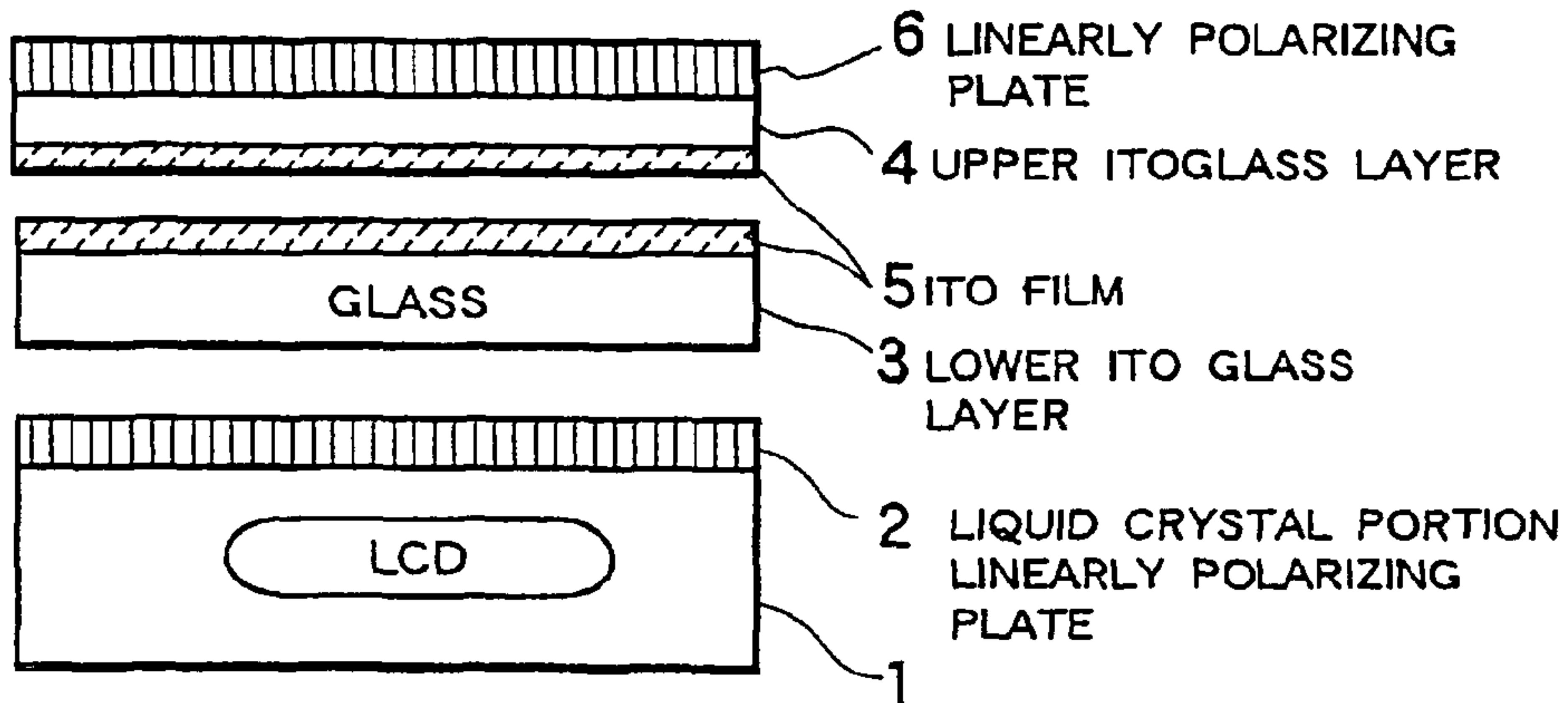
FIG.12 PRIOR ART
