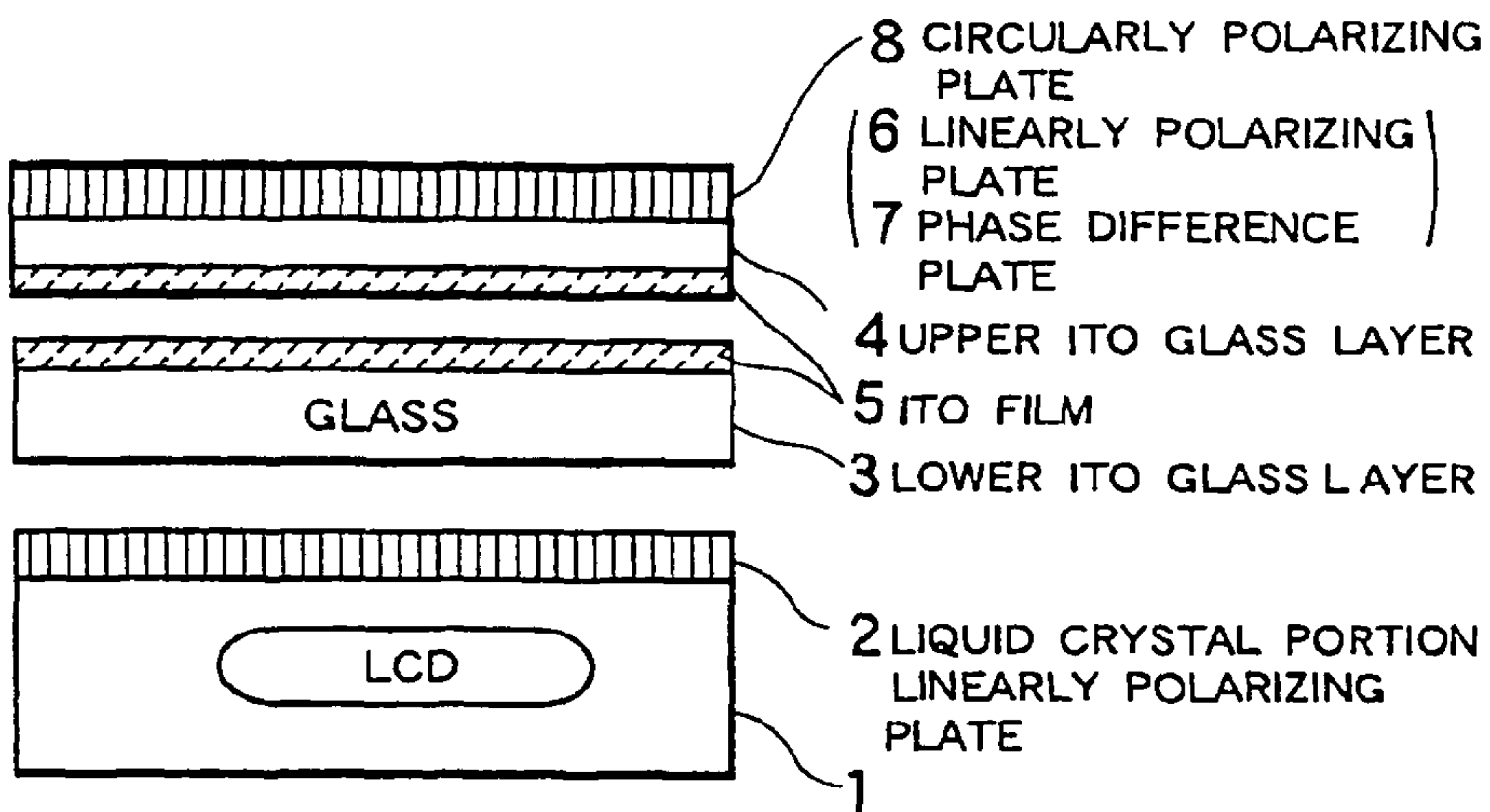
FIG.12 PRIOR ART
