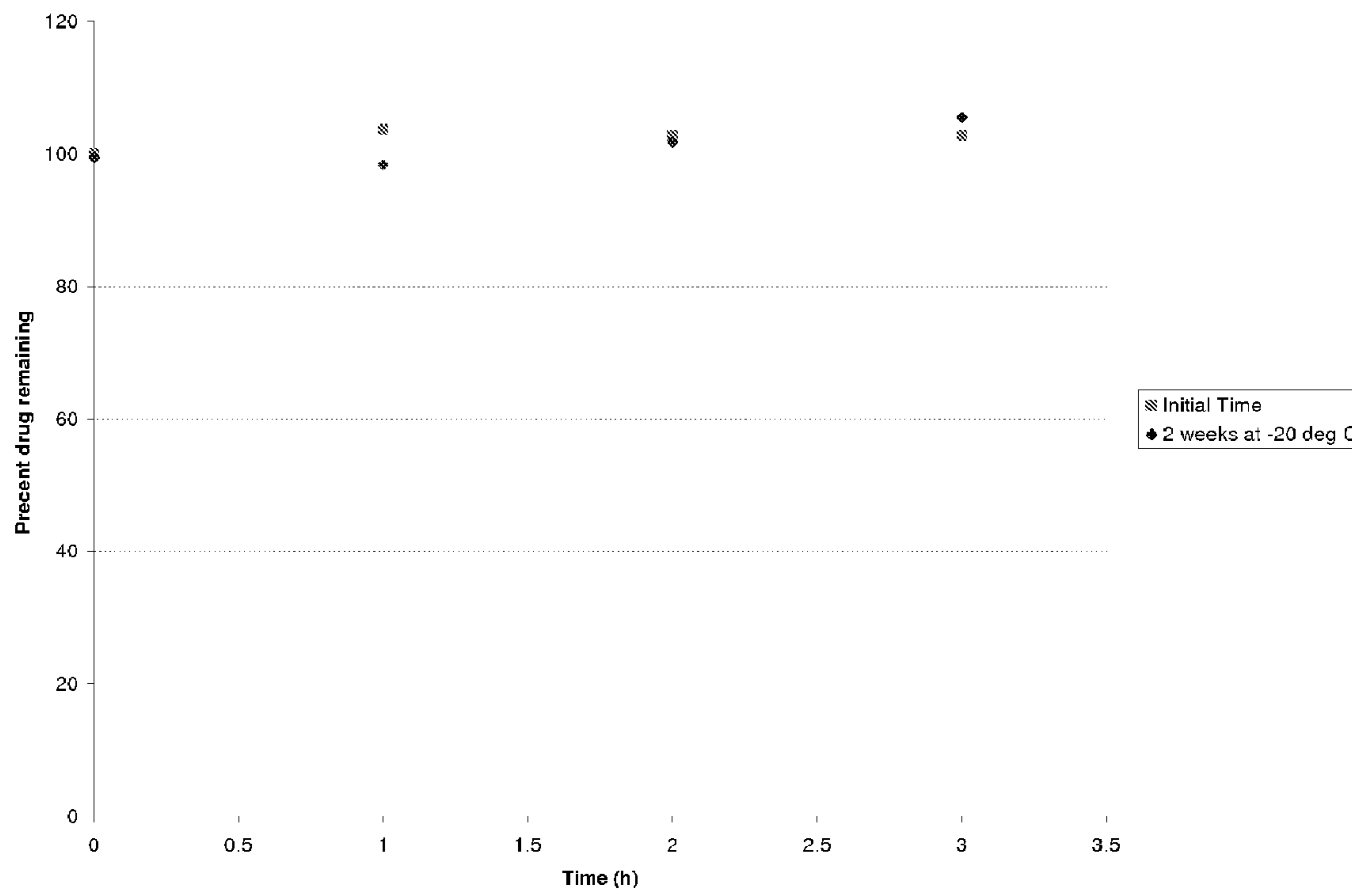
FIGURE 27 Stability of BH4 (1 mg/mL) in 5% mannitol aqueous solution
