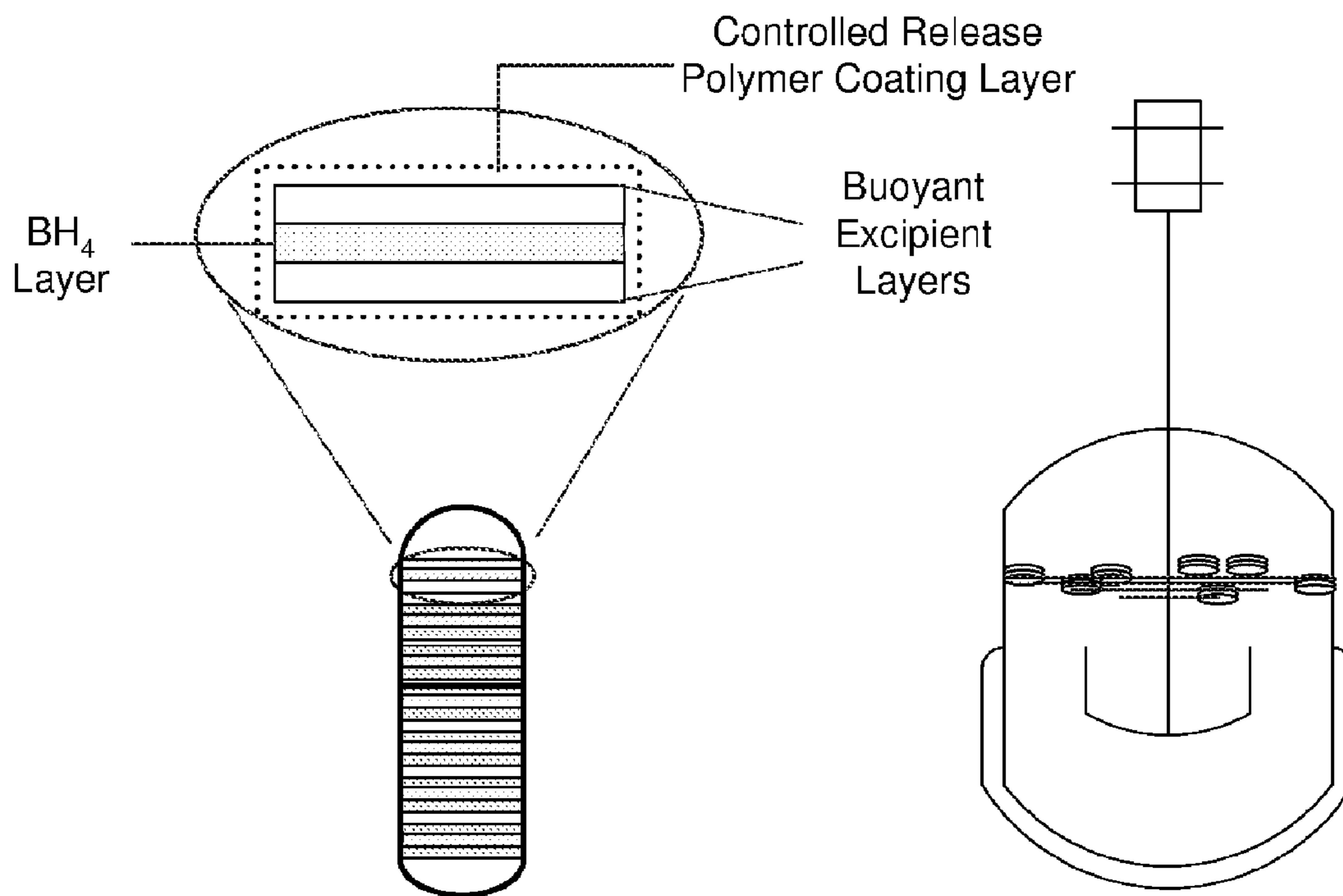
Schematic Diagram of Floating Dosage Form
