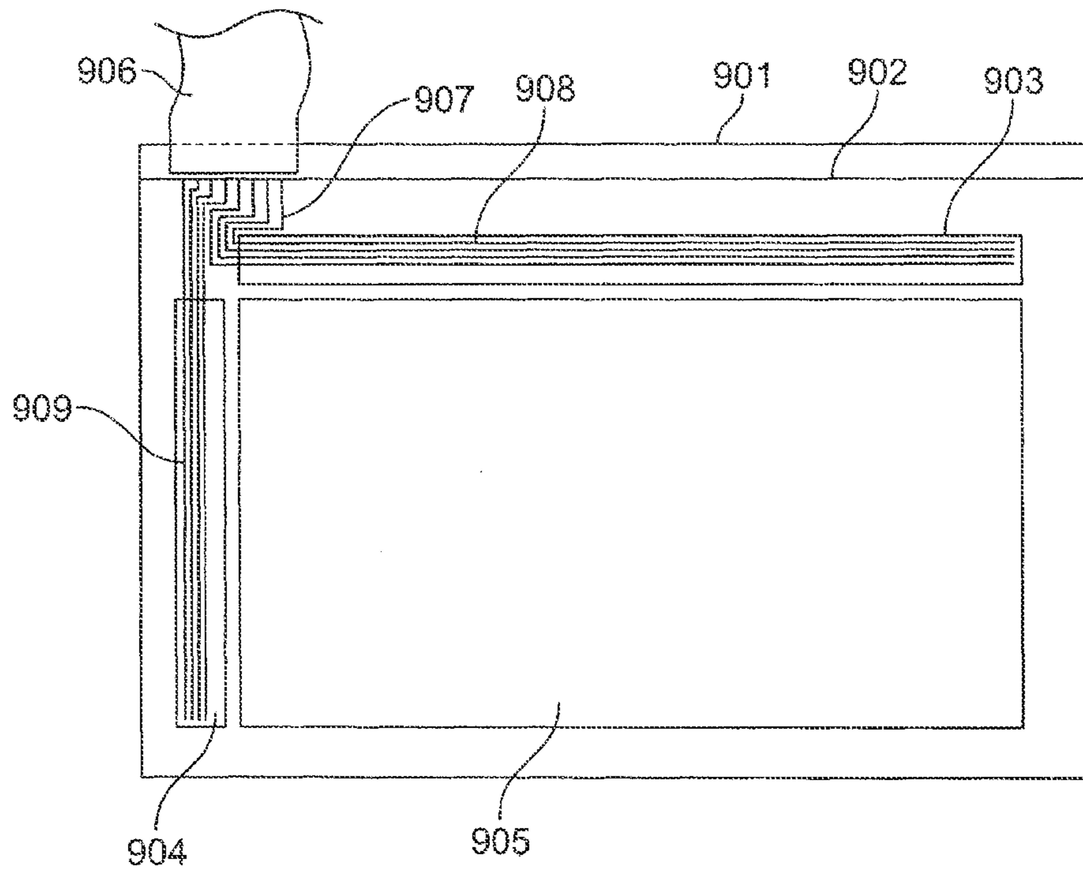
FIG. 5 (Prior Art)
