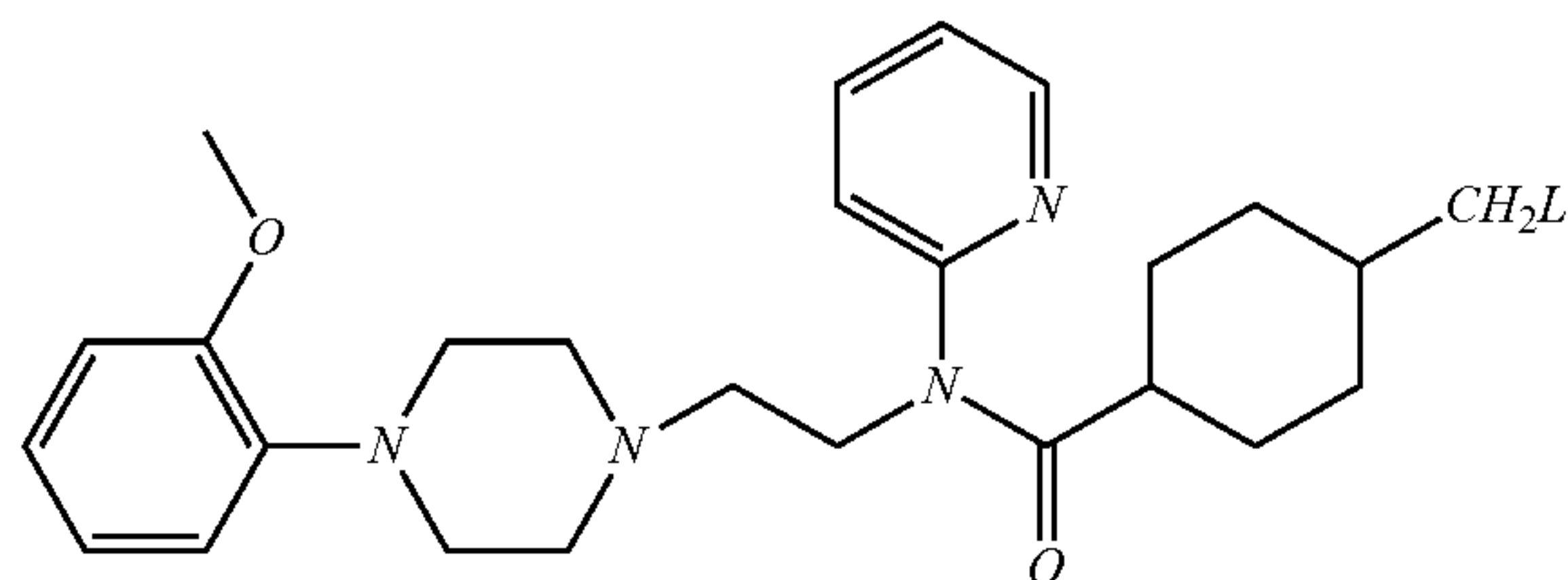
Formula III 5
