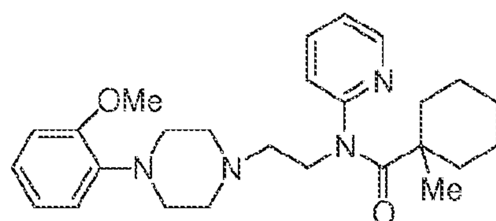
SWAY
