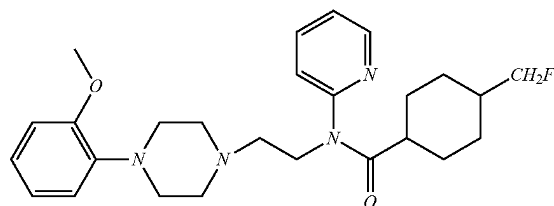
Formula II
