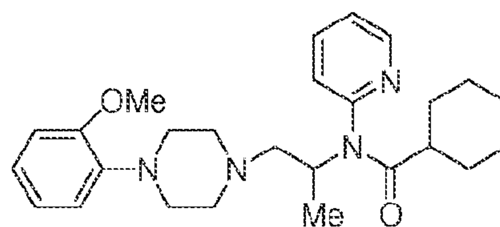
(R,S)-JWAY
