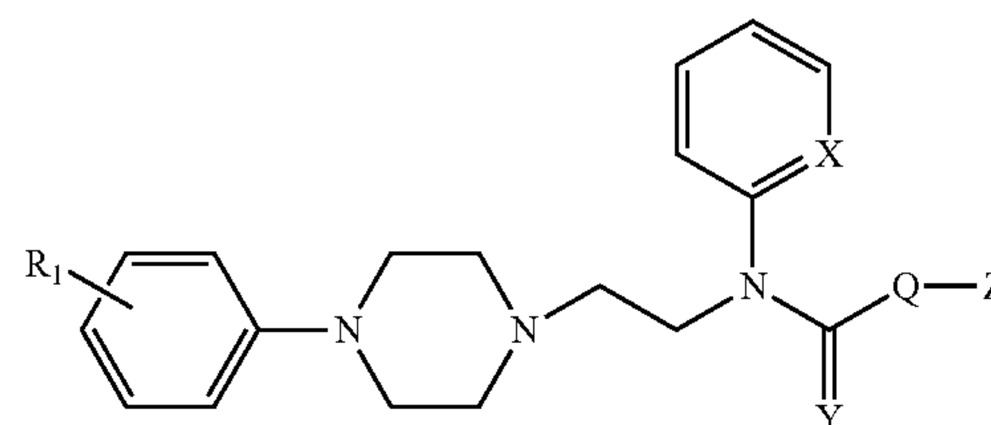
Formula I
