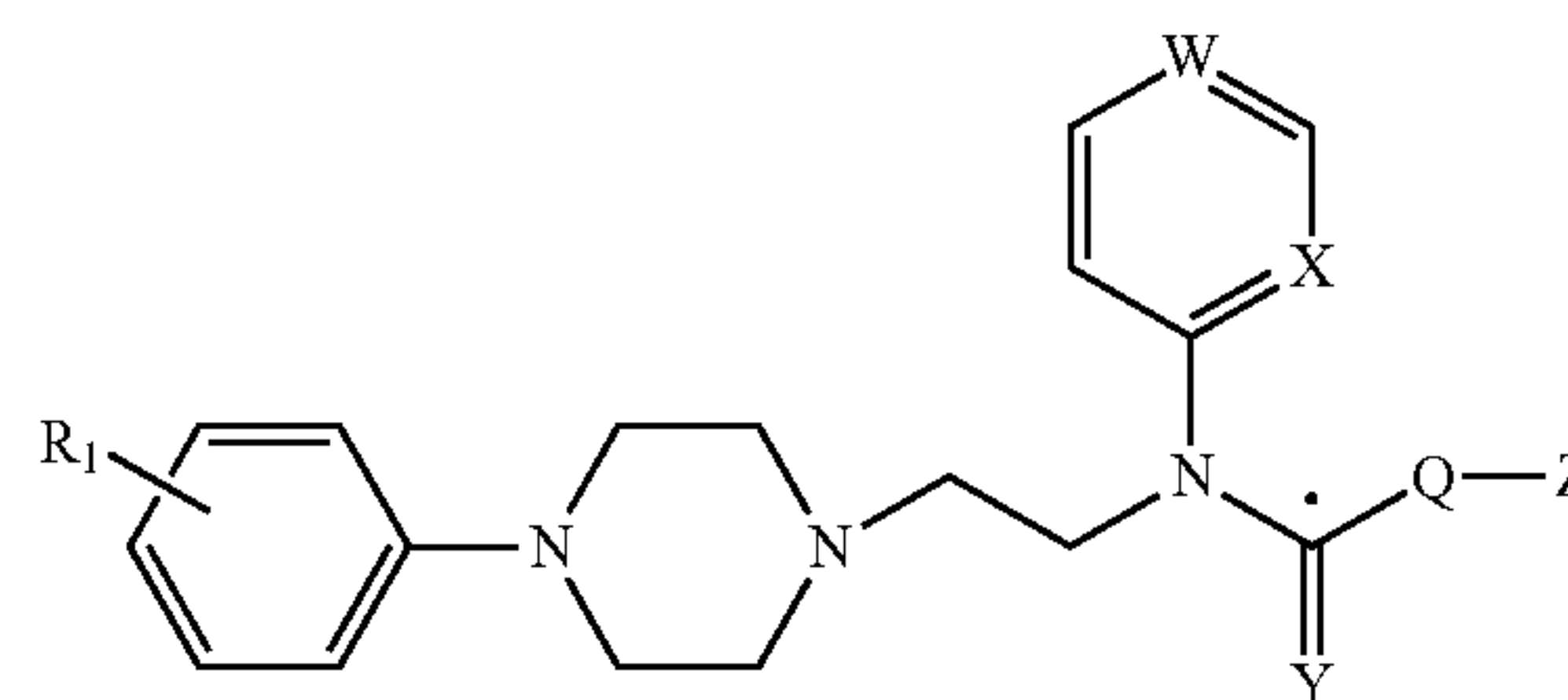
Formula I
