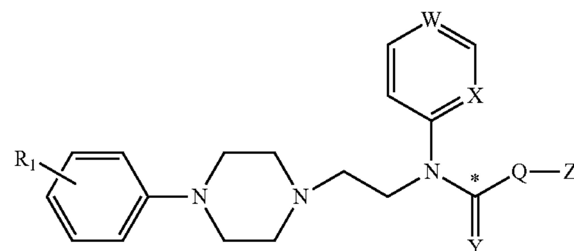
Formula I
