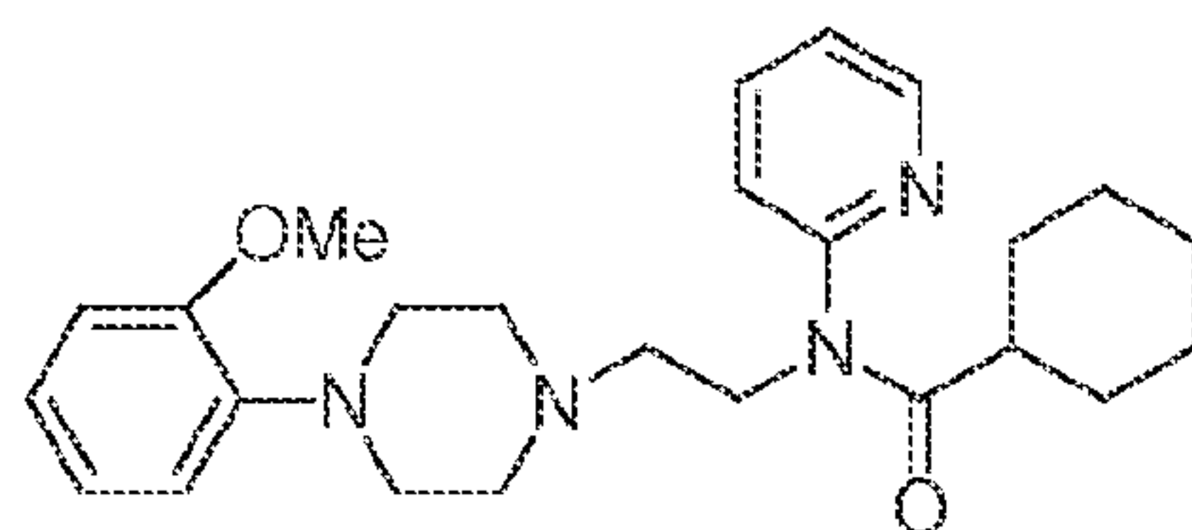
WAY-100635
