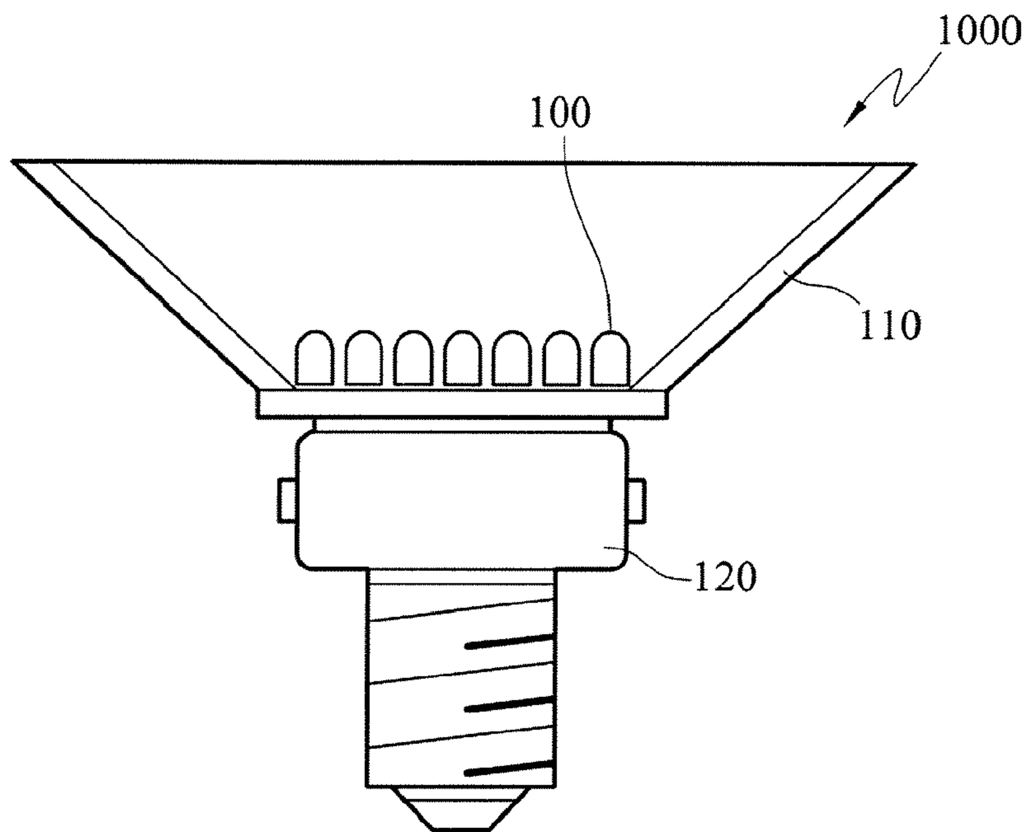
FIG. 1 (PRIOR ART)
