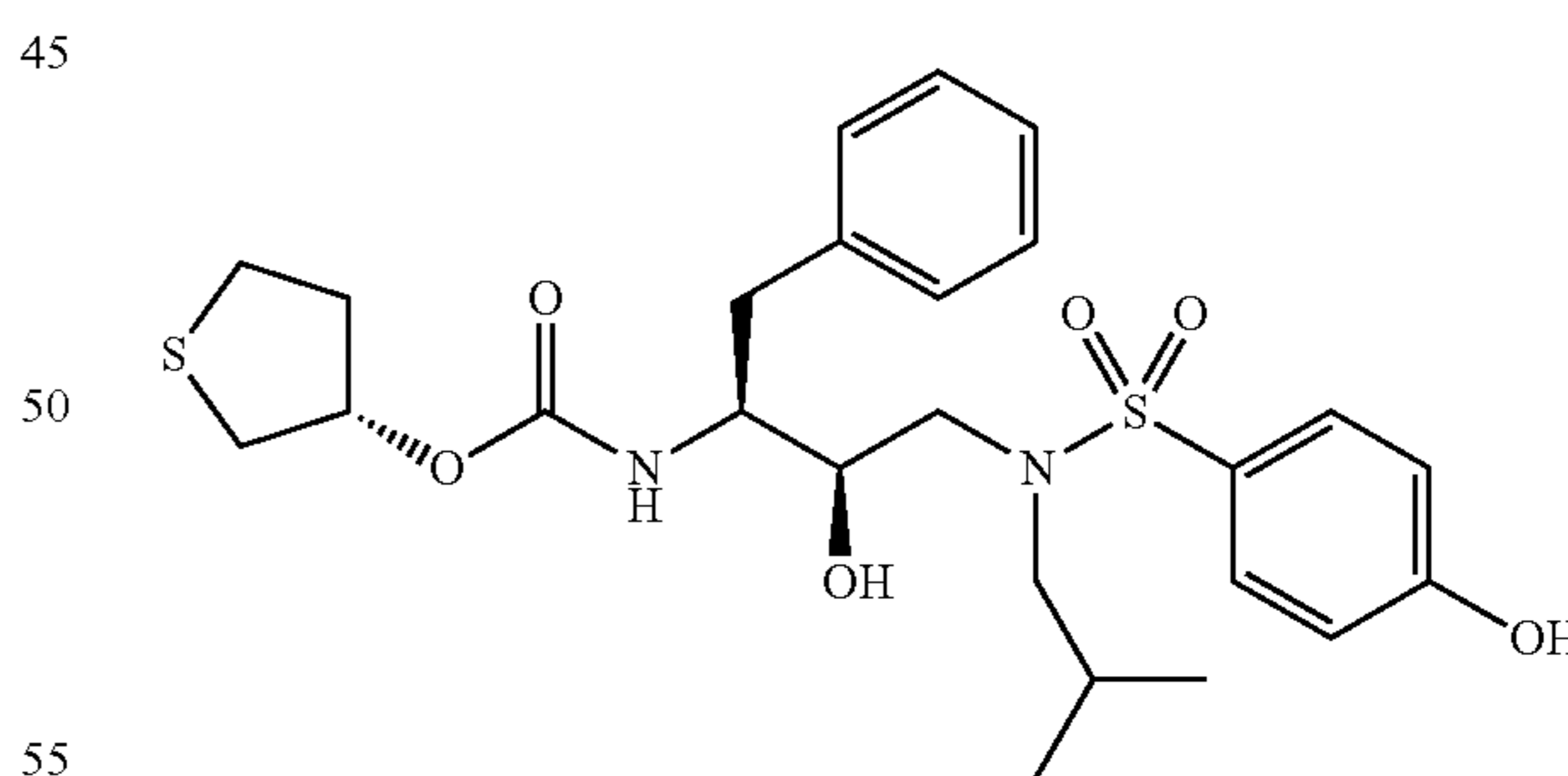
Preparation of Carbamic acid, [2R-hydroxy-3-[(4-hydroxyphenyl)sulfonyl](2-methylpropyl)amino]-1S-(phenylmethyl)propyl-, 3-S-tetrahydrothiophen-3-yl-ester
