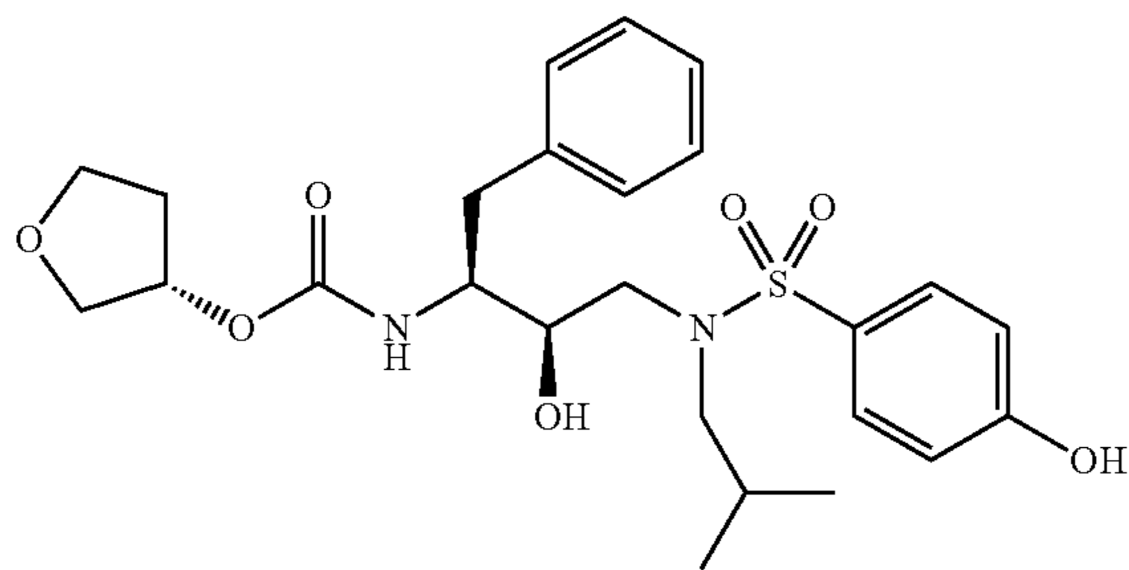
Preparation of Carbamic acid, [2R-hydroxy-3-[(4-hydroxyphenyl)sulfonyl](2-methylpropyl)amino]-1S-(phenylmethyl)propyl-, 3-S-tetrahydrofuran-3-yl-ester
