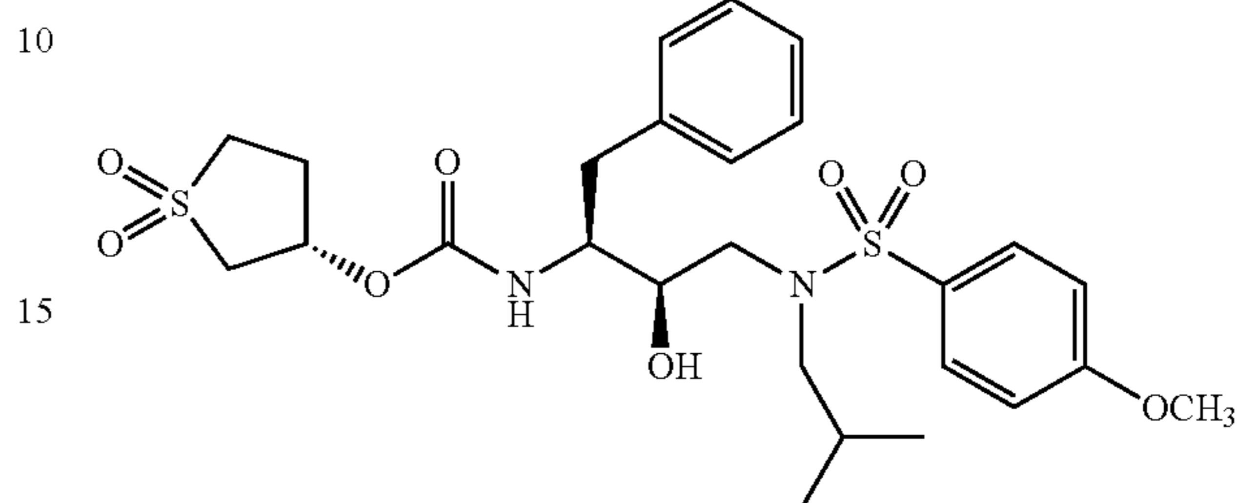
Preparation of Carbamic acid, [2R-hydroxy-3-[(4-methoxyphenyl)sulfonyl](2-methylpropyl)amino]-1S-(phenylmethyl)propyl-, 3(S)-1,1-dioxotetrahydrothiophen-3-yl-ester
