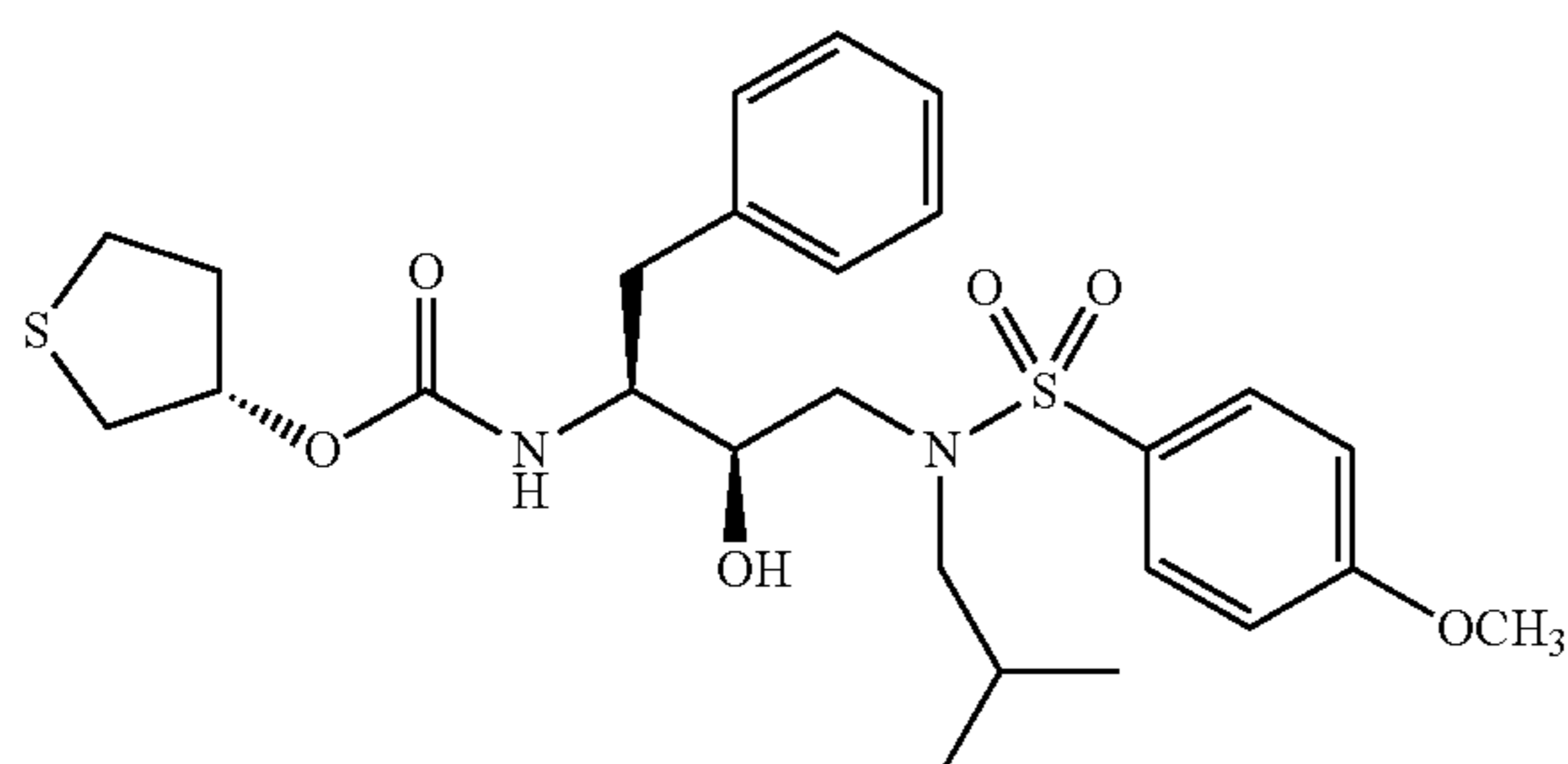
Preparation of Carbamic acid, [2R-hydroxy-3-[(4-methoxyphenyl)sulfonyl](2-methylpropyl)amino]-1S-(phenylmethyl)propyl-, 3-S-tetrahydrothiophen-3-yl-ester
