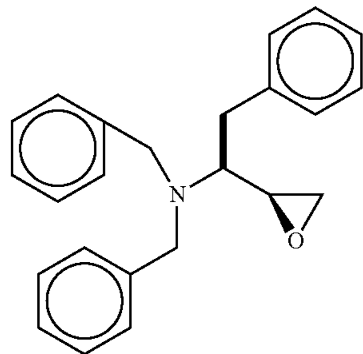
Preparation of N,N-dibenzyl-3(S)-amino-1,2-(S)-epoxy-4-phenylbutane
