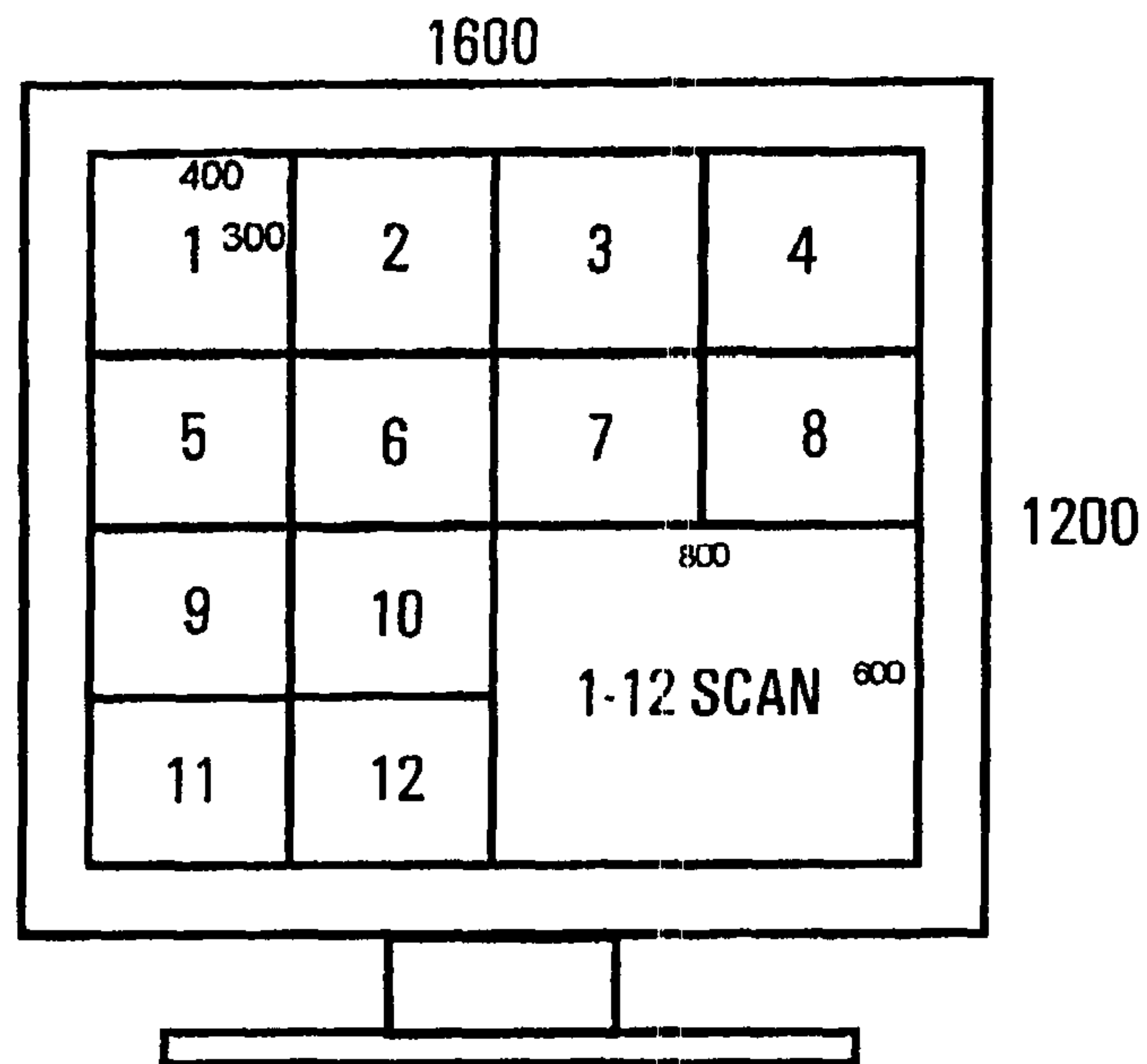
20" TO 21" SUPER HIGH RESOLUTION MONITOR
