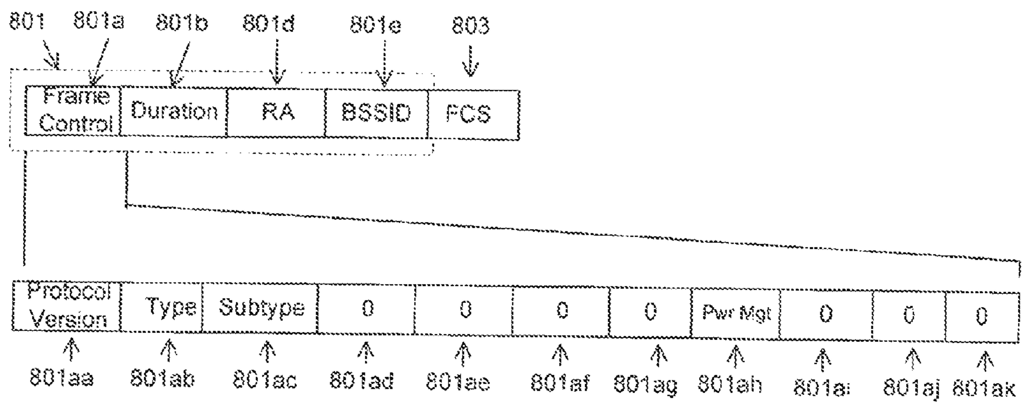
WLAN CF-End Control Frame Format Figure 8.0
