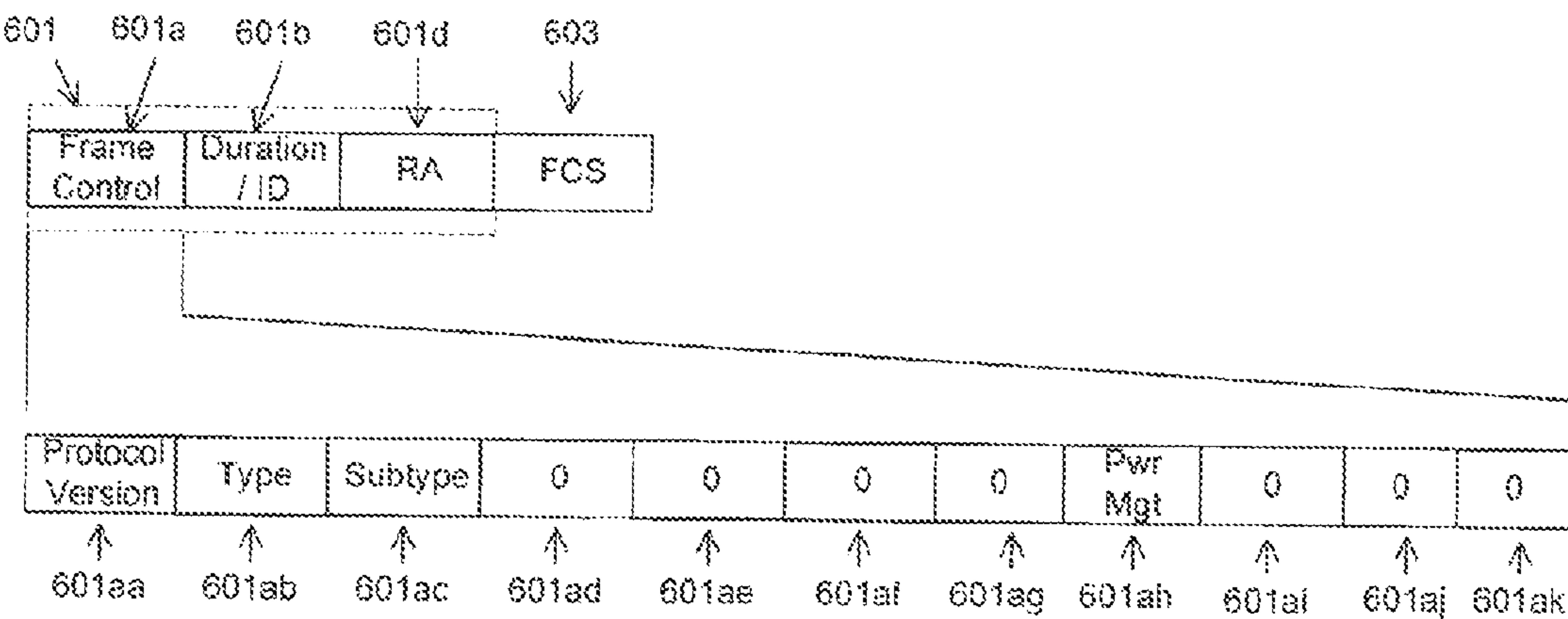
WLAN Acknowledgement (ACK) Control Frame Format Figure 6.0
