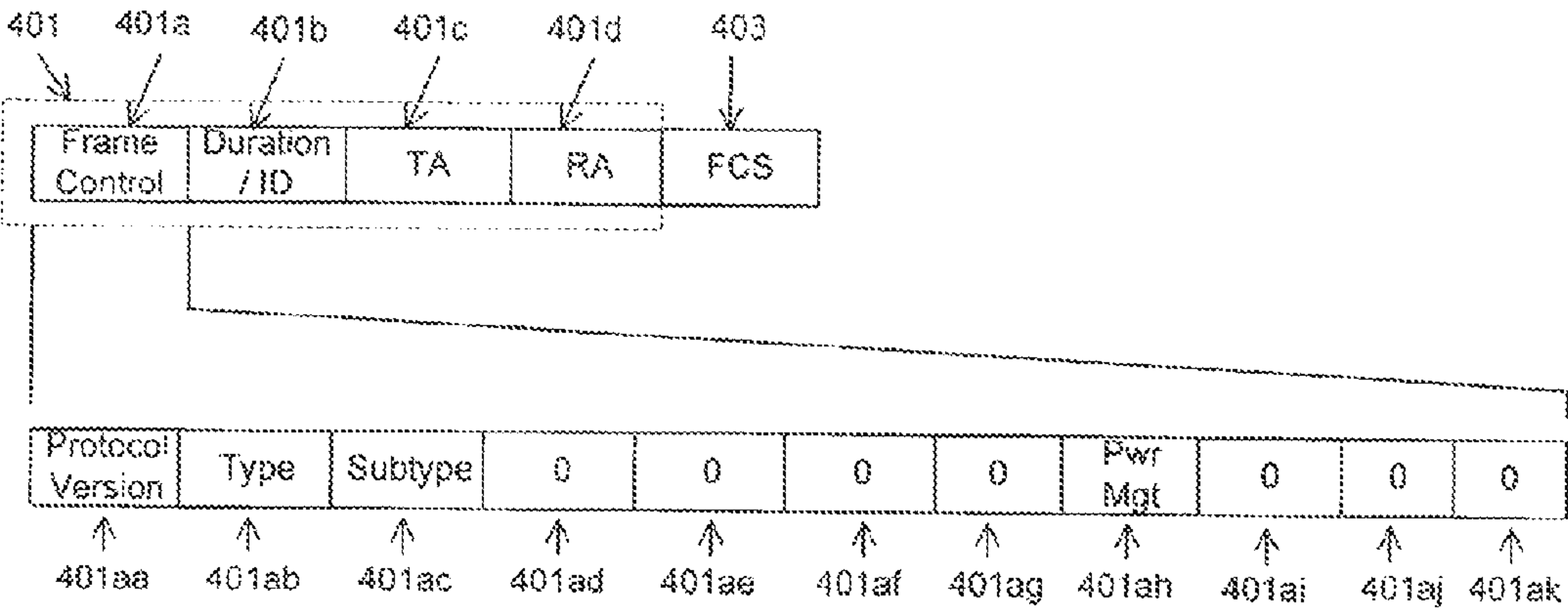
WLAN Request-to-Send (RTS) Control Frame Format Figure 4.0
