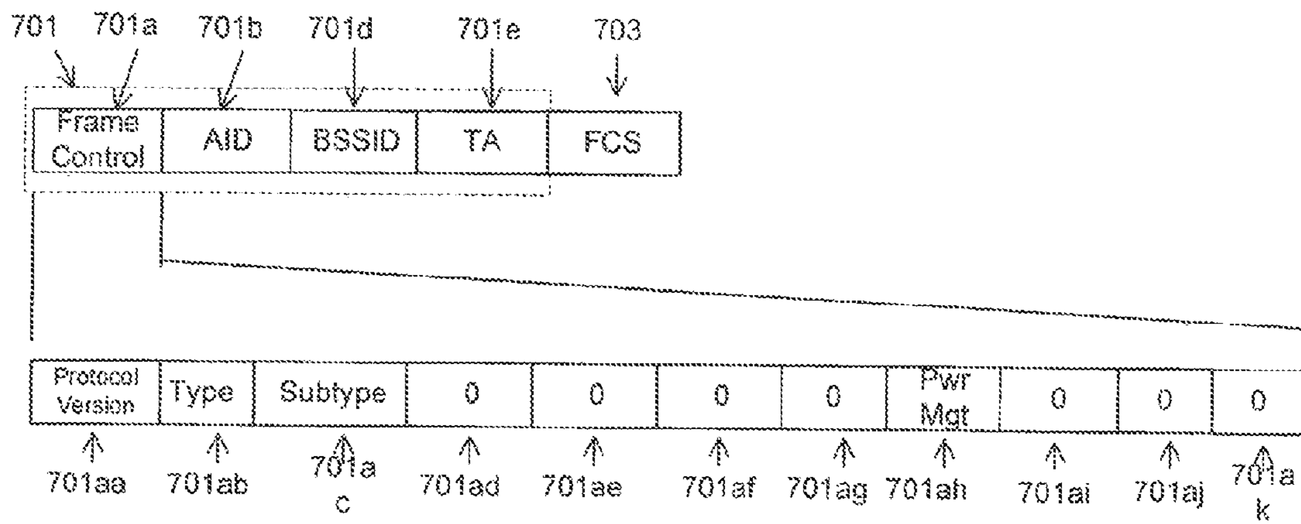
WLAN PS-Poll Control Frame Format Figure 7.0
