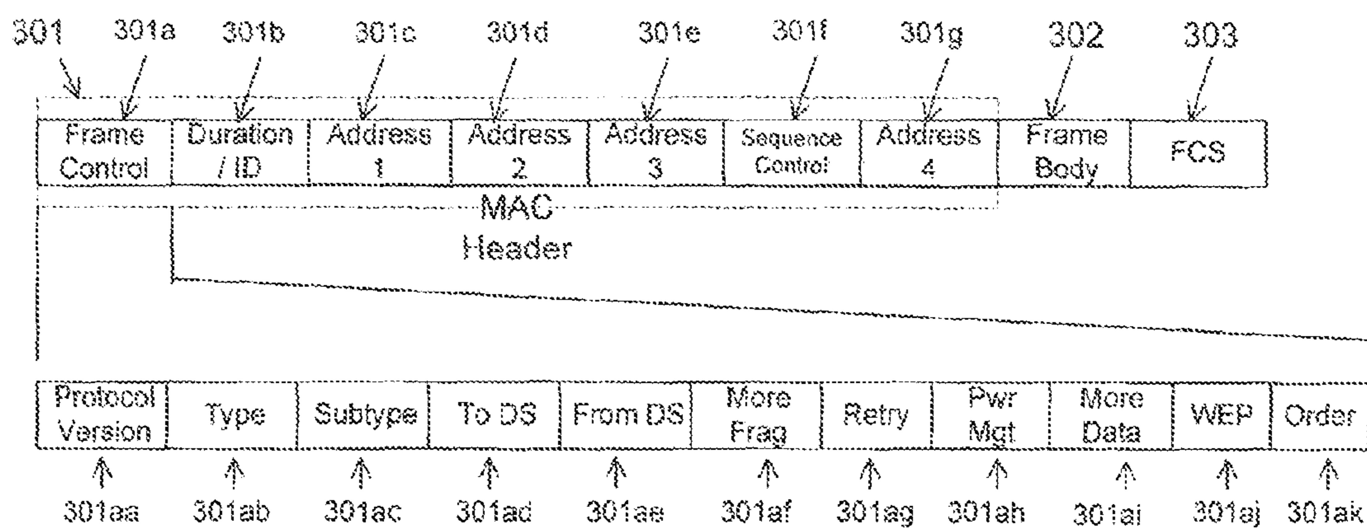
WLAN Generic MAC Frame Format Figure 3.0
