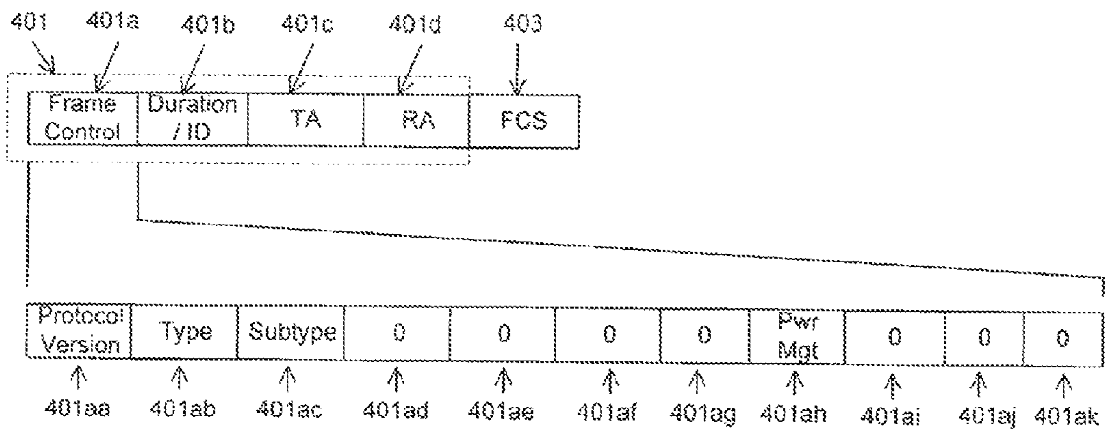
WLAN Request-to-Send (RTS) Control Frame Format Figure 4.0
