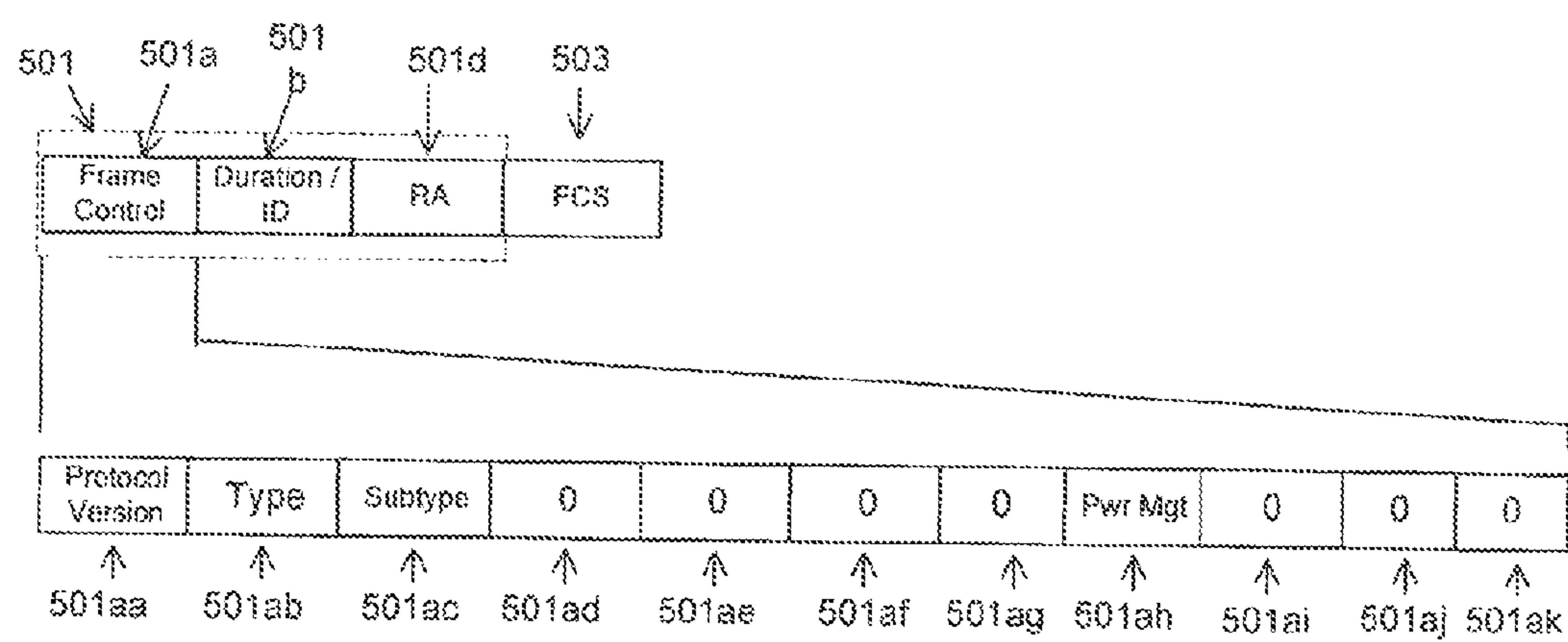
WLAN Clear-to-Send (CTS) Control Frame Format Figure 5.0
