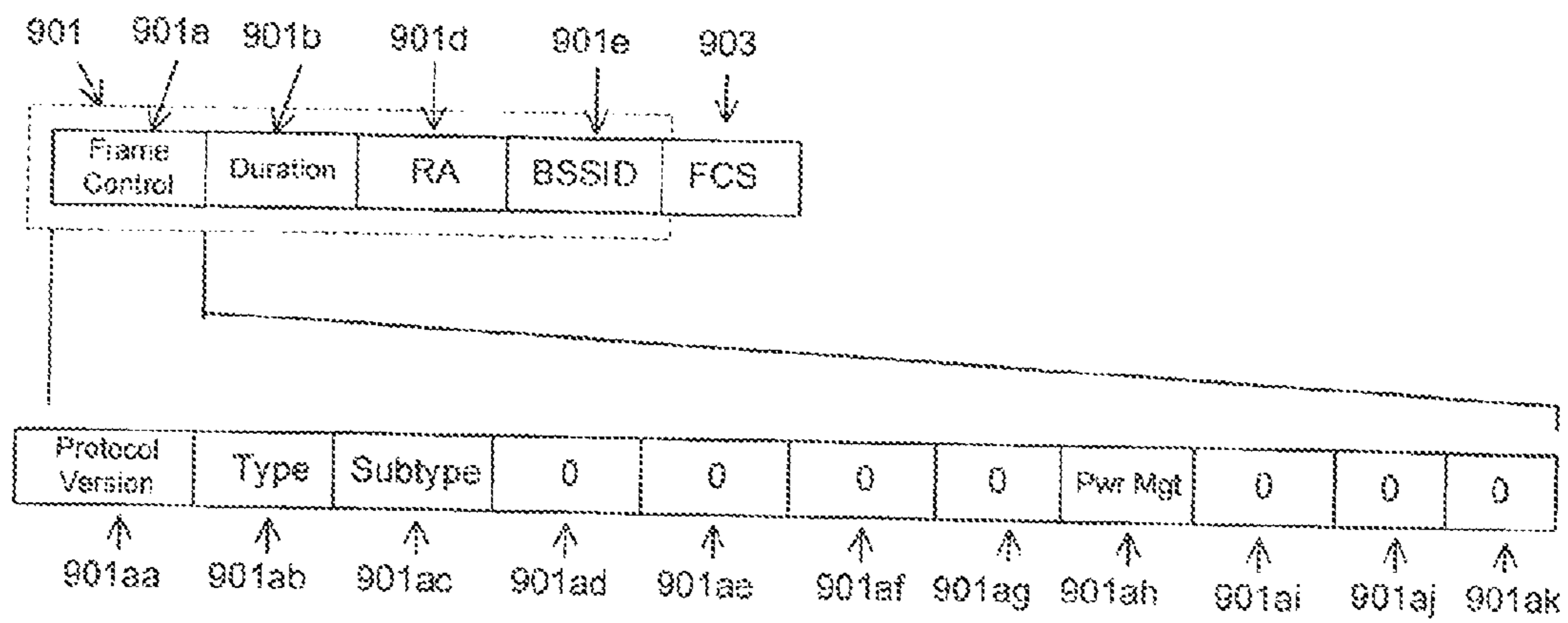
WLAN CF-End+CF-Ack Control Frame Format Figure 9.0
