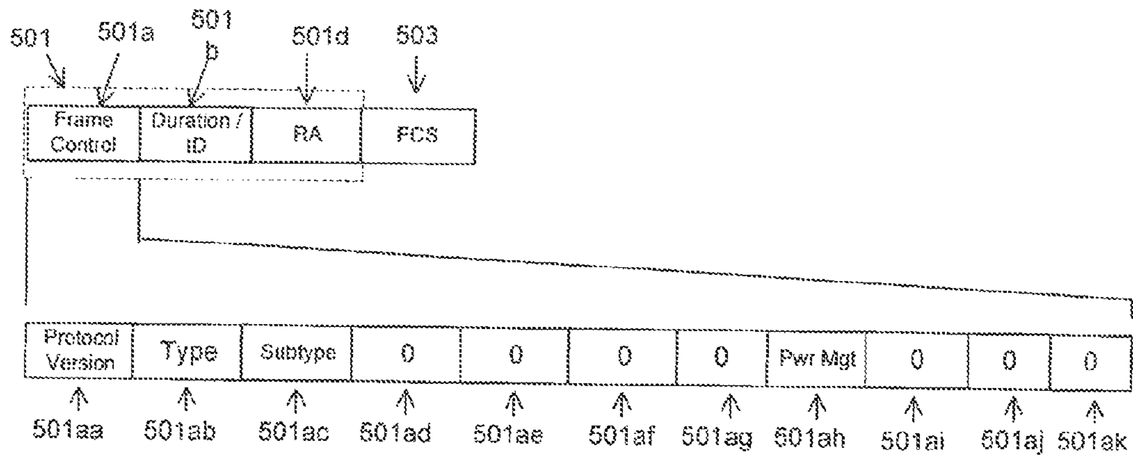
WLAN Clear-to-Send (CTS) Control Frame Format Figure 5.0
