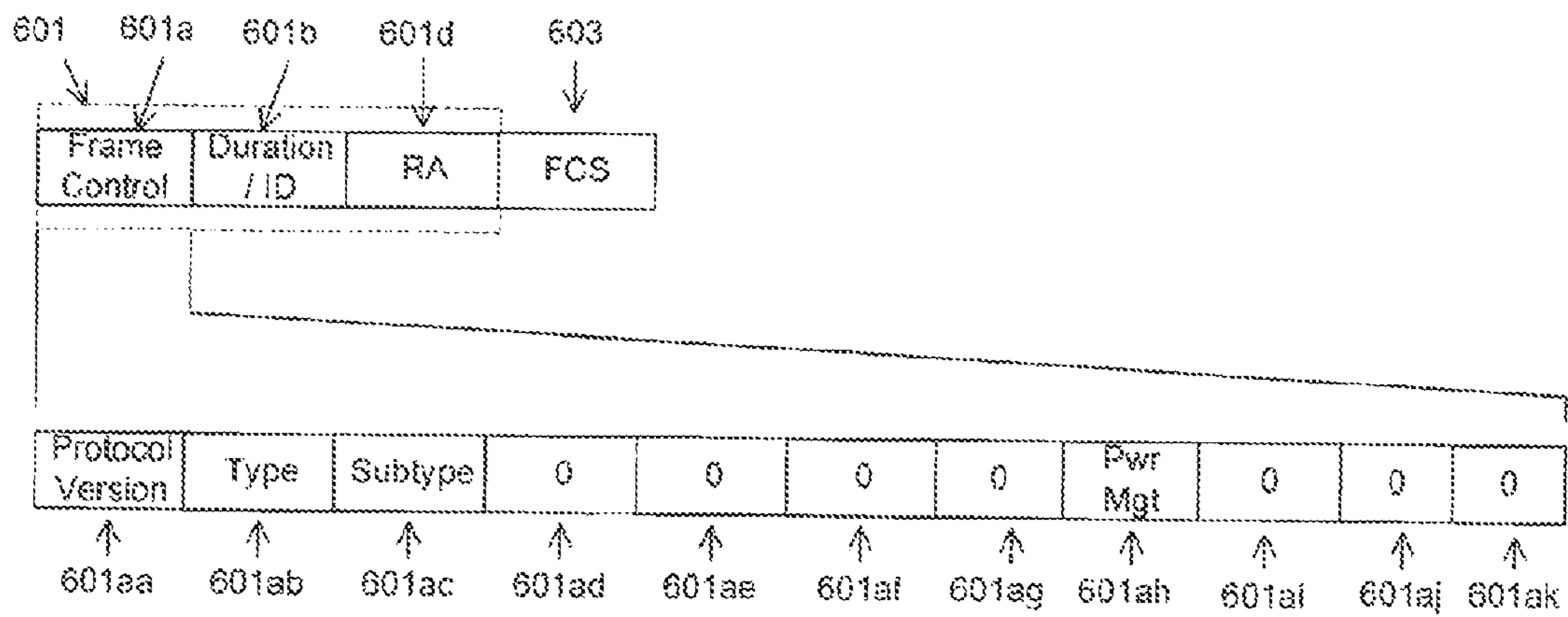
WLAN Acknowledgement (ACK) Control Frame Format
