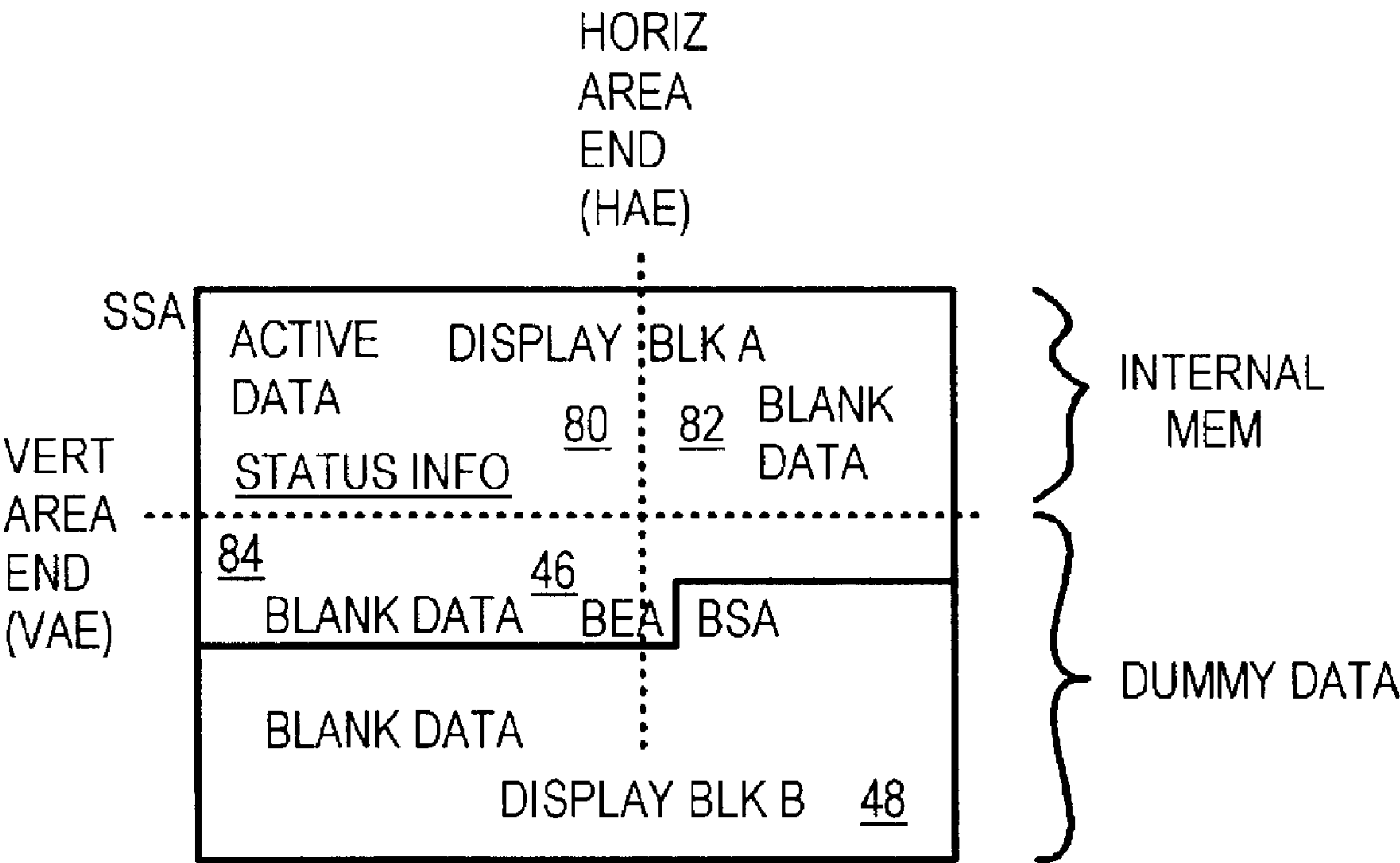
FIG. 8B LOW-POWER MODE
