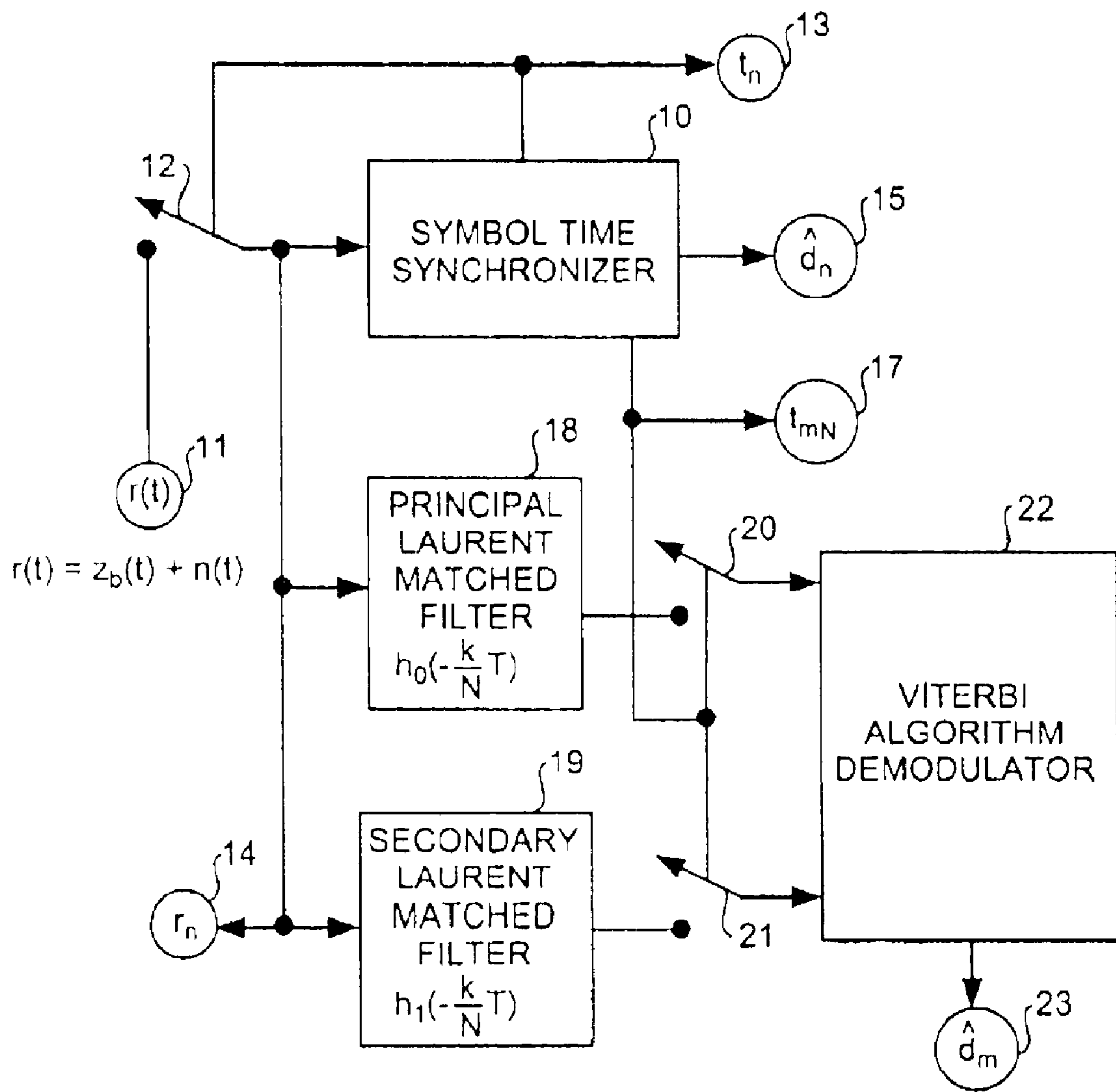
SYMBOL TIME SYNCHRONIZED DATA DEMODULATOR
