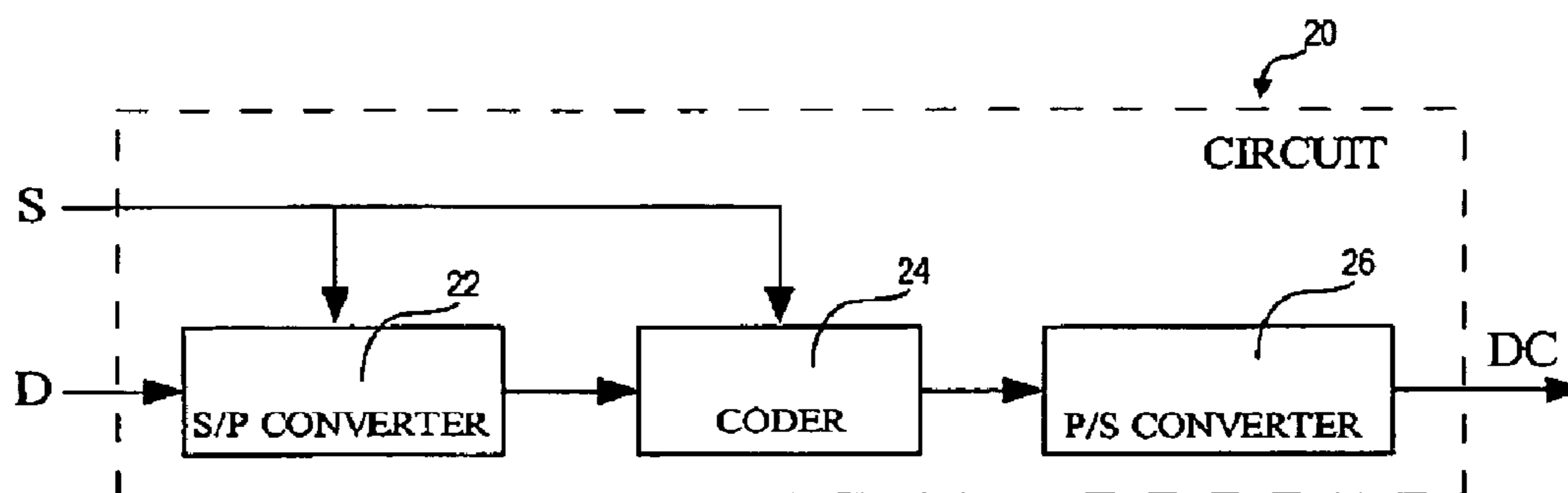
FIG. 2 PRIOR ART
