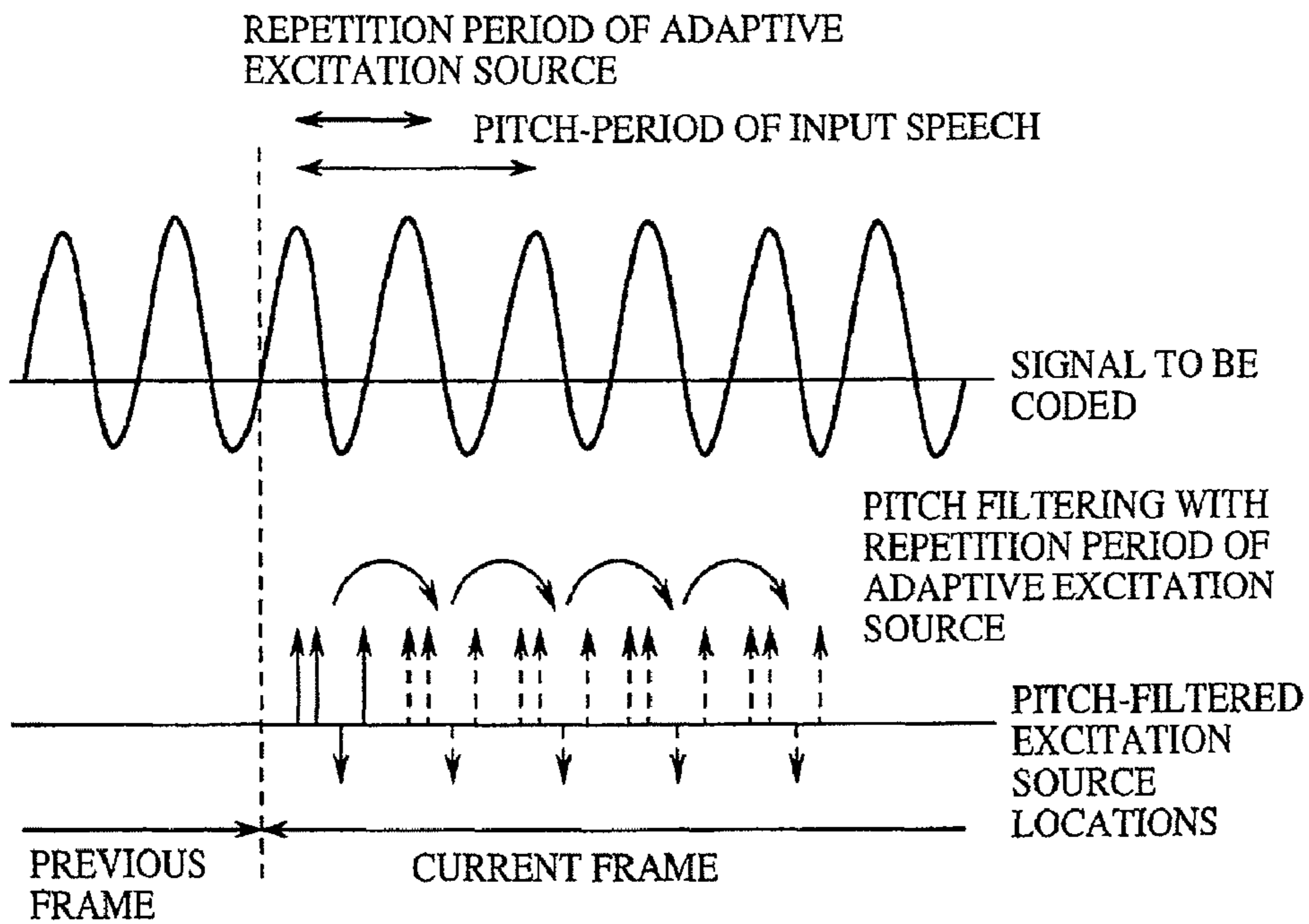
FIG. 19 (PRIOR ART)
