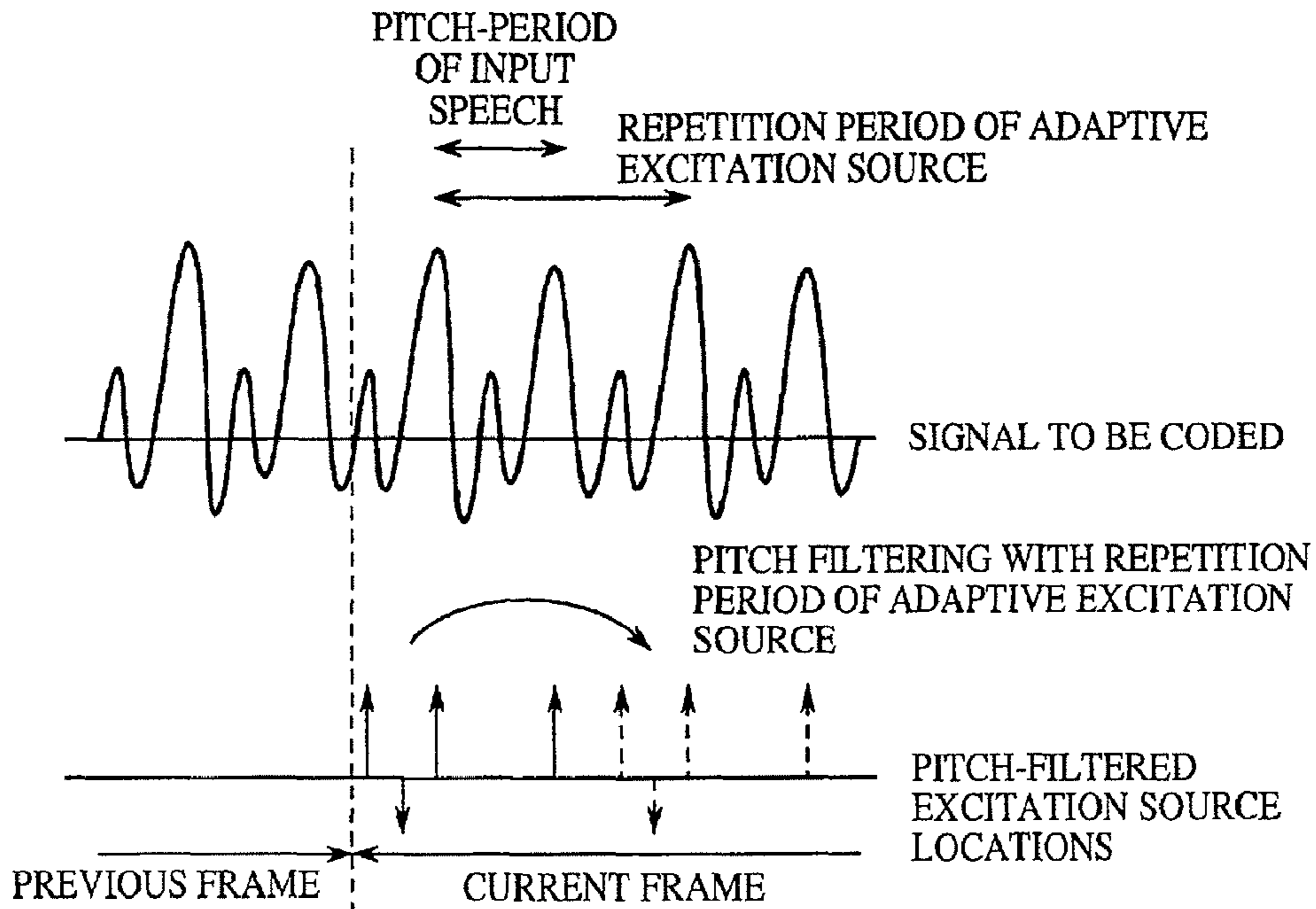
FIG. 18 (PRIOR ART)
