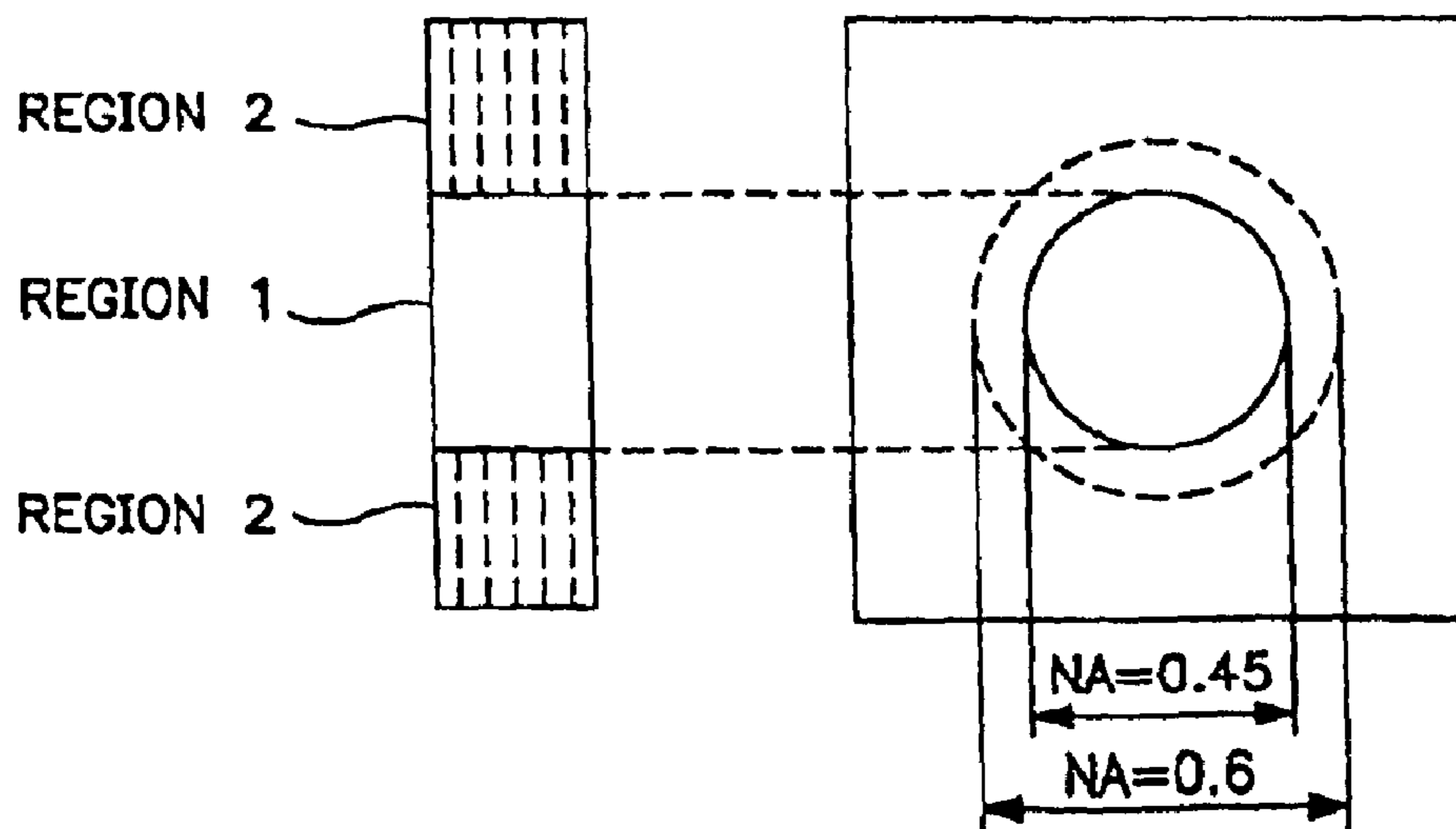
FIG. 2 (PRIOR ART)
