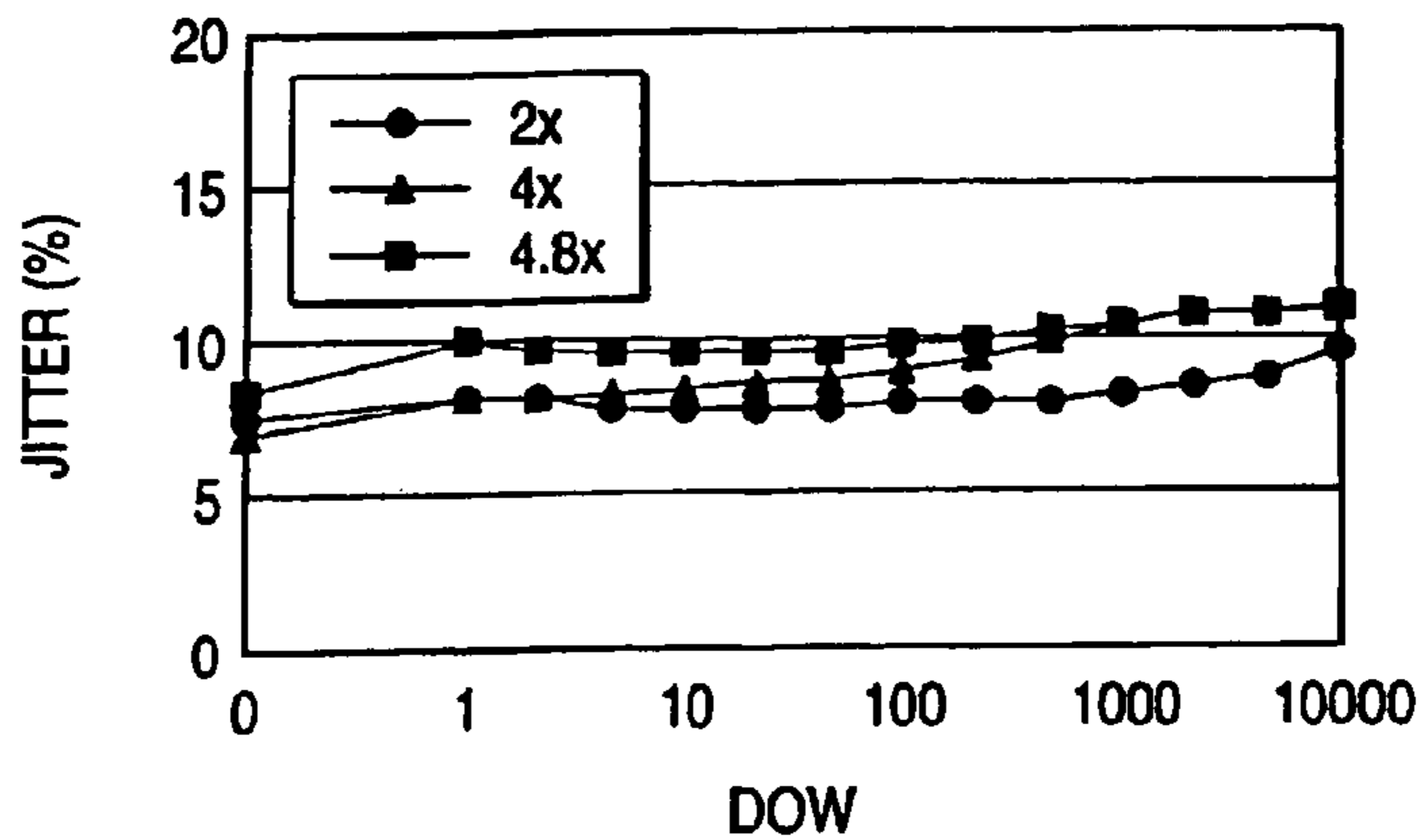
OVERWRITE CYCLE DEPENDENCY OF EDGE-TO-CLOCK JITTER
