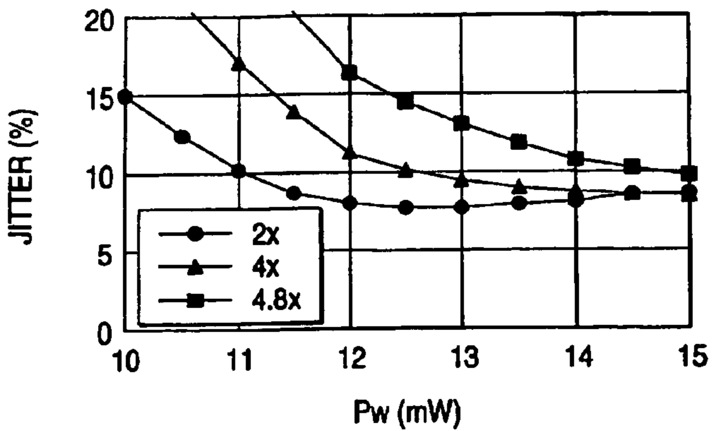
RECORDING POWER DEPENDENCY OF EDGE-TO-CLOCK JITTER
