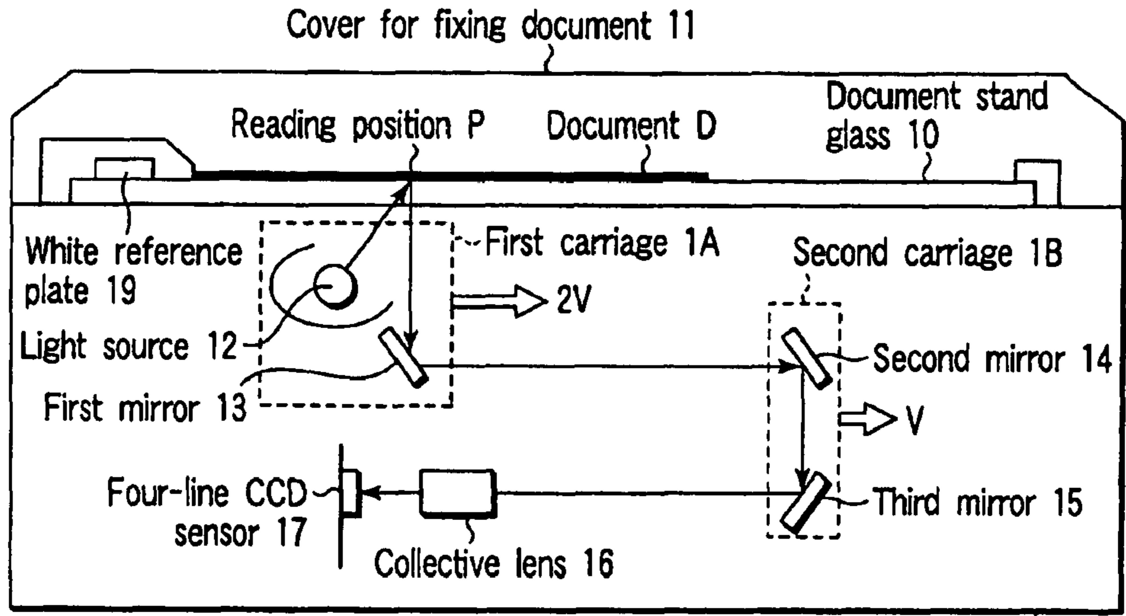
Image inputting apparatus 1
