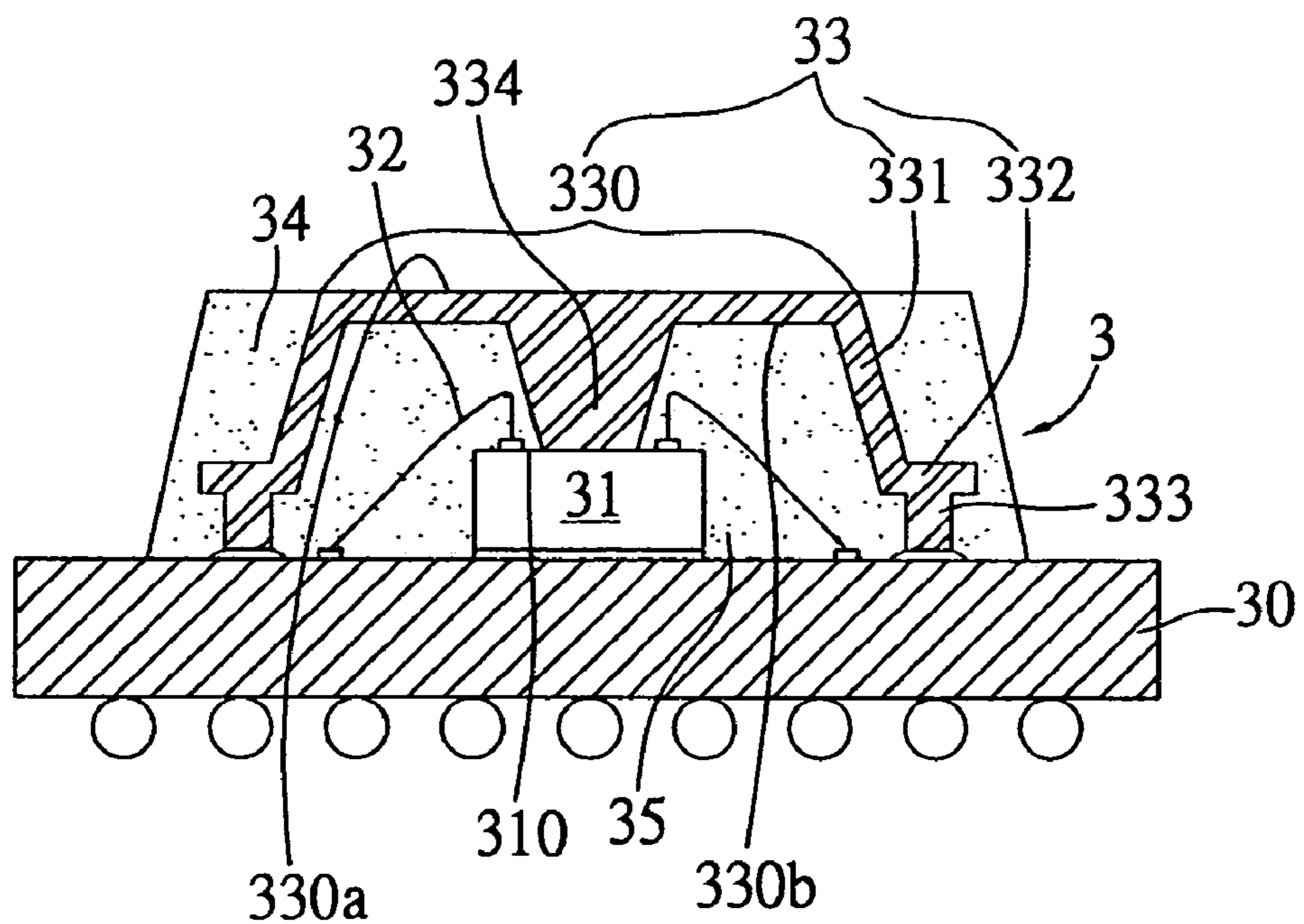
FIG. 5 (PRIOR ART)
