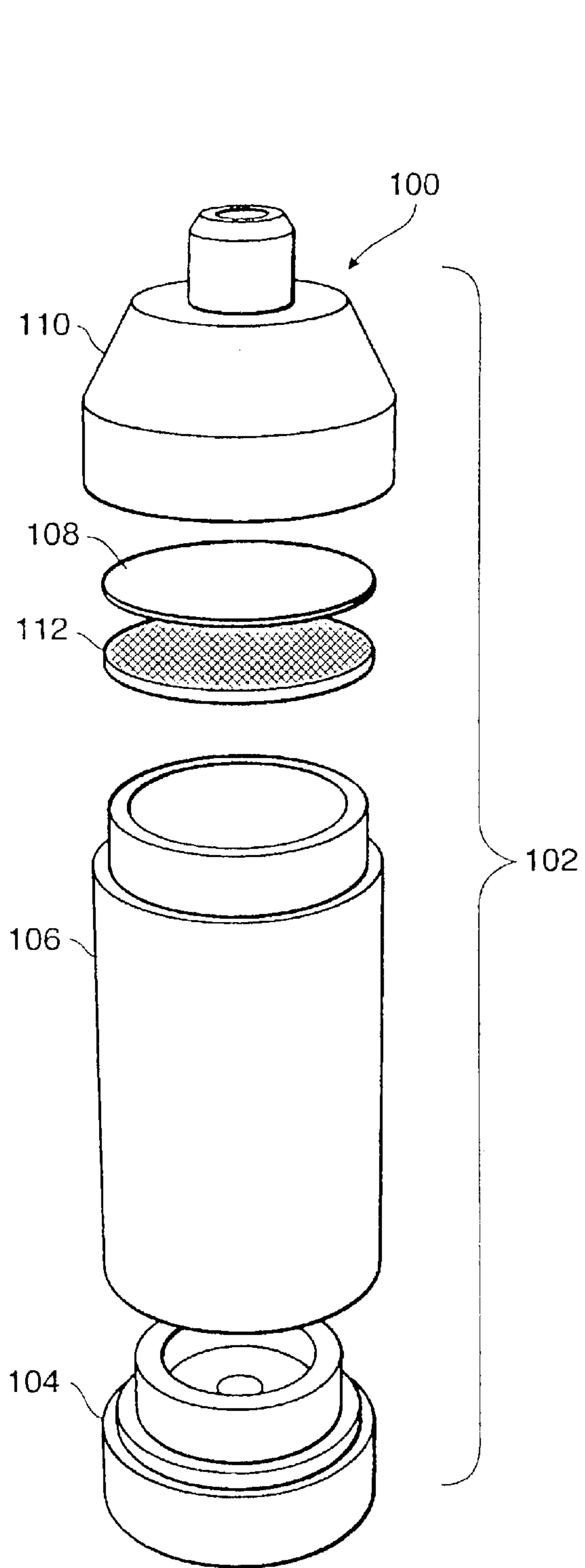
FIG. 1 (Prior Art)
